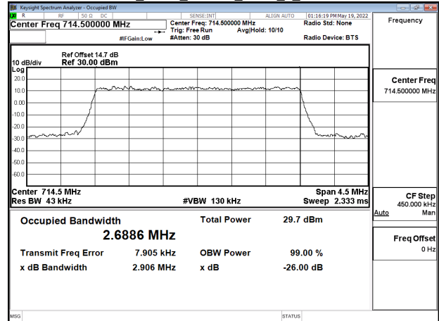
Band12_3MHz_64QAM_RB15_0_CH23165
