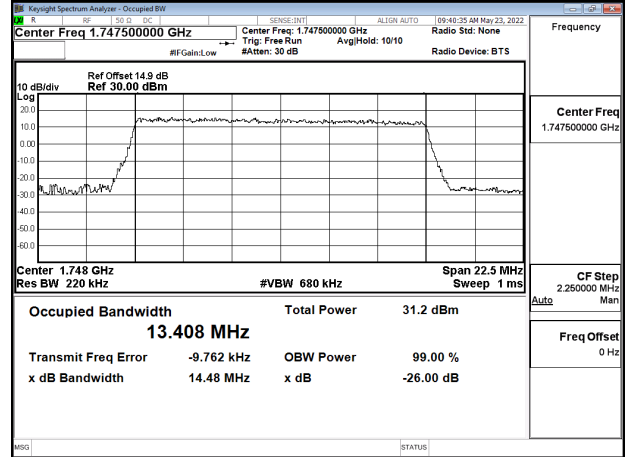
Band4_15MHz_16QAM_RB75_0_CH20325
