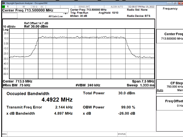
Band17_5MHz_64QAM_RB25_0_CH23825
