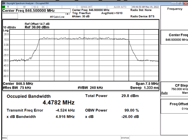
Band5_5MHz_64QAM_RB25_0_CH20625
