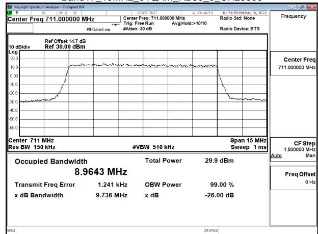
Band17_10MHz_64QAM_RB50_0_CH23800
