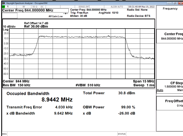
Band5_10MHz_16QAM_RB50_0_CH20600
