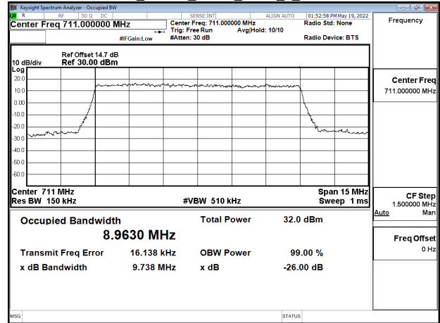
Band17_10MHz_QPSK_RB50_0_CH23800
