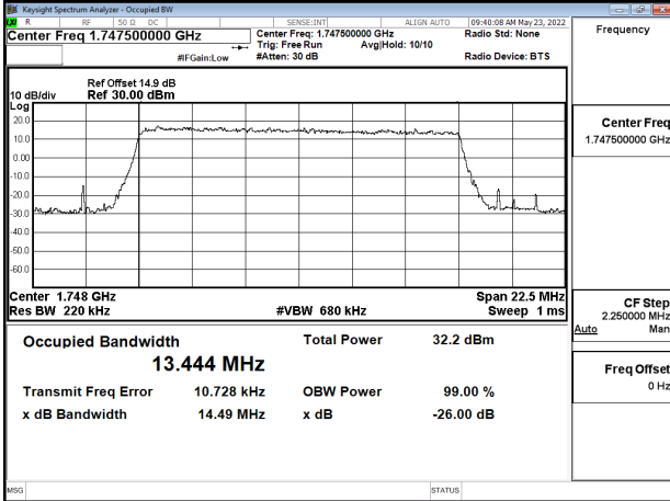
Band4_15MHz_QPSK_RB75_0_CH20325
