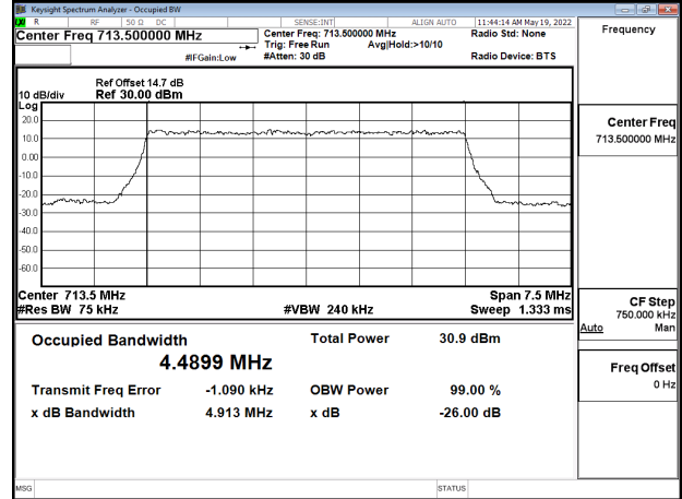
Band12_5MHz_16QAM_RB25_0_CH23155
