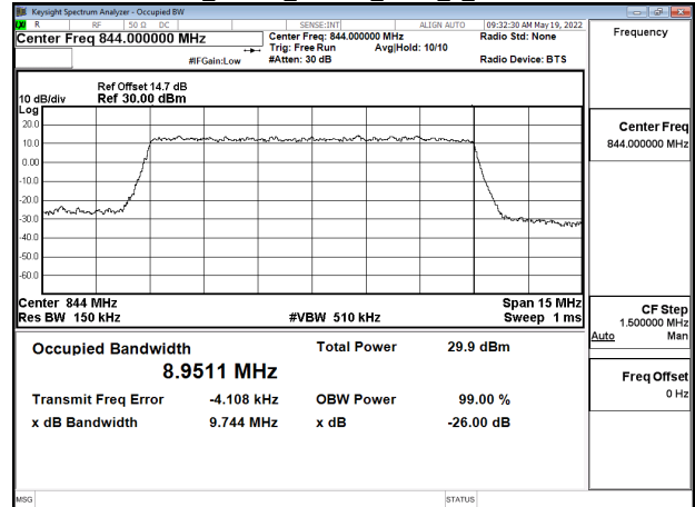
Band5_10MHz_64QAM_RB50_0_CH20600
