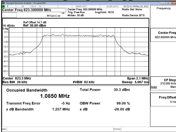
Band26-Part90s_1.4MHz_64QAM_RB6_0_CH26783
