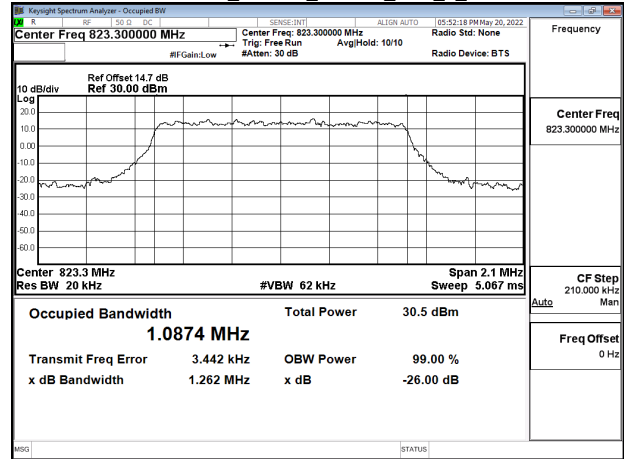
Band26-Part90s_1.4MHz_16QAM_RB6_0_CH26783
