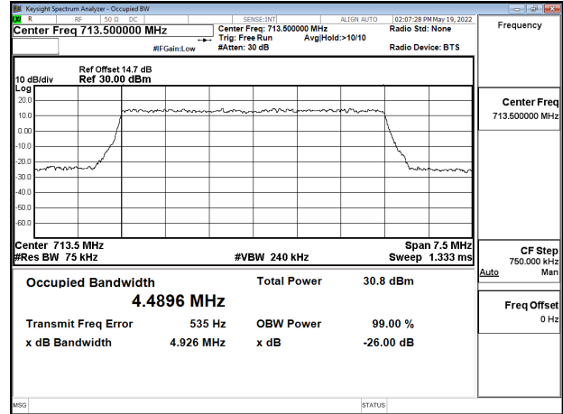
Band17_5MHz_16QAM_RB25_0_CH23825
