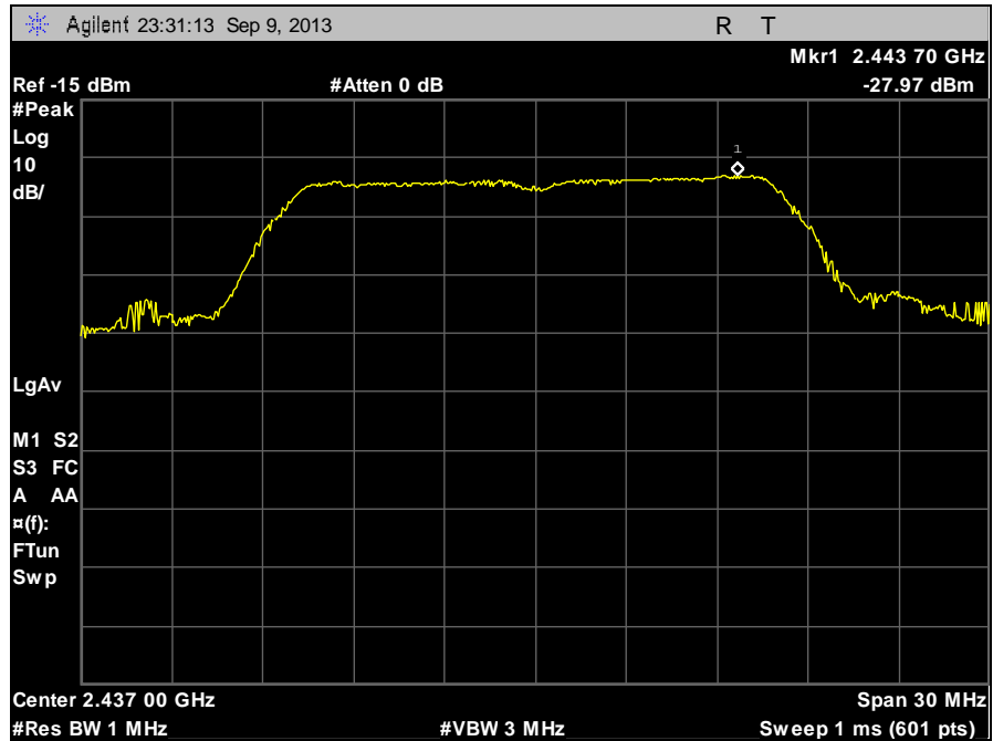
Plot 100. Peak Power Spectral Density, Mid Channel, 802.11g, Peak Search
