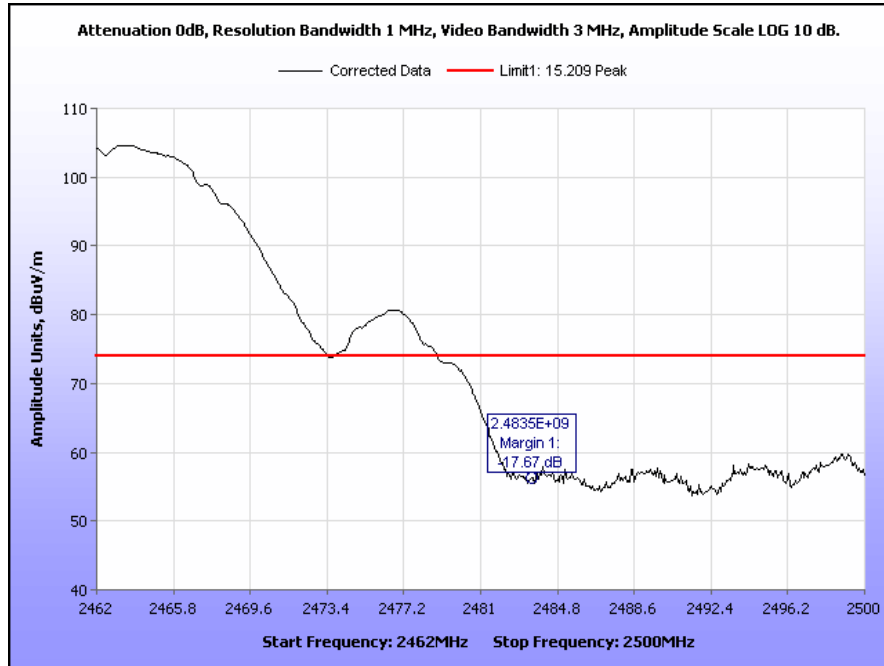
Plot 55. Radiated Band Edge, High Channel, 802.11b, Peak
