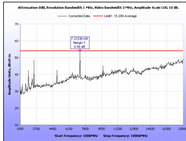
Plot 35. Radiated Spurious Emissions, Low Channel, 802.11b, 1 GHz – 18 GHz, Peak under Average
