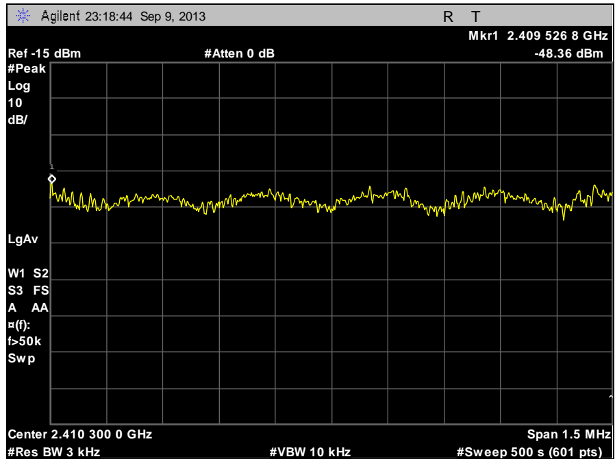
Plot 105. Peak Power Spectral Density, Low Channel, 802.11n
