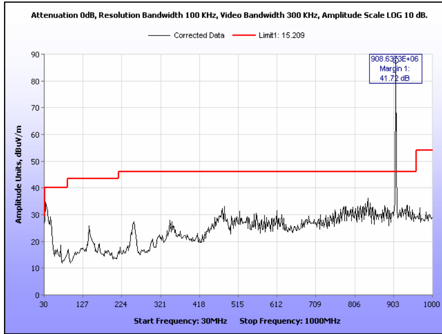
Plot 67. Radiated Spurious Emissions, Mid Channel, 802.11b, 30 MHz – 1 GHz, 900 MHz TX
