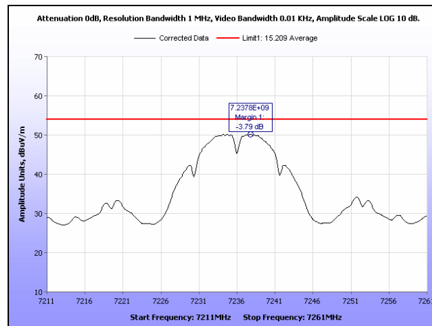
Plot 36. Radiated Spurious Emissions, Low Channel, 802.11b, 1 GHz – 18 GHz, 7237 MHz, Average
