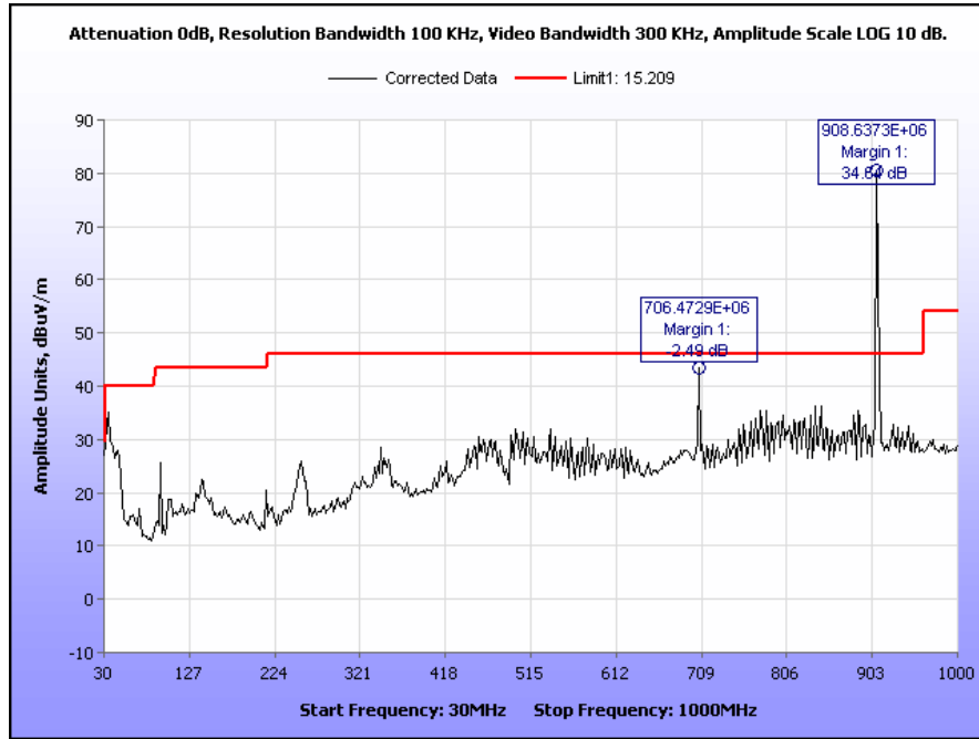
Plot 73. Radiated Spurious Emissions, Mid Channel, 802.11g, 30 MHz – 1 GHz, 900 MHz TX
