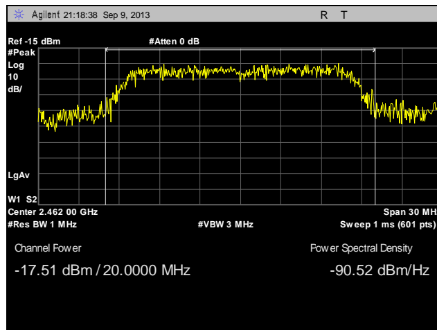
Plot 33. Peak Power Output, High Channel, 802.11n
