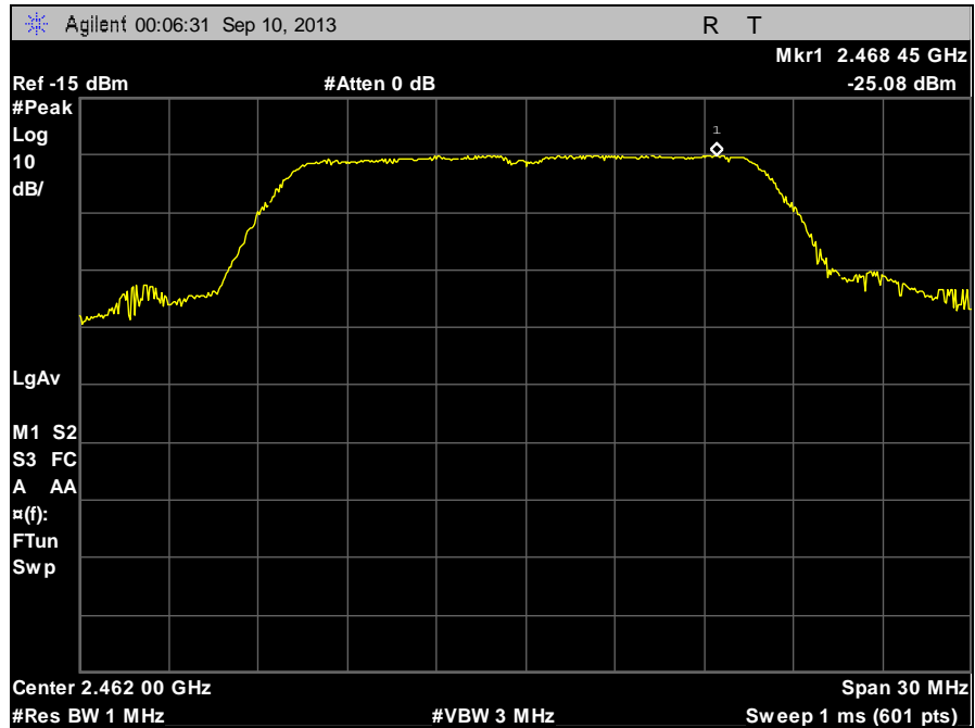
Plot 102. Peak Power Spectral Density, High Channel, 802.11g, Peak Search
