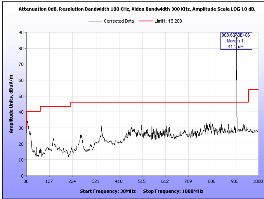
Plot 69. Radiated Spurious Emissions, High Channel, 802.11b, 30 MHz – 1 GHz, 900 MHz TX
