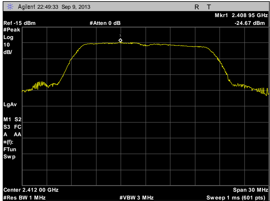
Plot 98. Peak Power Spectral Density, Low Channel, 802.11g, Peak Search
