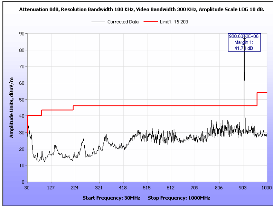
Plot 71. Radiated Spurious Emissions, Low Channel, 802.11g, 30 MHz – 1 GHz, 900 MHz TX
