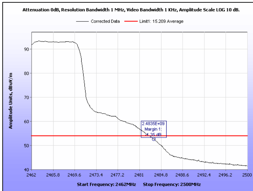
Plot 60. Radiated Band Edge, High Channel, 802.11g, Average
