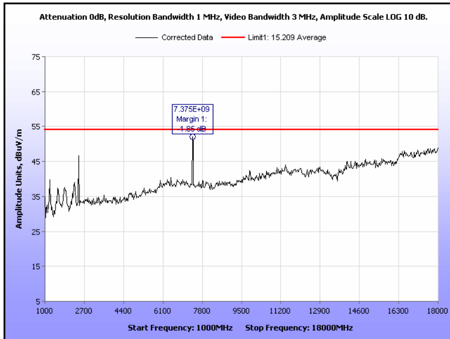
Plot 52. Radiated Spurious Emissions, High Channel, 802.11n, 1 GHz – 18 GHz, Peak under Average
