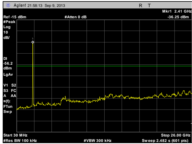
Plot 89. Conducted Spurious Emissions, Low Channel, 802.11n, 30 MHz – 26 GHz
