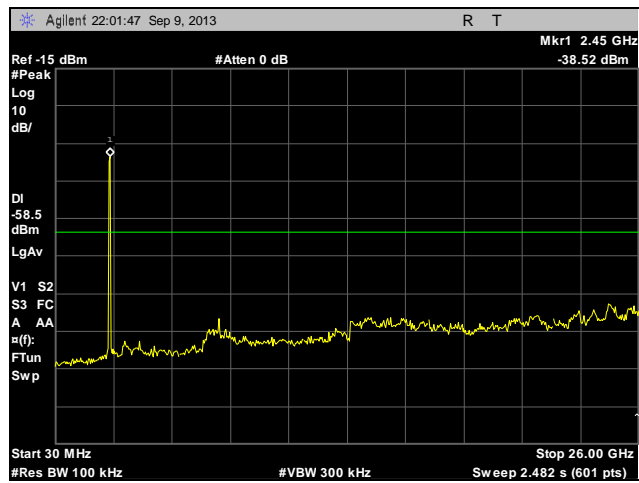
Plot 90. Conducted Spurious Emissions, Mid Channel, 802.11n, 30 MHz – 26 GHz
