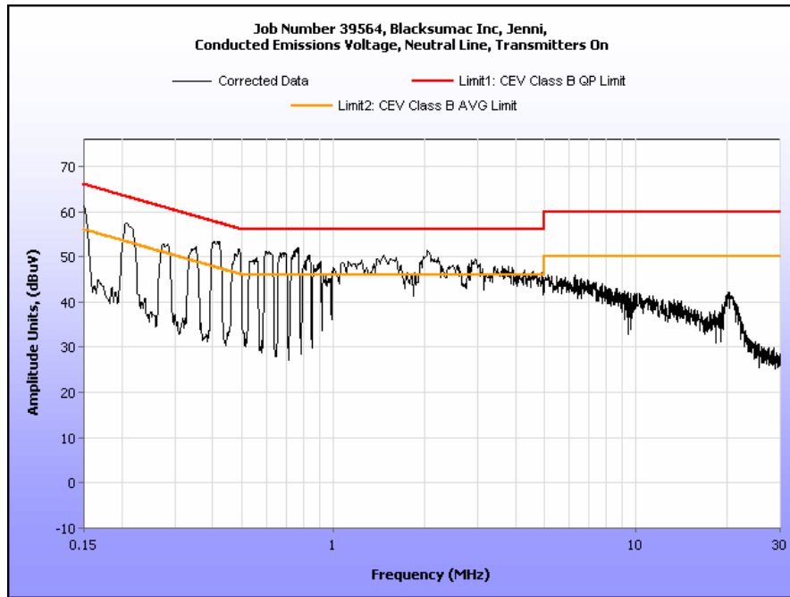
Plot 6. Conducted Emissions, 15.207, Neutral Line
