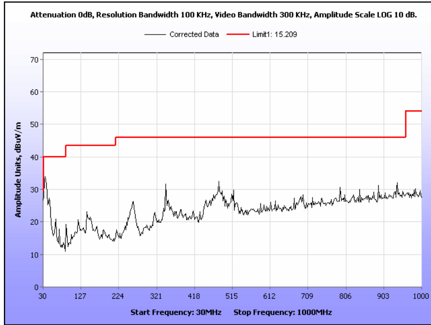
Plot 51. Radiated Spurious Emissions, High Channel, 802.11n, 30 MHz – 1 GHz
