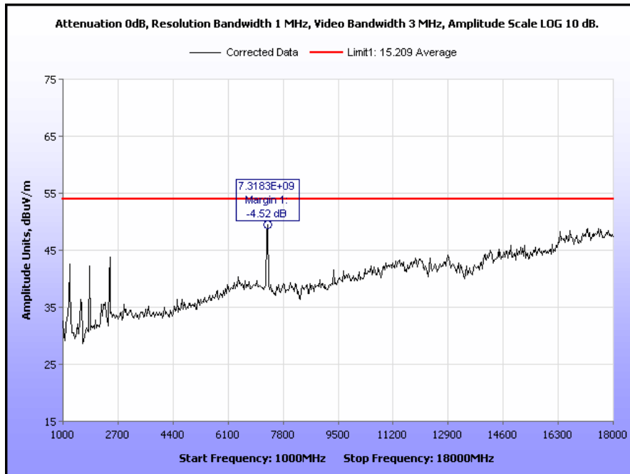
Plot 80. Radiated Spurious Emissions, Mid Channel, 802.11n, 1 GHz – 18 GHz, 900 MHz TX
