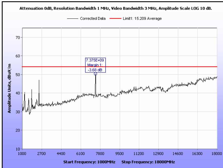
Plot 70. Radiated Spurious Emissions, High Channel, 802.11b, 1 GHz – 18 GHz, 900 MHz TX
