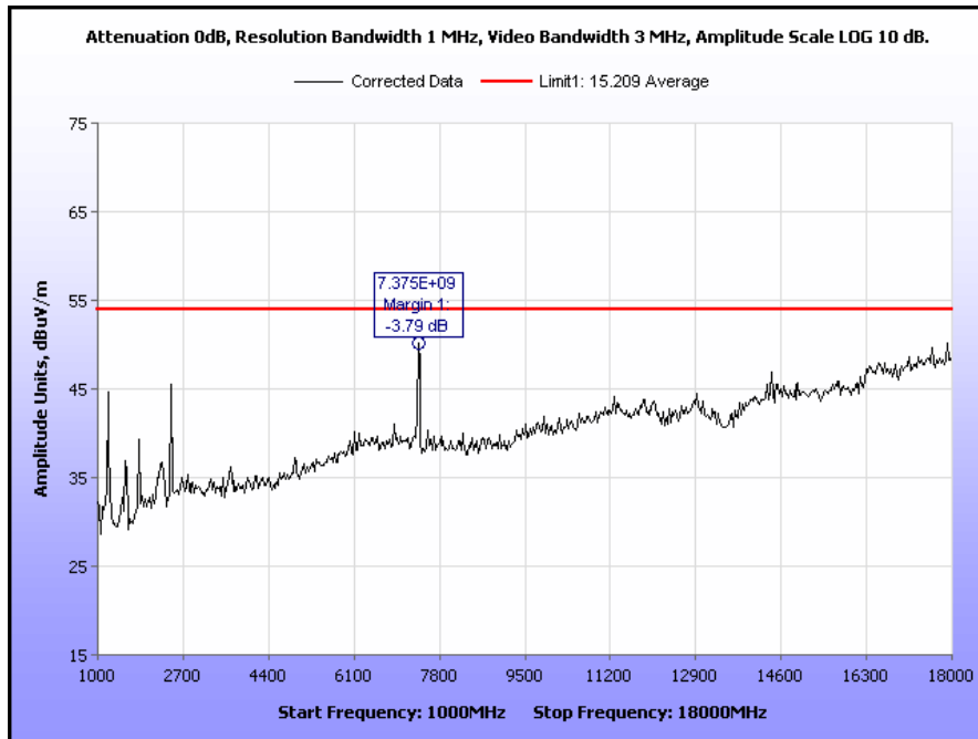
Plot 76. Radiated Spurious Emissions, High Channel, 802.11g, 1 GHz – 18 GHz, 900 MHz TX
