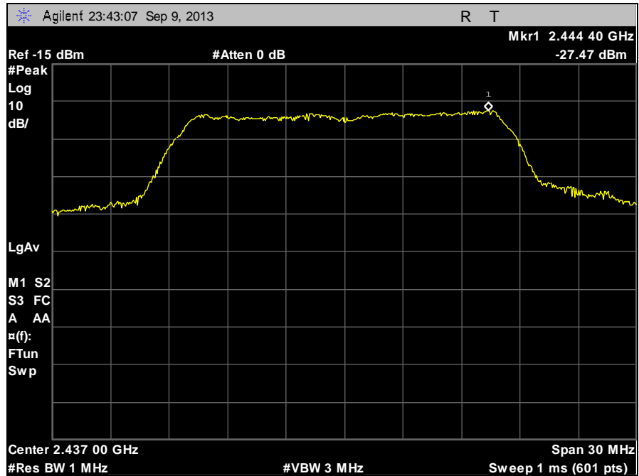
Plot 106. Peak Power Spectral Density, Mid Channel, 802.11n, Peak Search
