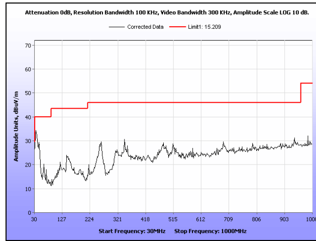
Plot 34. Radiated Spurious Emissions, Low Channel, 802.11b, 30 MHz – 1 GHz
