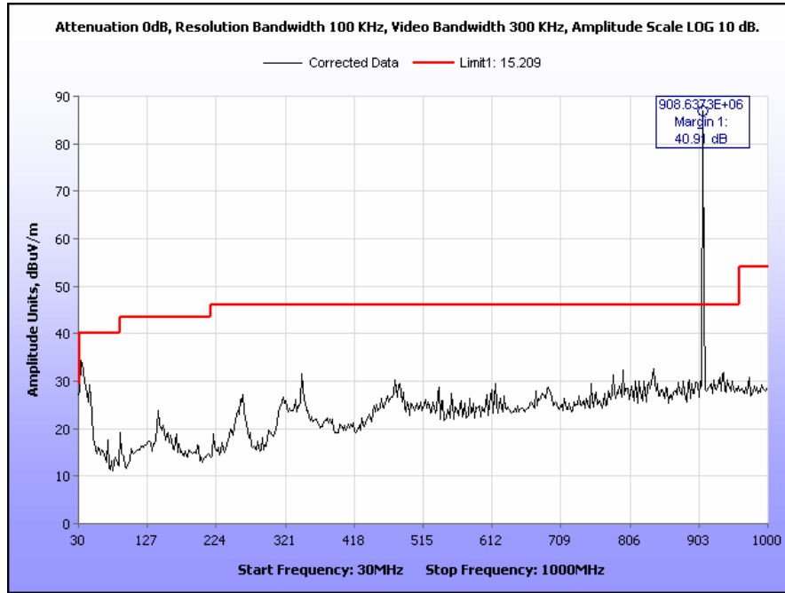
Plot 81. Radiated Spurious Emissions, High Channel, 802.11n, 30 MHz – 1 GHz, 900 MHz TX
