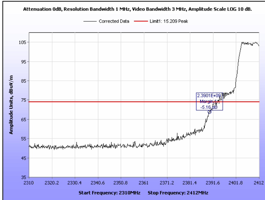
Plot 61. Radiated Band Edge, Low Channel, 802.11n, Peak
