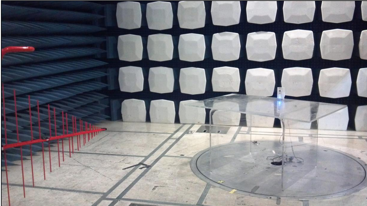
Photograph 5. Radiated Spurious Emissions, Test Setup, 30 MHz – 1 GHz
