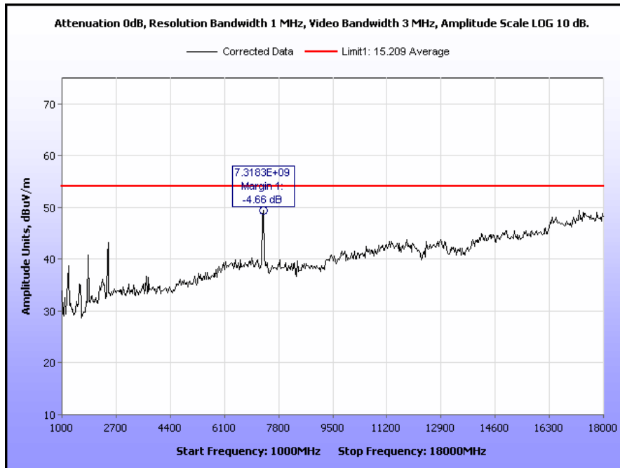
Plot 68. Radiated Spurious Emissions, Mid Channel, 802.11b, 1 GHz – 18 GHz, 900 MHz TX
