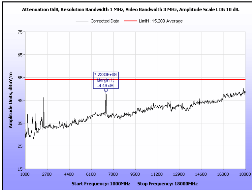
Plot 78. Radiated Spurious Emissions, Low Channel, 802.11n, 1 GHz – 18 GHz, 900 MHz TX
