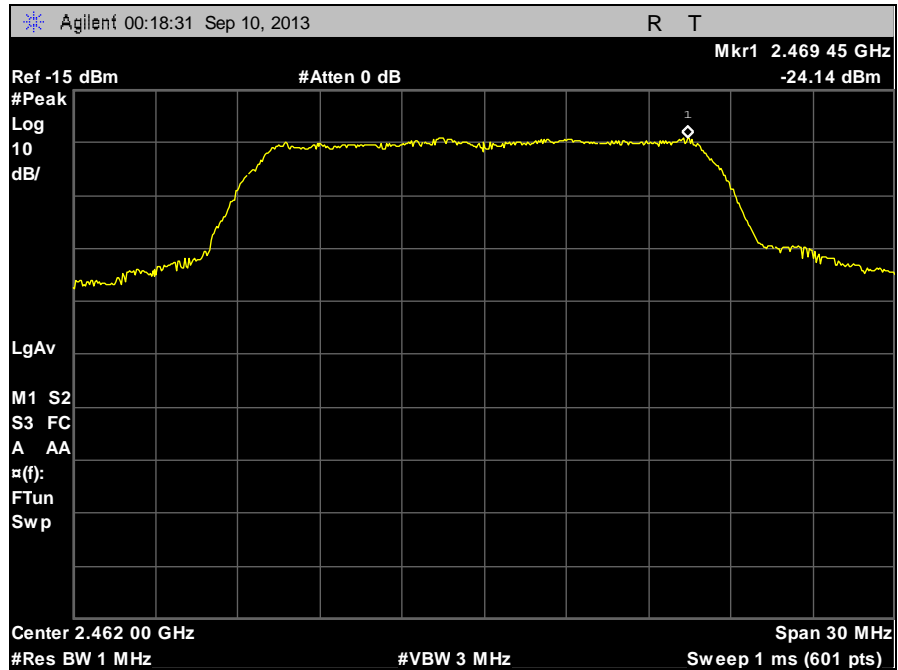
Plot 108. Peak Power Spectral Density, High Channel, 802.11n, Peak Search
