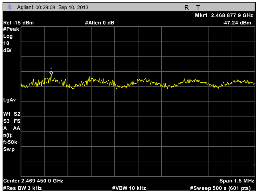
Plot 109. Peak Power Spectral Density, High Channel, 802.11n
