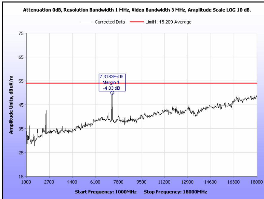
Plot 74. Radiated Spurious Emissions, Mid Channel, 802.11g, 1 GHz – 18 GHz, 900 MHz TX
