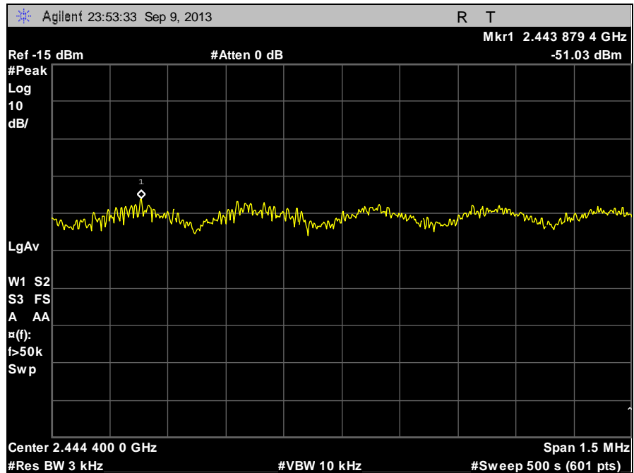
Plot 107. Peak Power Spectral Density, Mid Channel, 802.11n
