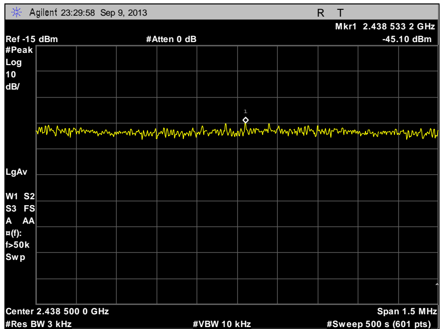
Plot 95. Peak Power Spectral Density, Mid Channel, 802.11b
