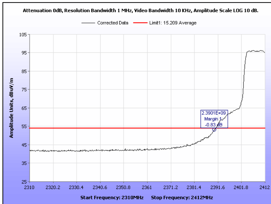
Plot 62. Radiated Band Edge, Low Channel, 802.11n, Average
