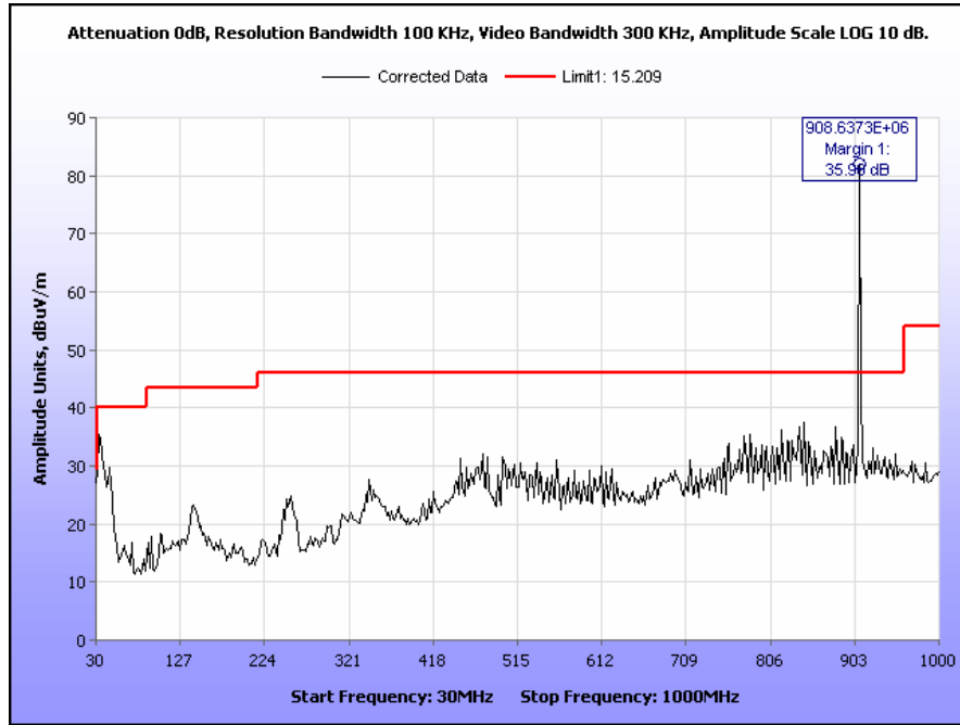
Plot 77. Radiated Spurious Emissions, Low Channel, 802.11n, 30 MHz – 1 GHz, 900 MHz TX
