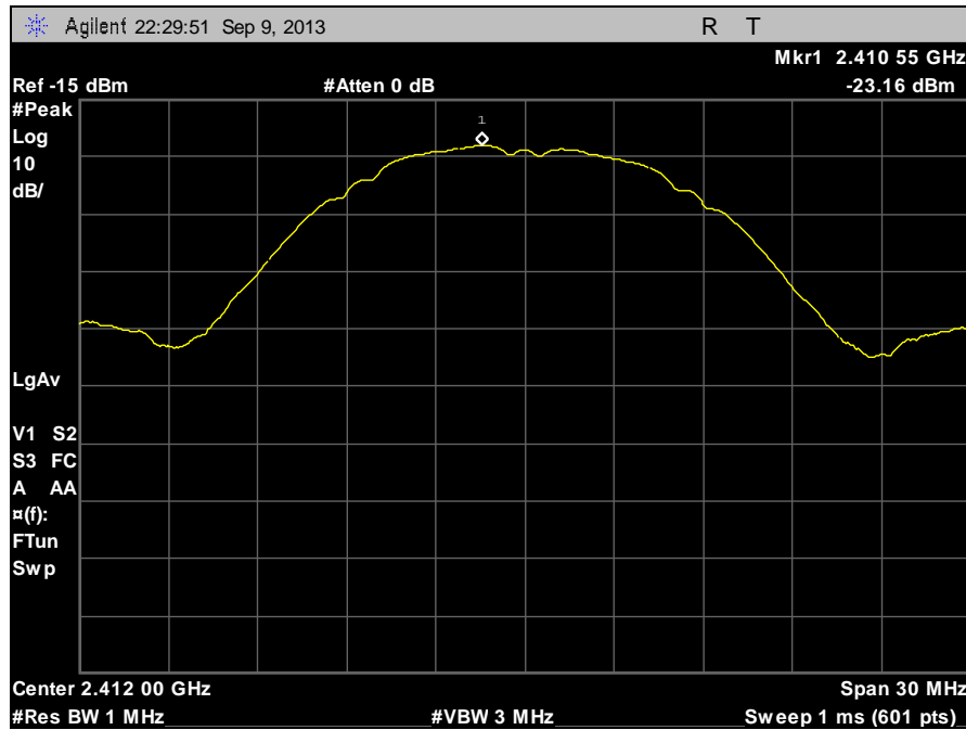
Plot 92. Peak Power Spectral Density, Low Channel, 802.11b, Peak Search
