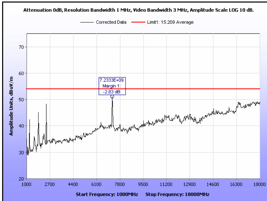
Plot 48. Radiated Spurious Emissions, Low Channel, 802.11n, 1 GHz – 18 GHz, Peak under Average
