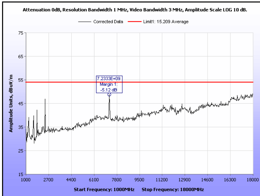
Plot 72. Radiated Spurious Emissions, Low Channel, 802.11g, 1 GHz – 18 GHz, 900 MHz TX
