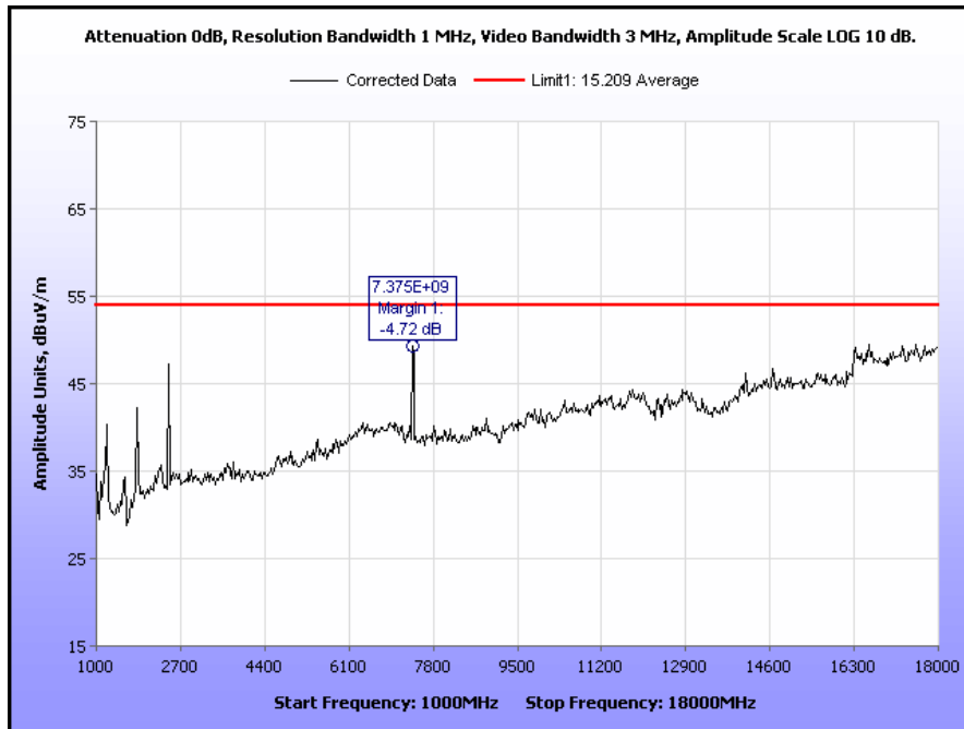
Plot 82. Radiated Spurious Emissions, High Channel, 802.11n, 1 GHz – 18 GHz, 900 MHz TX
