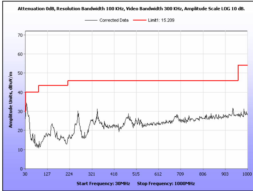
Plot 39. Radiated Spurious Emissions, High Channel, 802.11b, 30 MHz – 1 GHz
