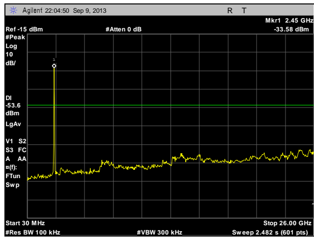
Plot 91. Conducted Spurious Emissions, High Channel, 802.11n, 30 MHz – 26 GHz
