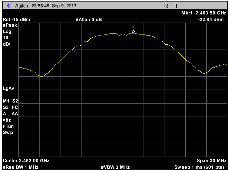
Plot 96. Peak Power Spectral Density, High Channel, 802.11b, Peak Search
