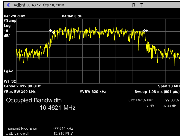
Plot 22. 99% Occupied Bandwidth, Low Channel, 802.11n
