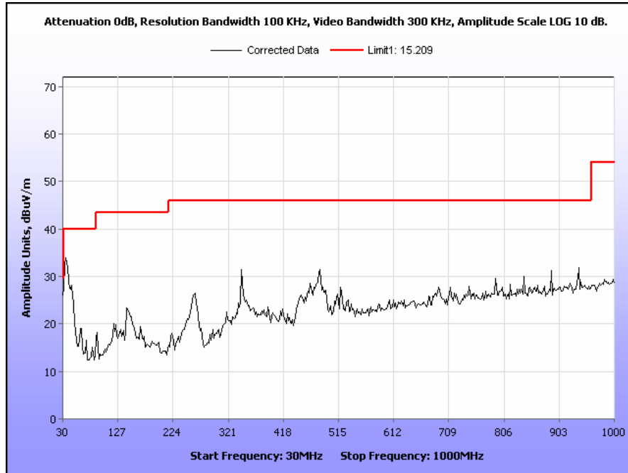
Plot 49. Radiated Spurious Emissions, Mid Channel, 802.11n, 30 MHz – 1 GHz
