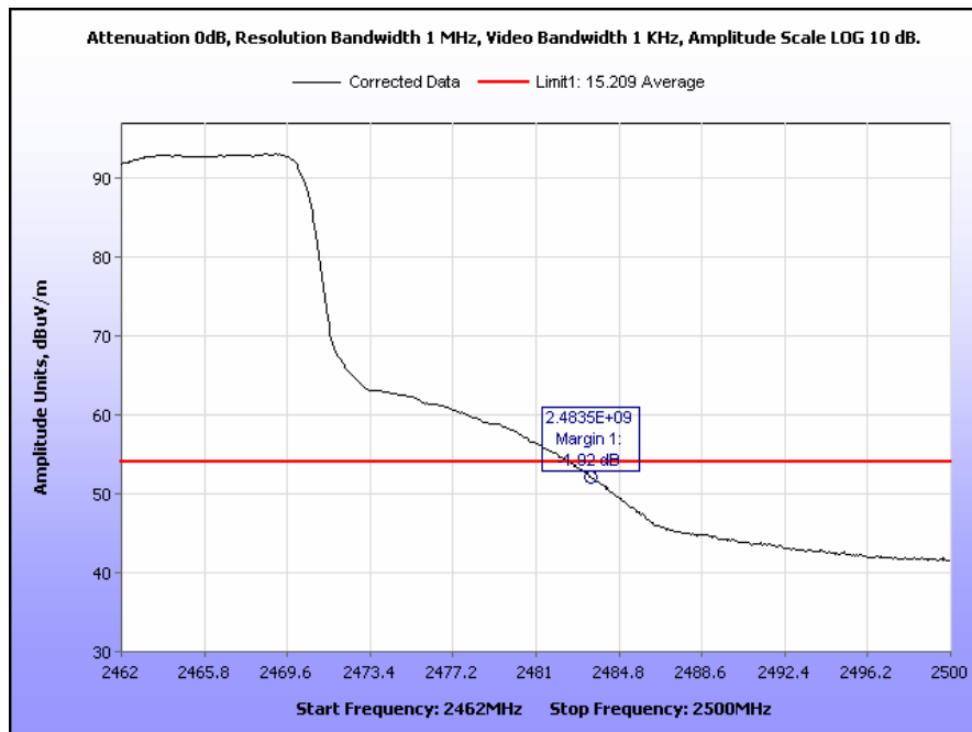
Plot 64. Radiated Band Edge, High Channel, 802.11n, Average
