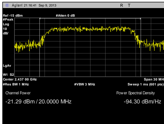
Plot 32. Peak Power Output, Mid Channel, 802.11n
