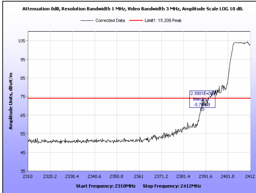
Plot 57. Radiated Band Edge, Low Channel, 802.11g, Peak
