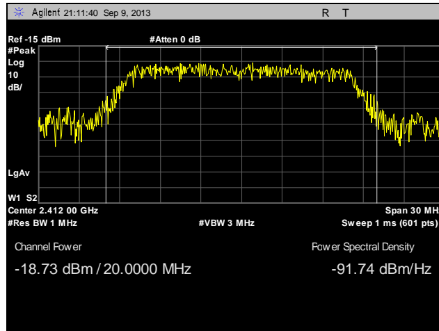
Plot 31. Peak Power Output, Low Channel, 802.11n
