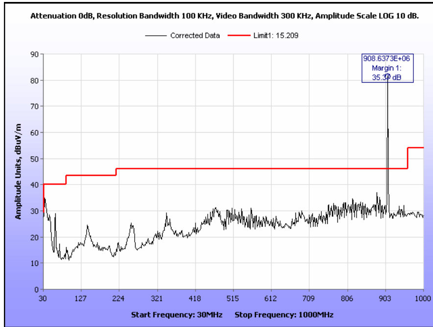
Plot 65. Radiated Spurious Emissions, Low Channel, 802.11b, 30 MHz – 1 GHz, 900 MHz TX
