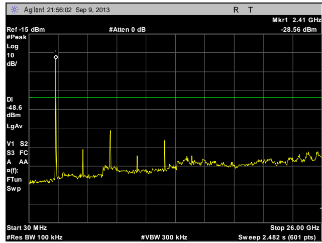
Plot 83. Conducted Spurious Emissions, Low Channel, 802.11b, 30 MHz – 26 GHz
