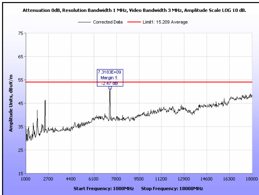
Plot 44. Radiated Spurious Emissions, Mid Channel, 802.11g, 1 GHz – 18 GHz, Peak under Average
