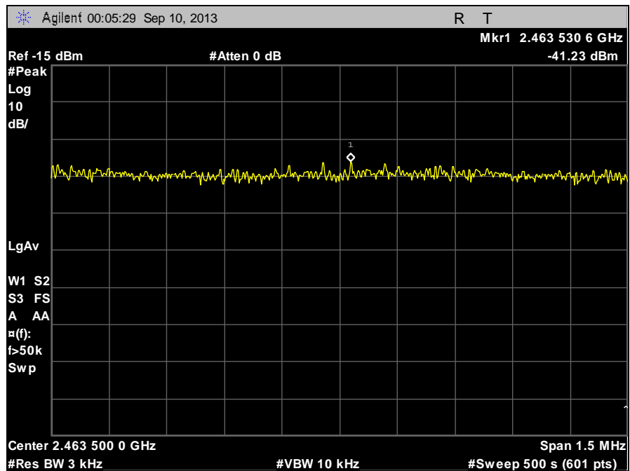
Plot 97. Peak Power Spectral Density, High Channel, 802.11b
