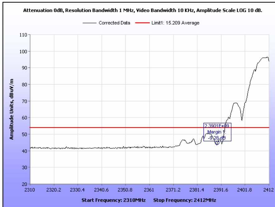
Plot 54. Radiated Band Edge, Low Channel, 802.11b, Average
