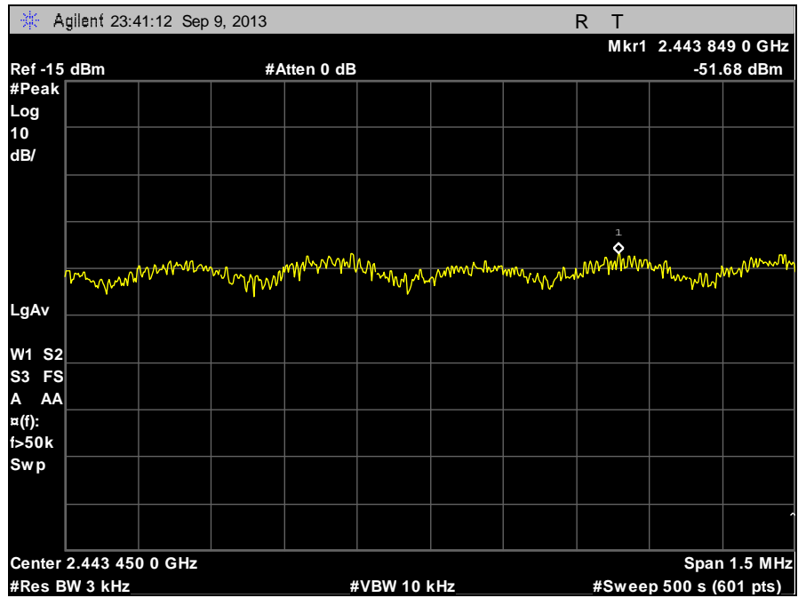
Plot 101. Peak Power Spectral Density, Mid Channel, 802.11g
