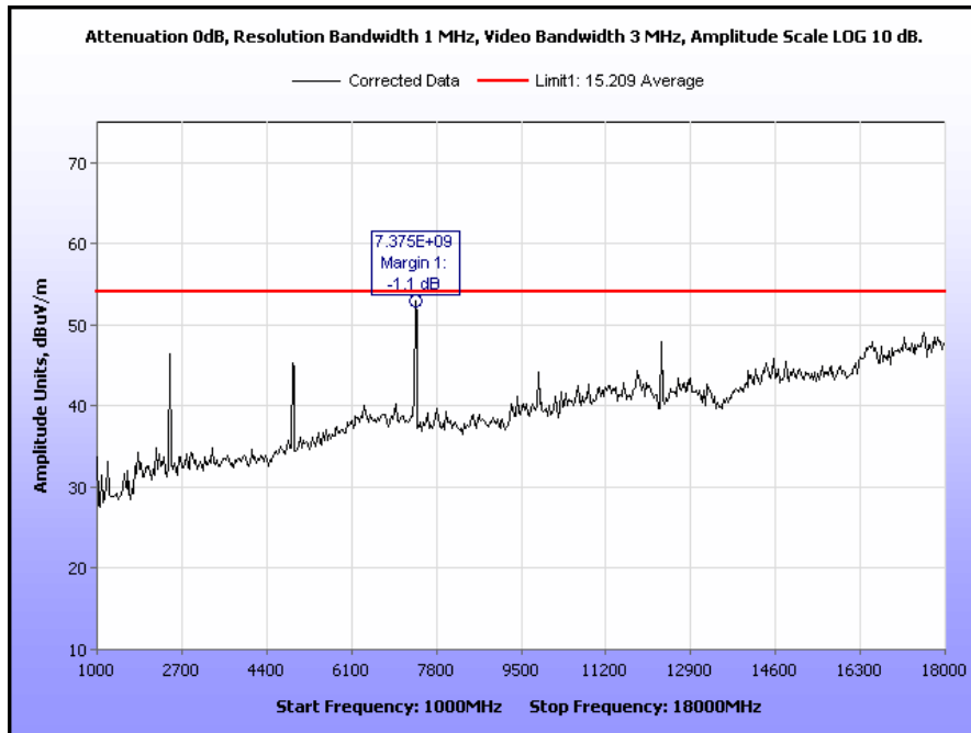
Plot 40. Radiated Spurious Emissions, High Channel, 802.11b, 1 GHz – 18 GHz, Peak under Average
