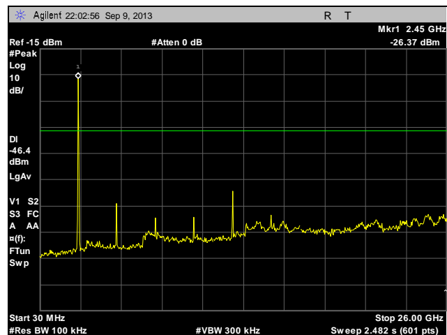
Plot 85. Conducted Spurious Emissions, High Channel, 802.11b, 30 MHz – 26 GHz
