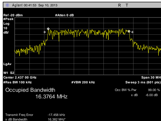
Plot 14. 6 dB Occupied Bandwidth, Mid Channel, 802.11n
