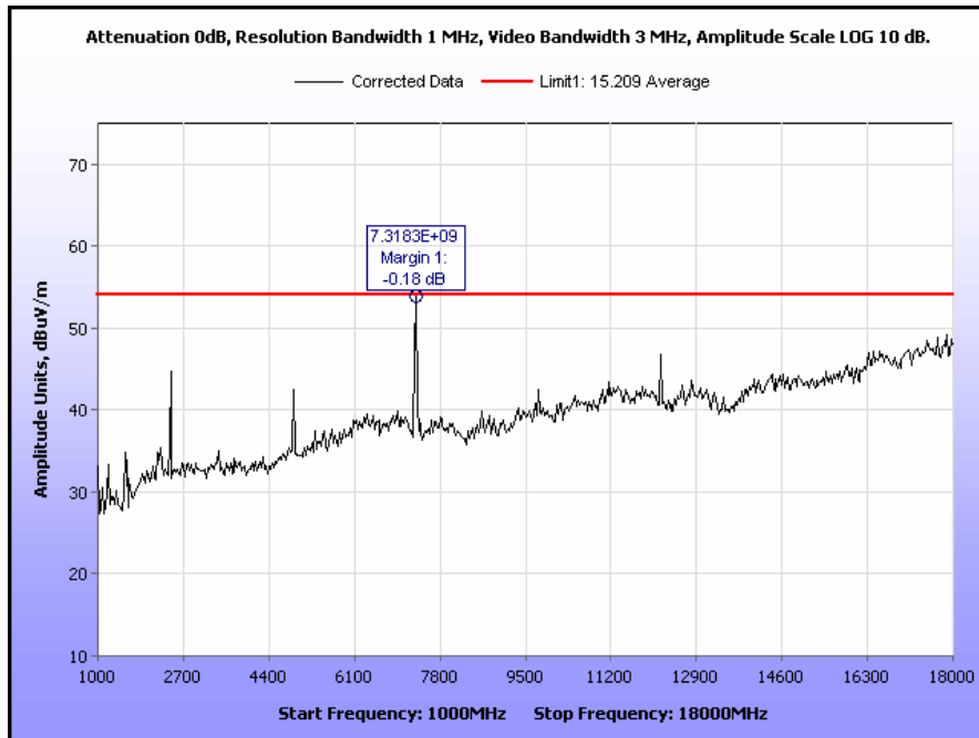
Plot 38. Radiated Spurious Emissions, Mid Channel, 802.11b, 1 GHz – 18 GHz, Peak under Average
