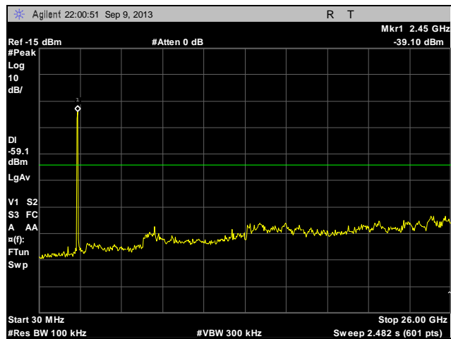
Plot 87. Conducted Spurious Emissions, Mid Channel, 802.11g, 30 MHz – 26 GHz
