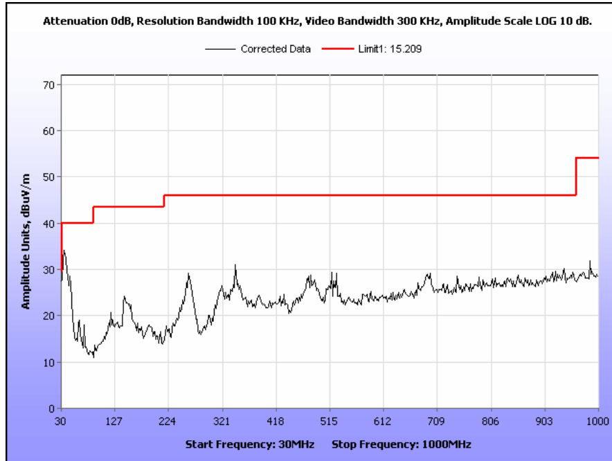
Plot 37. Radiated Spurious Emissions, Mid Channel, 802.11b, 30 MHz – 1 GHz
