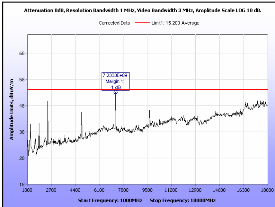
Plot 66. Radiated Spurious Emissions, Low Channel, 802.11b, 1 GHz – 18 GHz, 900 MHz TX
