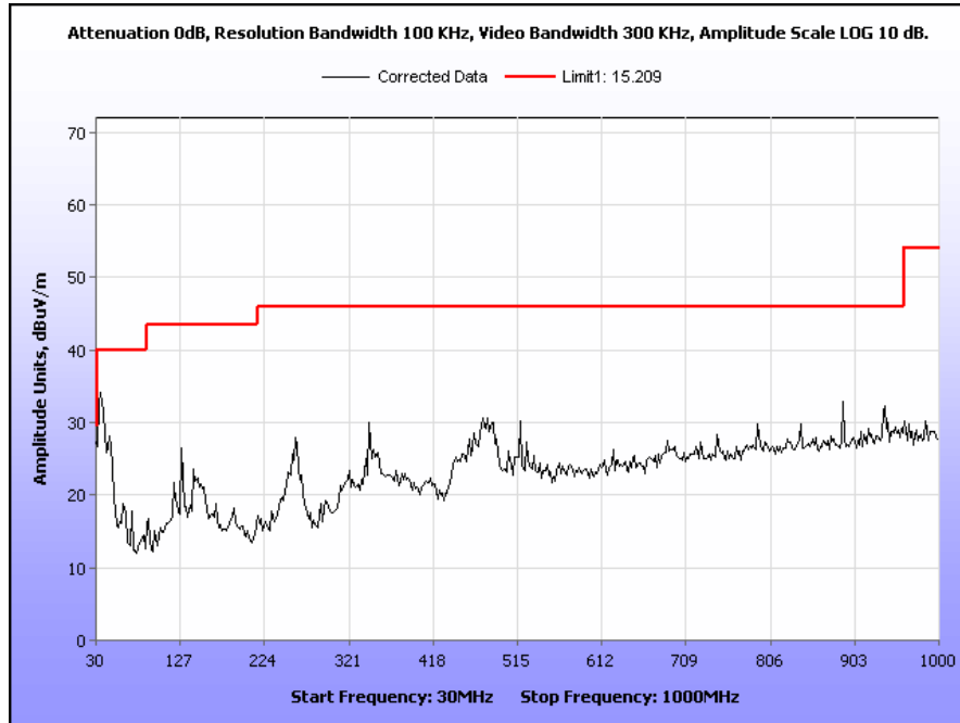
Plot 47. Radiated Spurious Emissions, Low Channel, 802.11n, 30 MHz – 1 GHz
