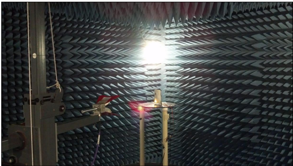
Photograph 6. Radiated Spurious Emissions, Test Setup, Above 1 GHz
