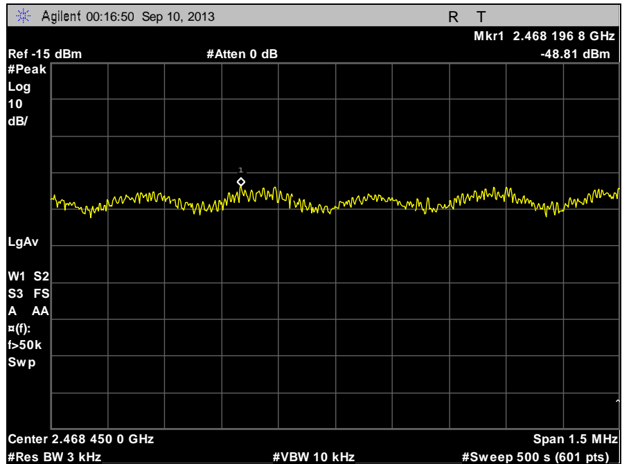
Plot 103. Peak Power Spectral Density, High Channel, 802.11g
