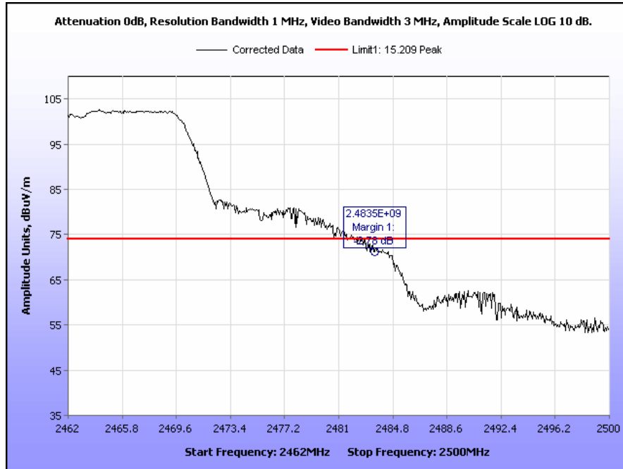
Plot 59. Radiated Band Edge, High Channel, 802.11g, Peak
