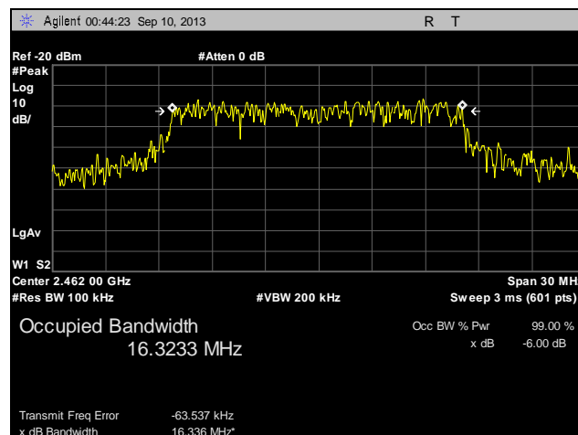
Plot 15. 6 dB Occupied Bandwidth, High Channel, 802.11n
