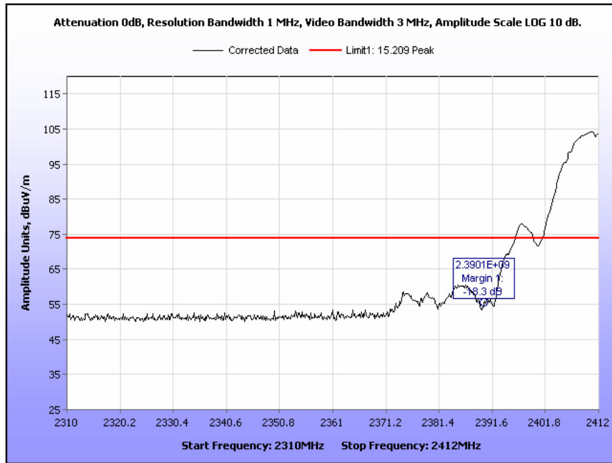
Plot 53. Radiated Band Edge, Low Channel, 802.11b, Peak
