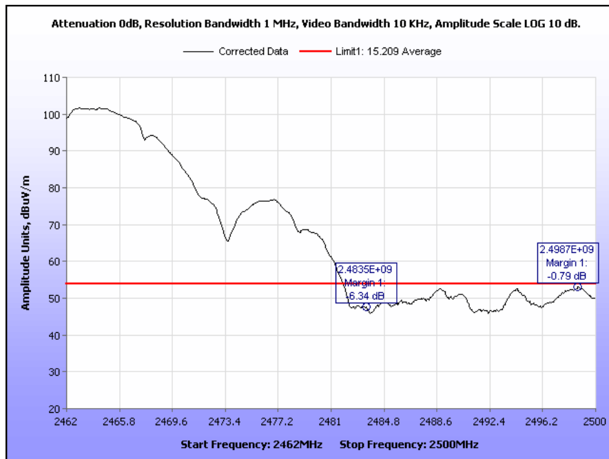
Plot 56. Radiated Band Edge, High Channel, 802.11b, Average
