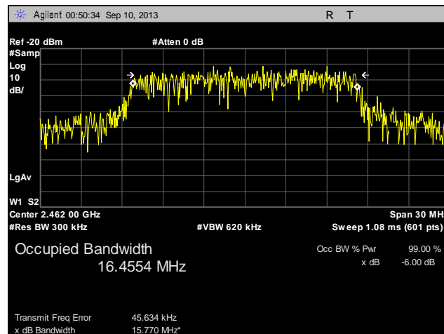
Plot 24. 99% Occupied Bandwidth, High Channel, 802.11n
