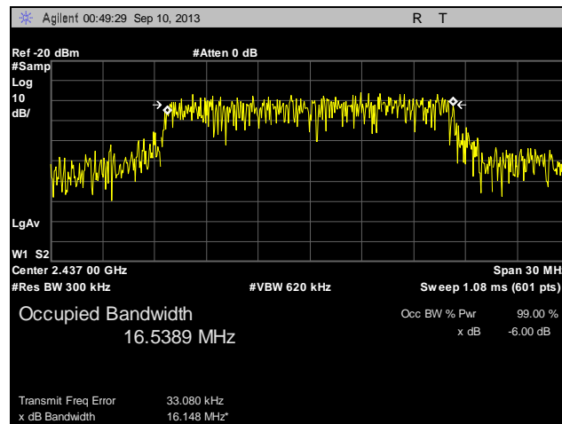
Plot 23. 99% Occupied Bandwidth, Mid Channel, 802.11n
