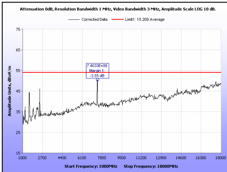
Plot 46. Radiated Spurious Emissions, High Channel, 802.11g, 1 GHz – 18 GHz, Peak under Average
