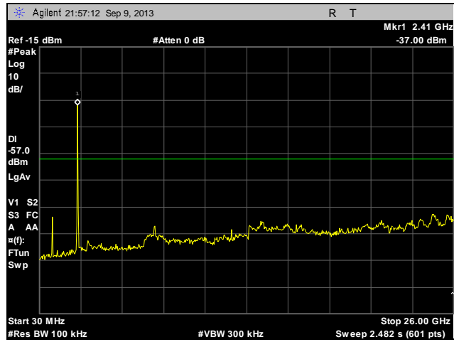
Plot 86. Conducted Spurious Emissions, Low Channel, 802.11g, 30 MHz – 26 GHz
