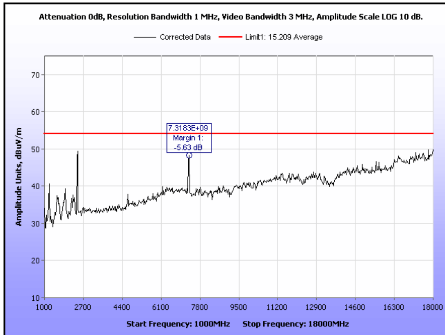
Plot 50. Radiated Spurious Emissions, Mid Channel, 802.11n, 1 GHz – 18 GHz, Peak under Average
