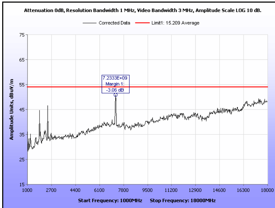
Plot 42. Radiated Spurious Emissions, Low Channel, 802.11g, 1 GHz – 18 GHz, Peak under Average
