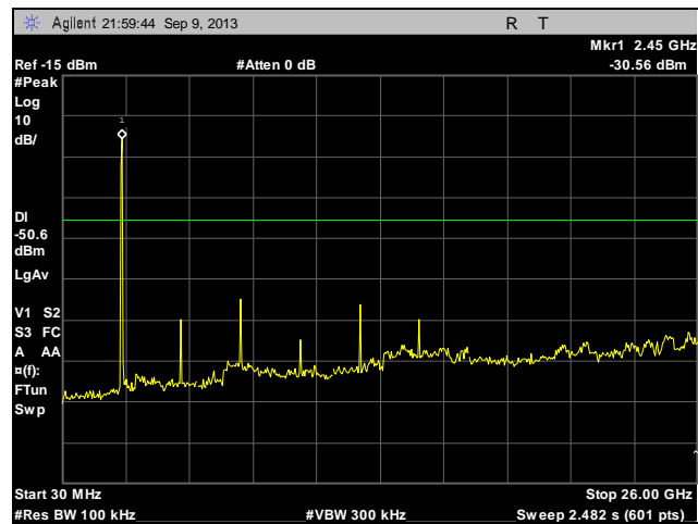
Plot 84. Conducted Spurious Emissions, Mid Channel, 802.11b, 30 MHz – 26 GHz
