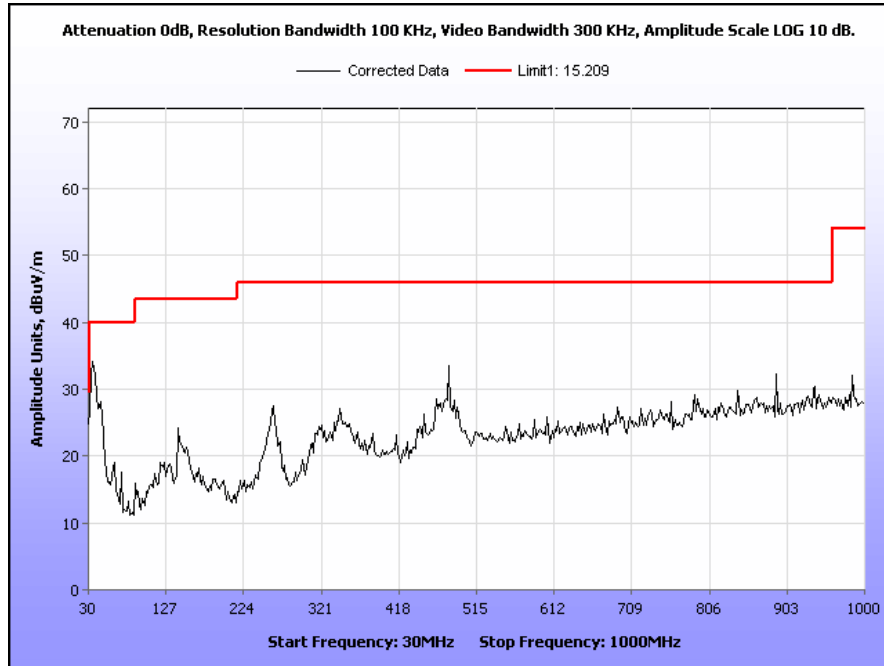
Plot 43. Radiated Spurious Emissions, Mid Channel, 802.11g, 30 MHz – 1 GHz
