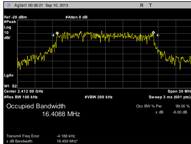
Plot 13. 6 dB Occupied Bandwidth, Low Channel, 802.11n
