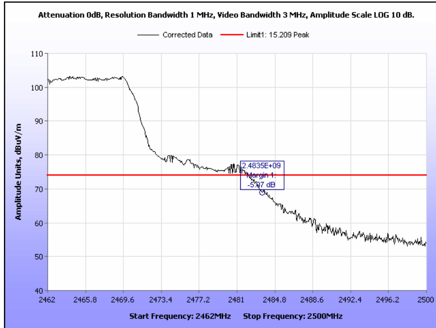
Plot 63. Radiated Band Edge, High Channel, 802.11n, Peak
