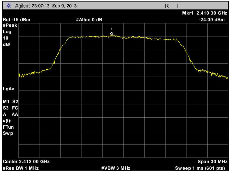
Plot 104. Peak Power Spectral Density, Low Channel, 802.11n, Peak Search
