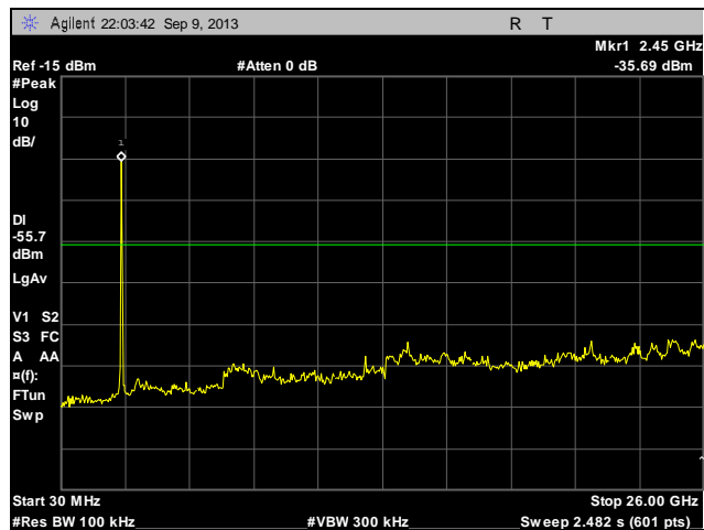
Plot 88. Conducted Spurious Emissions, High Channel, 802.11g, 30 MHz – 26 GHz
