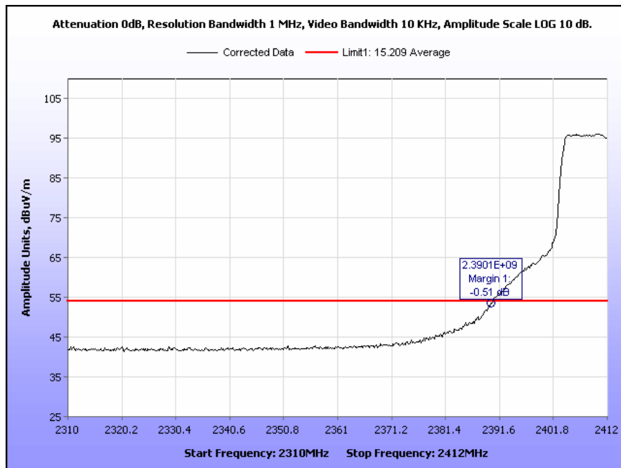
Plot 58. Radiated Band Edge, Low Channel, 802.11g, Average
