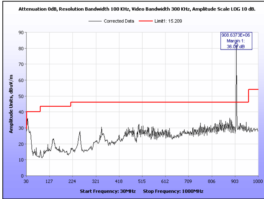
Plot 79. Radiated Spurious Emissions, Mid Channel, 802.11n, 30 MHz – 1 GHz, 900 MHz TX
