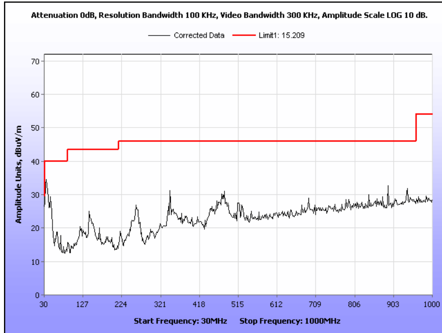
Plot 45. Radiated Spurious Emissions, High Channel, 802.11g, 30 MHz – 1 GHz
