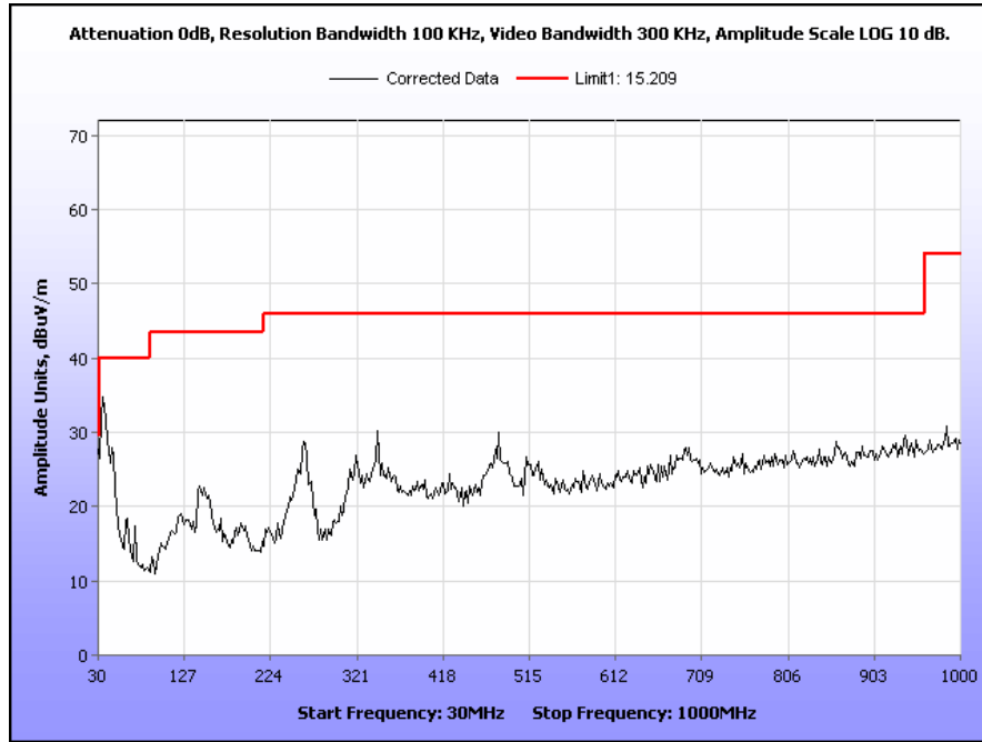
Plot 41. Radiated Spurious Emissions, Low Channel, 802.11g, 30 MHz – 1 GHz
