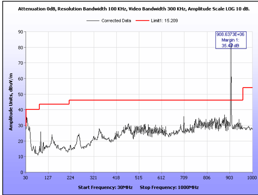
Plot 75. Radiated Spurious Emissions, High Channel, 802.11g, 30 MHz – 1 GHz, 900 MHz TX
