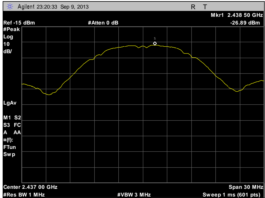
Plot 94. Peak Power Spectral Density, Mid Channel, 802.11b, Peak Search
