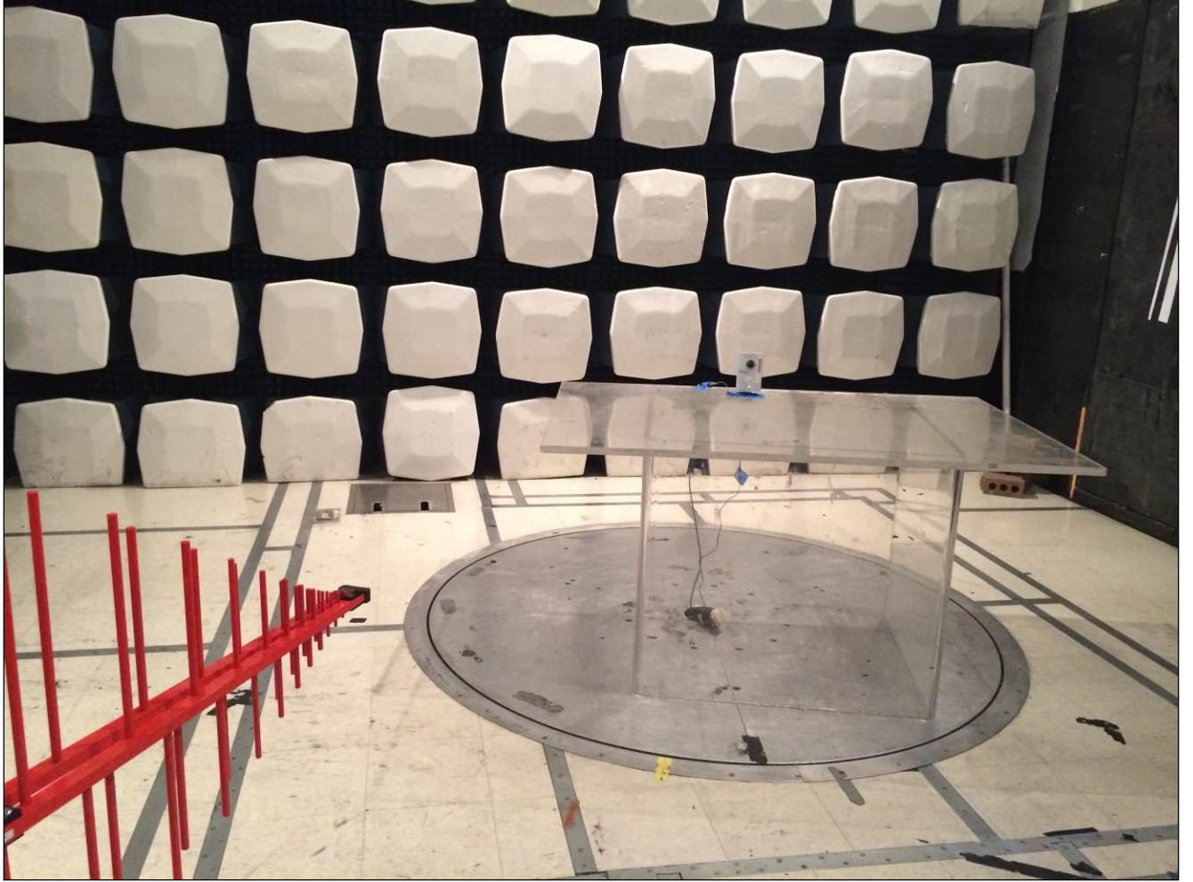
Photograph 5. Radiated Spurious Emissions, Test Setup, 2
