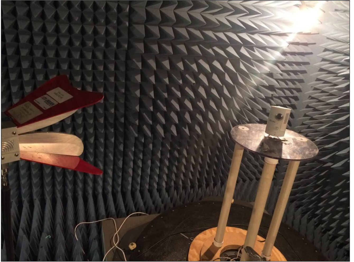
Photograph 4. Radiated Spurious Emissions, Test Setup, 1
