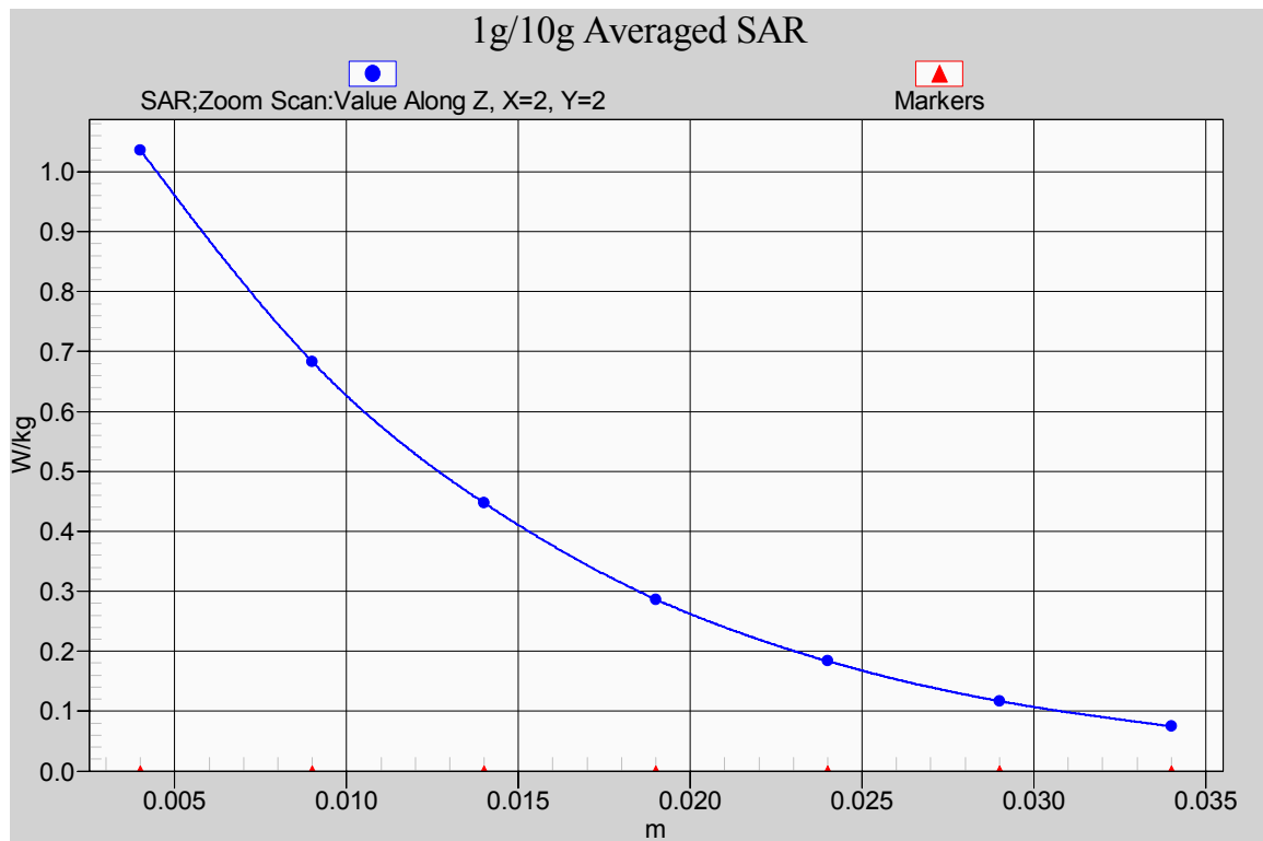
Fig. 16-1 Z-Scan at power reference point (1900 MHz CH810)
