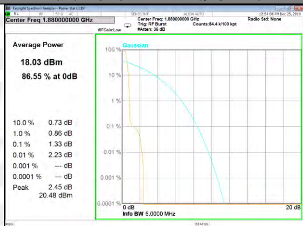
Band 2-15KHz-1#0-QPSK-Mid
