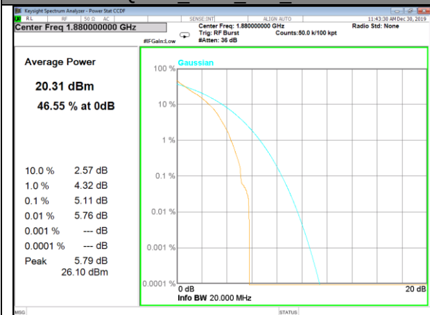
QPSK_3M_6#0_Mid
