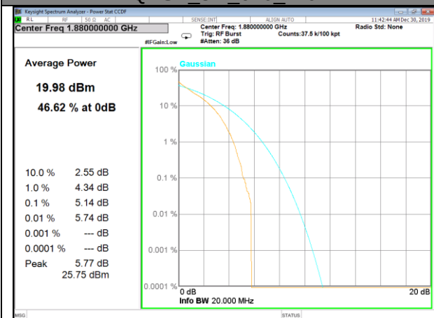
QPSK_5M_6#0_Mid
