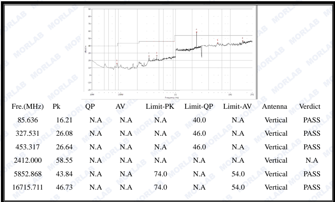
(Antenna Vertical, 30MHz to 25GHz)
