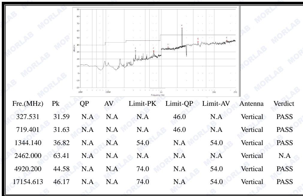
(Antenna Vertical, 30MHz to 25GHz)
