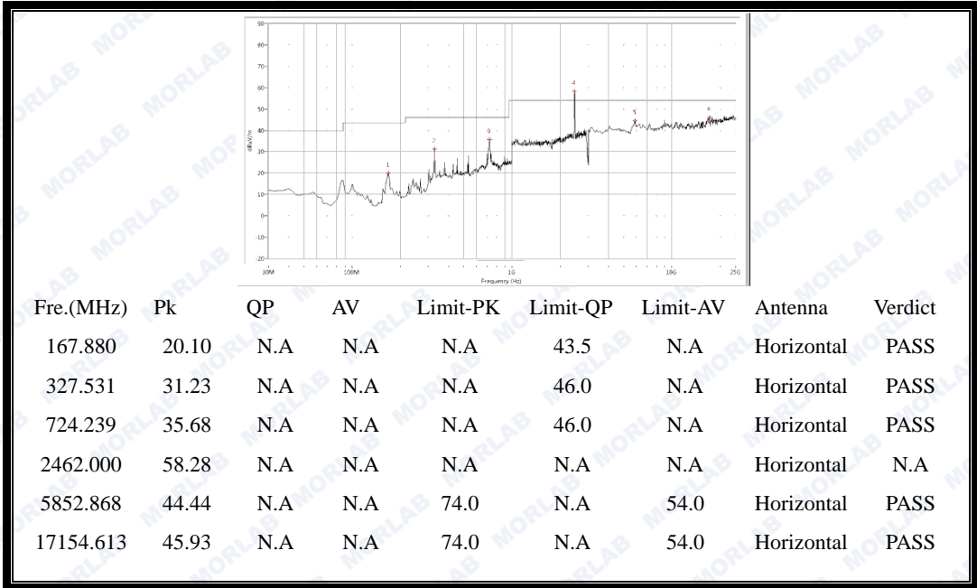
(Antenna Horizontal, 30MHz to 25GHz)
