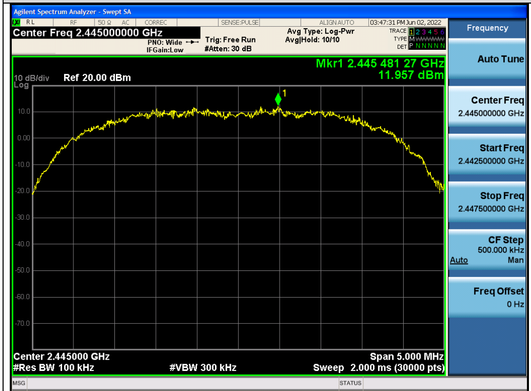
Test_Graph_GFSK_ANT1_2445_Reference Level
