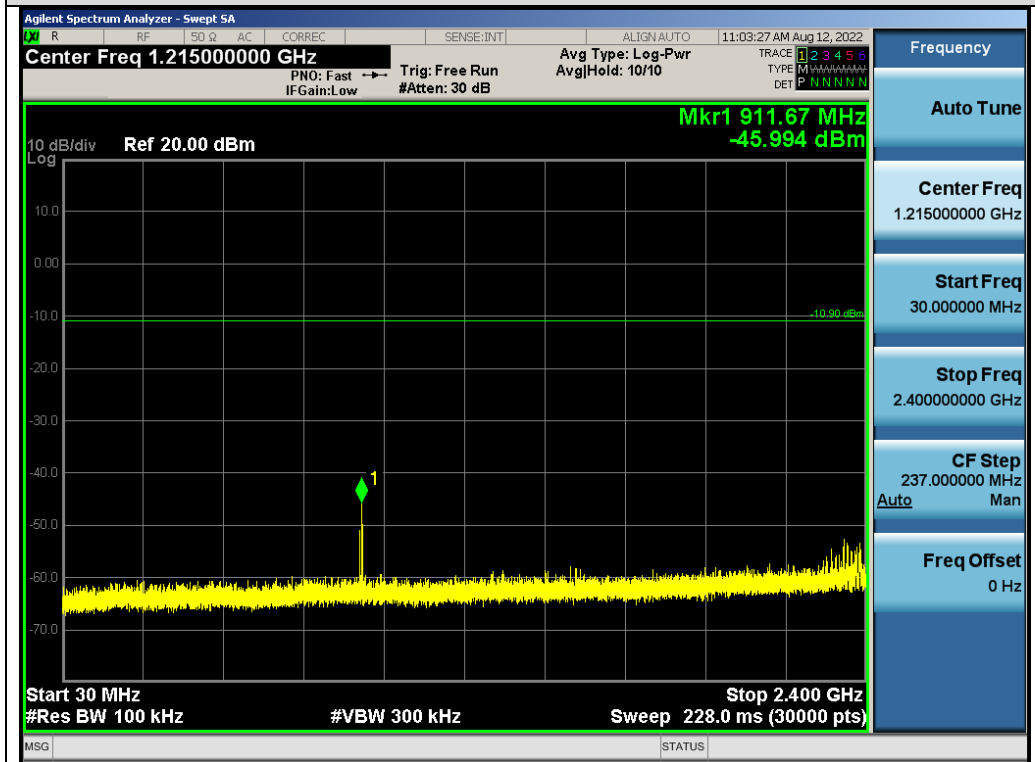
Test_Graph_GFSK_ANT1_2476_Lower Band Emissions
