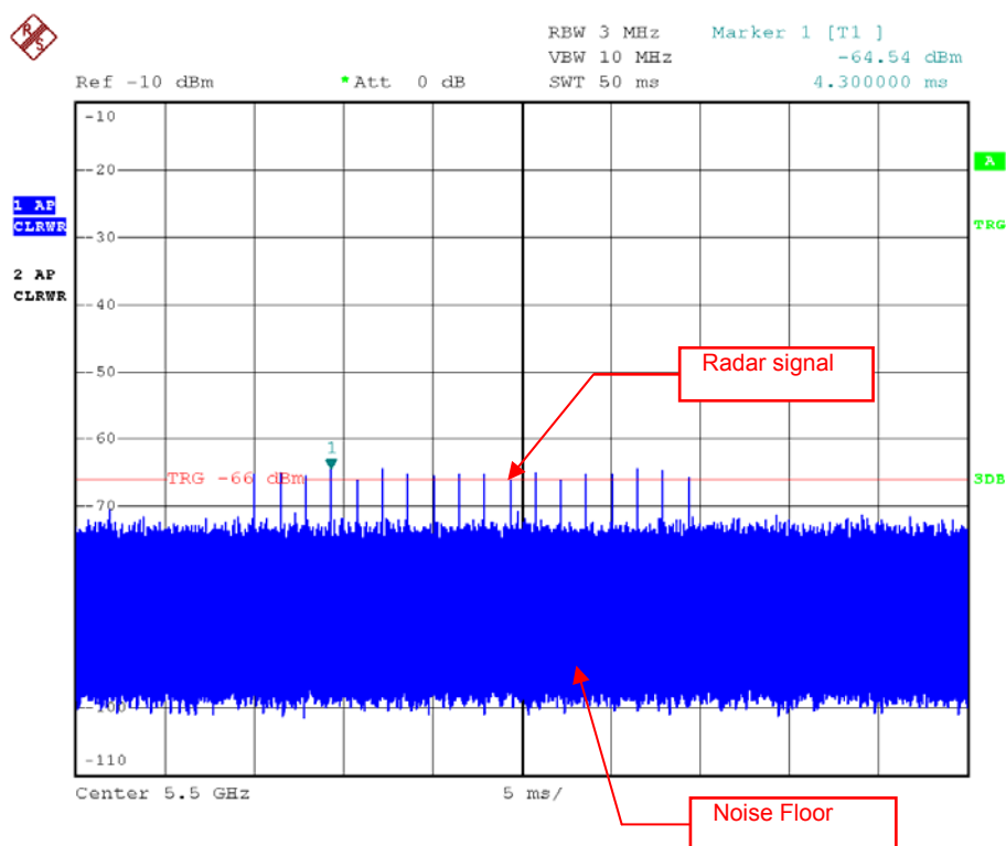
Radar Signal 1
