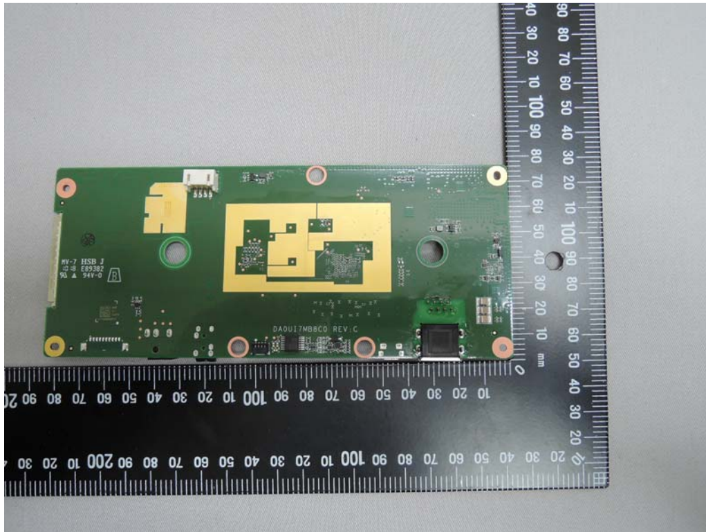
WIFI / BT / ANT+ Antenna
