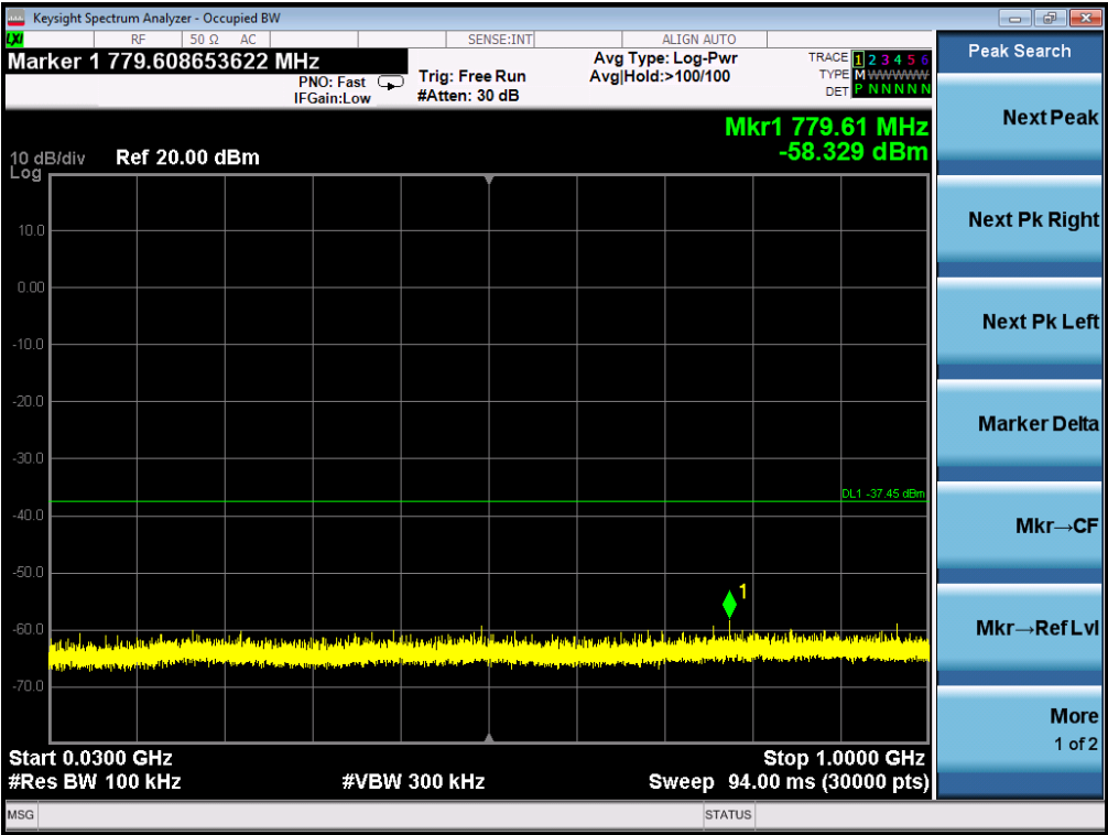
TEST PLOT OF OUT OF BAND EMISSIONS THE WORST CASE OF 802.11n40 FOR MODULATION IN Low CHANNEL
