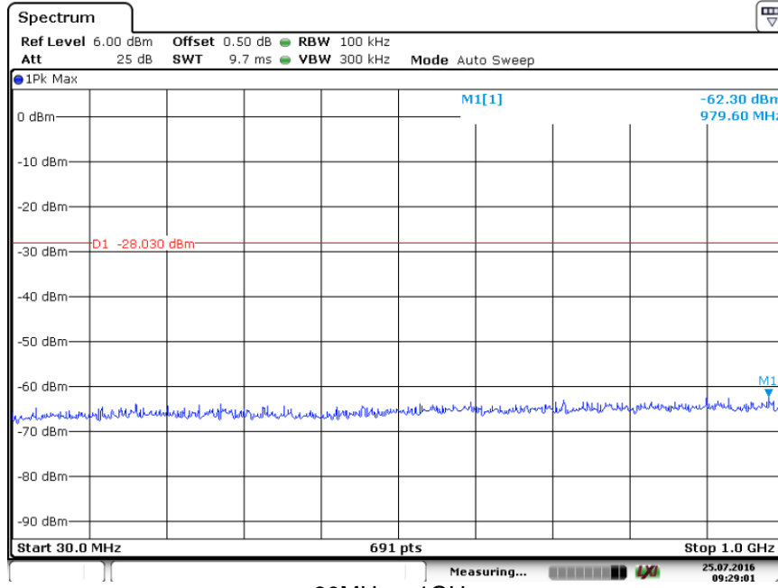
30MHz – 1GHz
