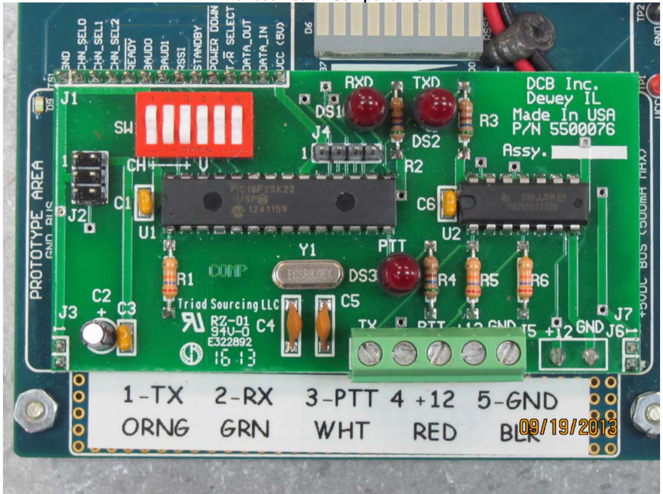
Interface Board: Component Side
