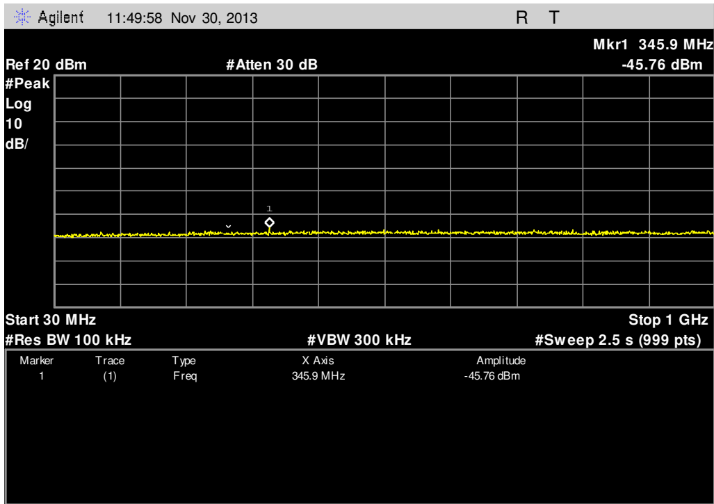
Figure 29: Test figure of conducted emissions in 100kHz Bandwidth, Mode A.1
