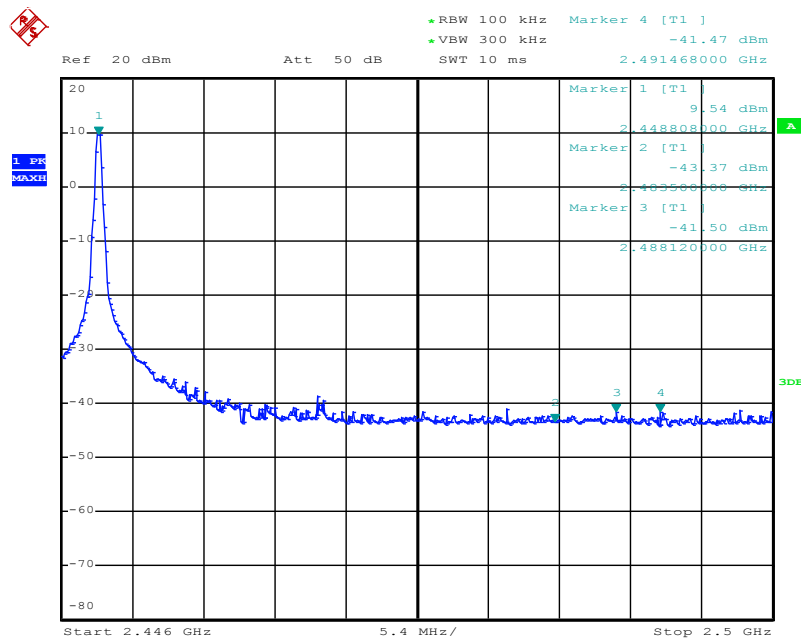
Figure 33: Test figure of Frequency Band Edge in 100kHz Bandwidth, Mode A.3
