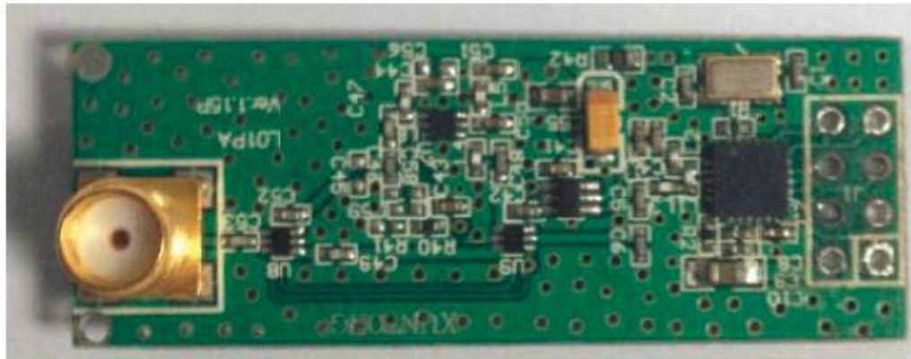
Fig. 5: Internal view of RF Module
