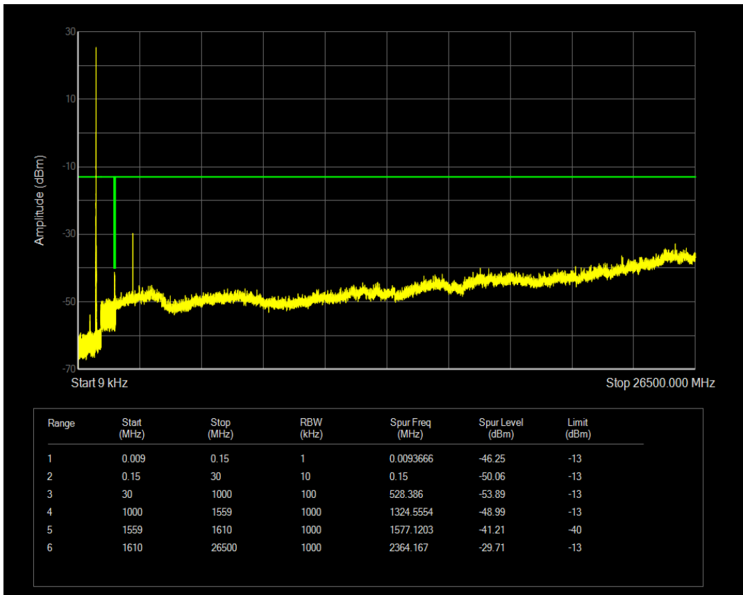
Band14 QAM16 BW=5MHz Channel=23305 RB Size=25 Position=#0
