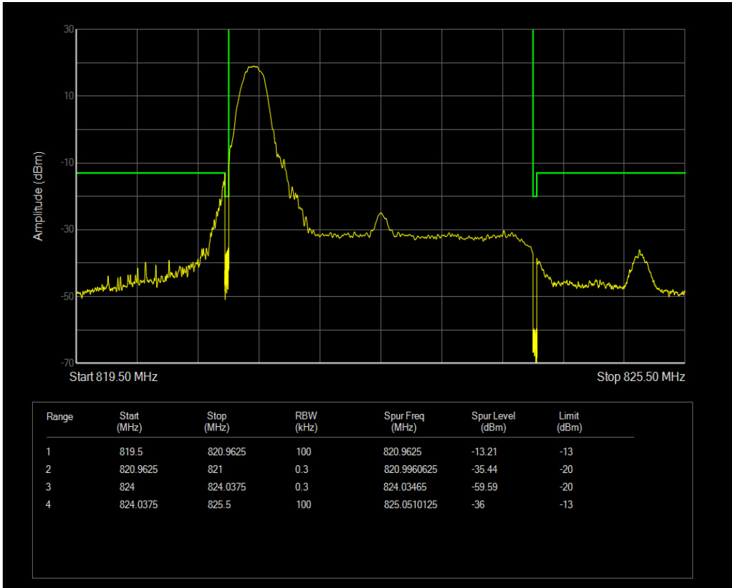
Band26(814-824) QAM16 BW=3MHz Channel=26775 RB Size=1 Position=#Max
