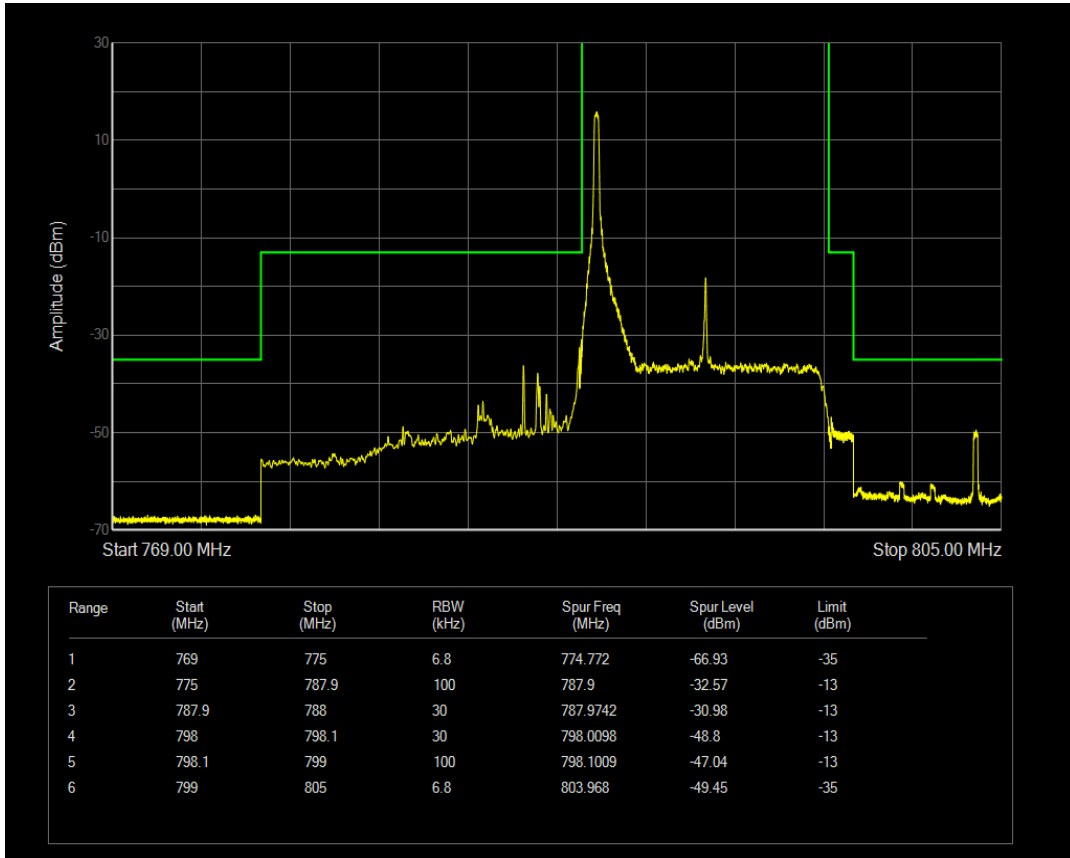
Band14 QAM16 BW=10MHz Channel=23330 RB Size=1 Position=#Max
