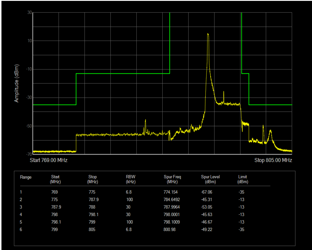
Band14 QAM16 BW=5MHz Channel=23355 RB Size=1 Position=#Max
