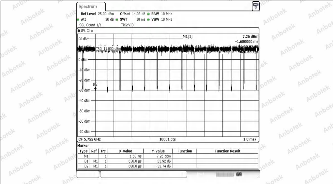
NTNV-11N40SISO-Ant1-5755
