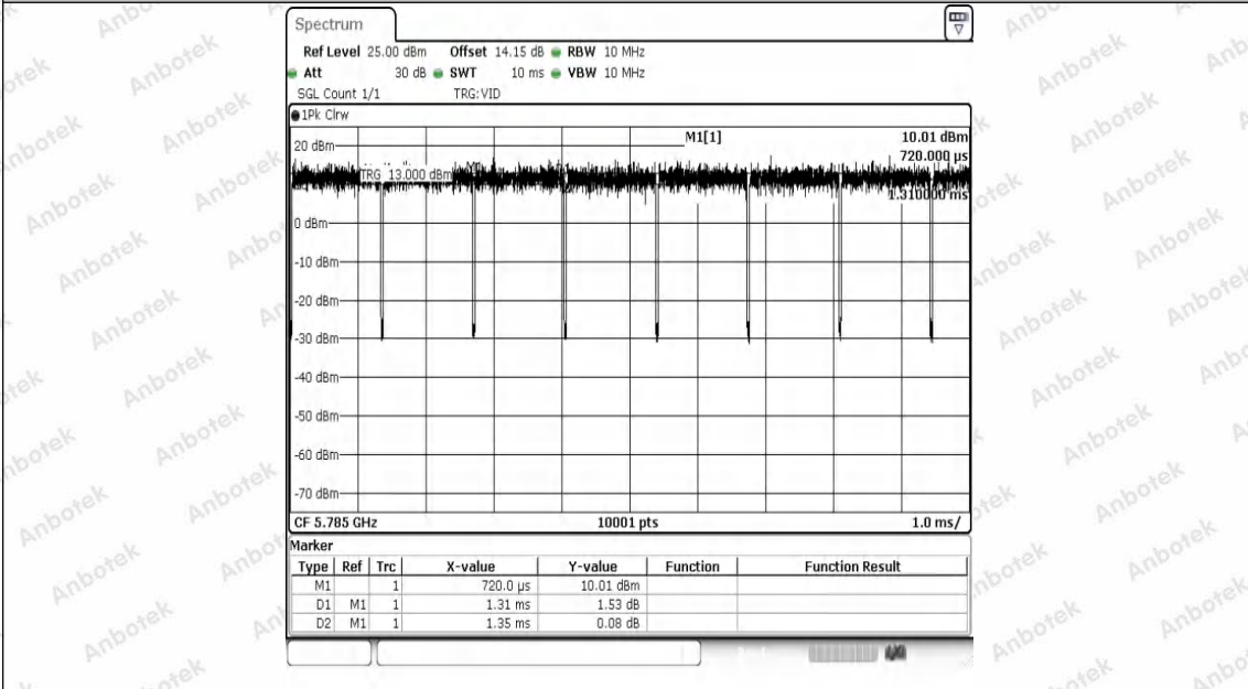
NTNV-11AC20SISO-Ant1-5785
