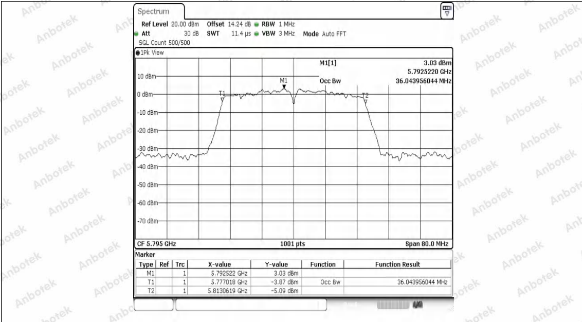
11AC40SISO-Ant1-5795
