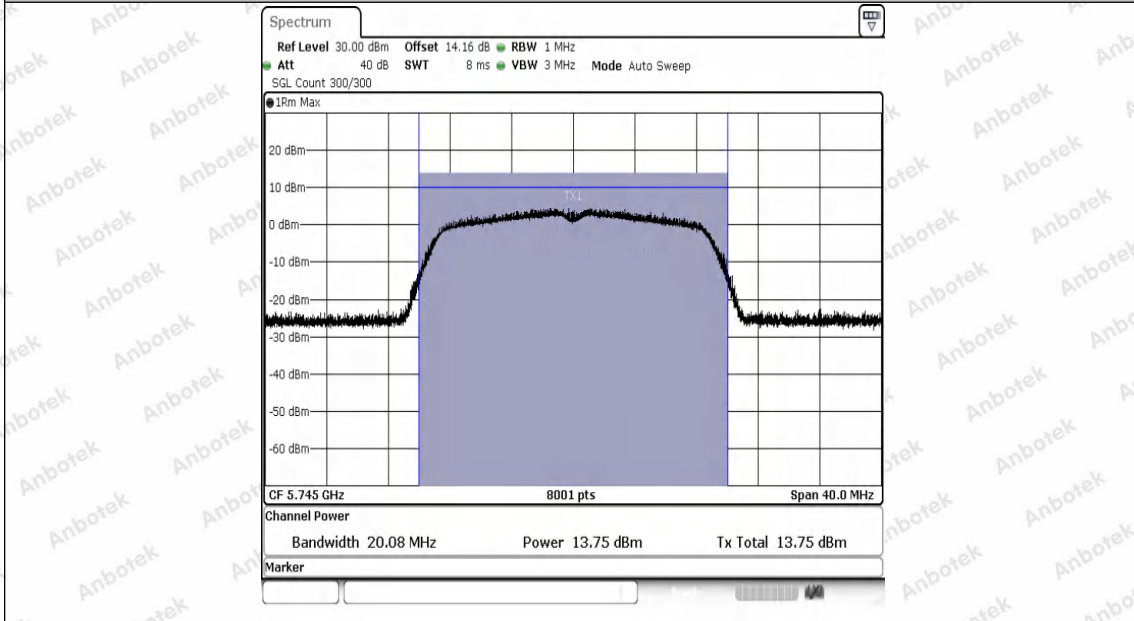
11N20SISO-Ant1-5745-PASS
