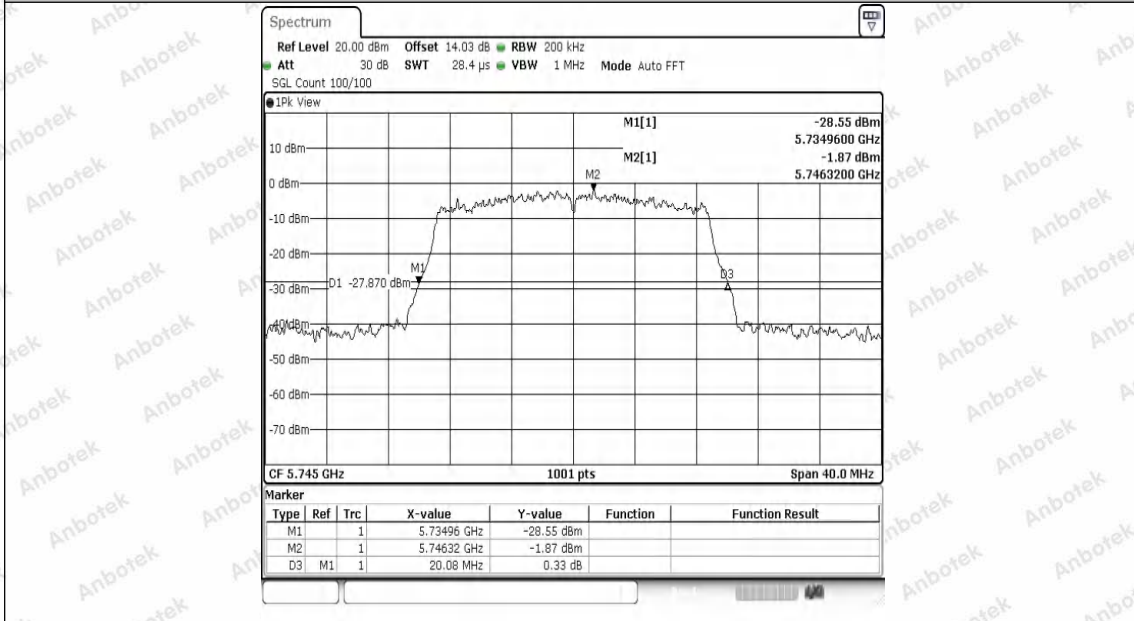
11N20SISO-Ant1-5745
