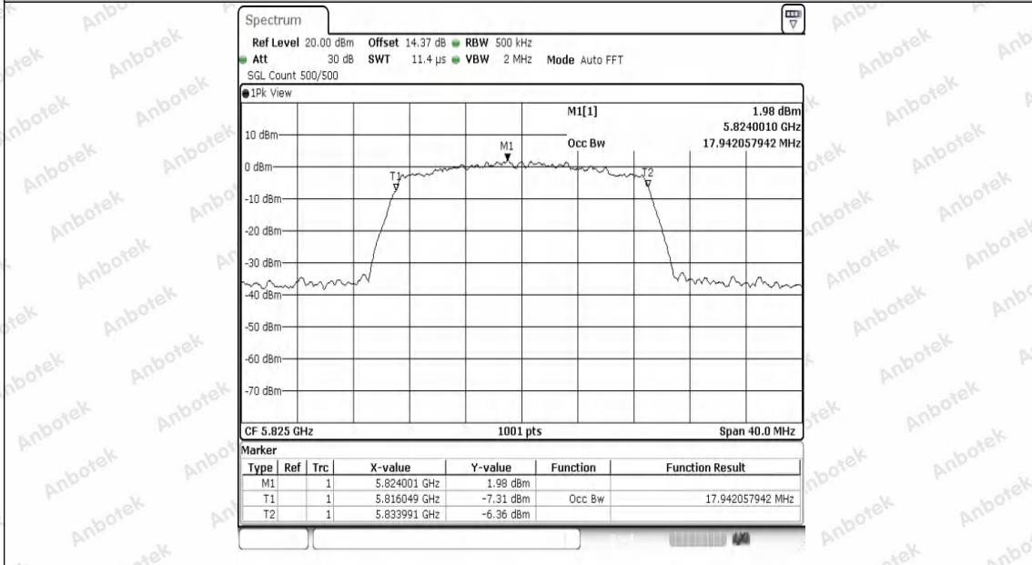
11N20SISO-Ant1-5825
