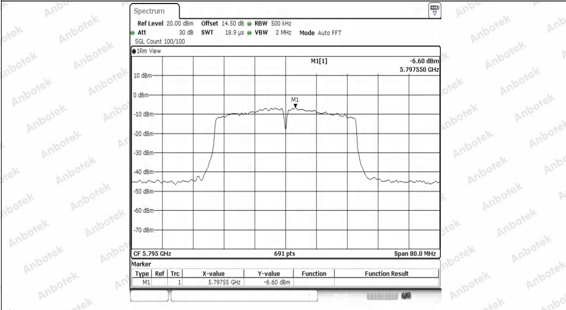
11N40SISO-Ant1-5795-PASS
