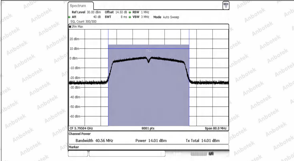
11N40SISO-Ant1-5795-PASS
