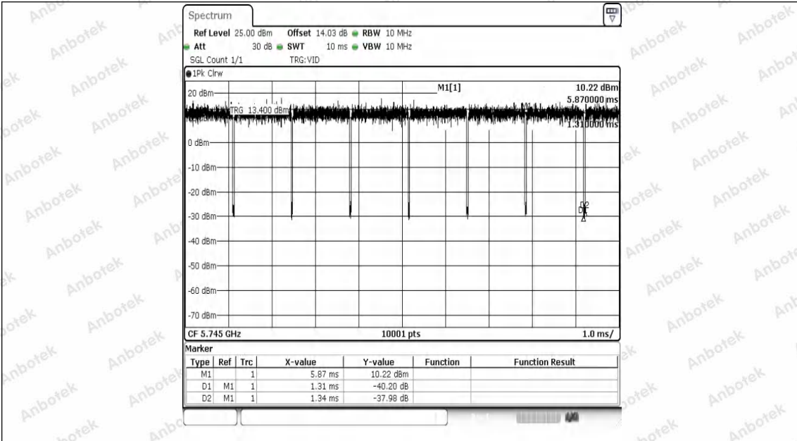
NTNV-11AC20SISO-Ant1-5745
