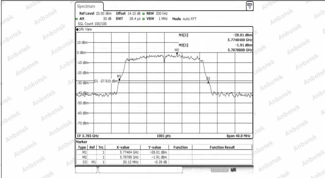
11AC20SISO-Ant1-5785
