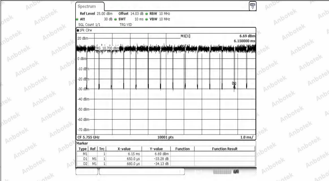
NTNV-11AC40SISO-Ant1-5755
