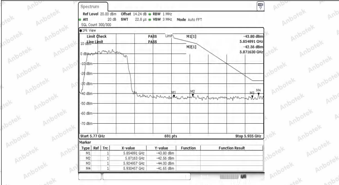
11AC40SISO-Ant1-5795-PASS
