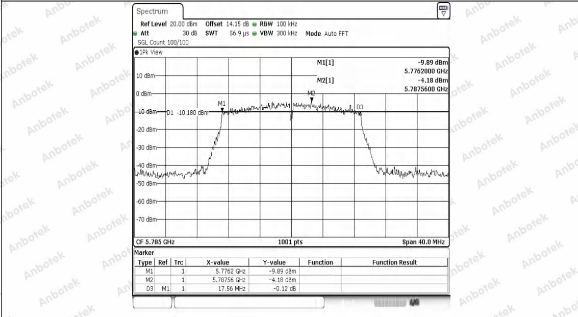
11AC20SISO-Ant1-5785-PASS
