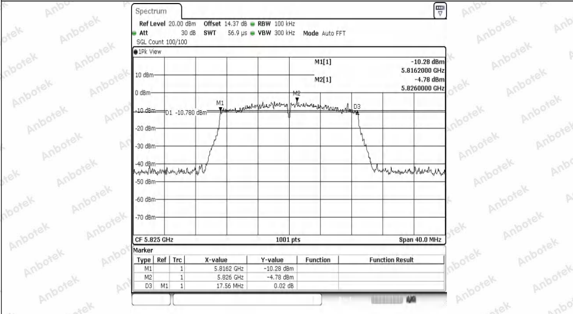
11N20SISO-Ant1-5825-PASS
