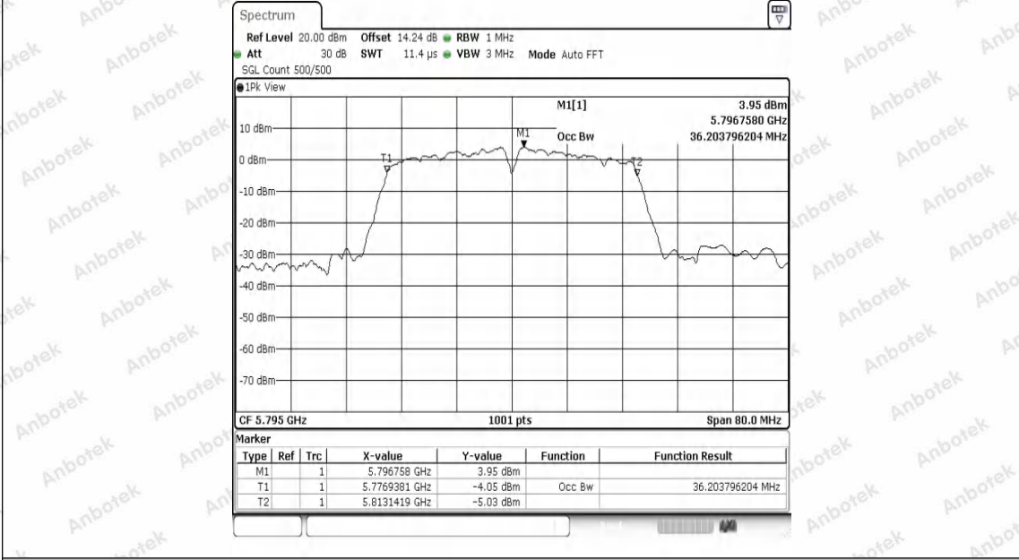
11N40SISO-Ant1-5795
