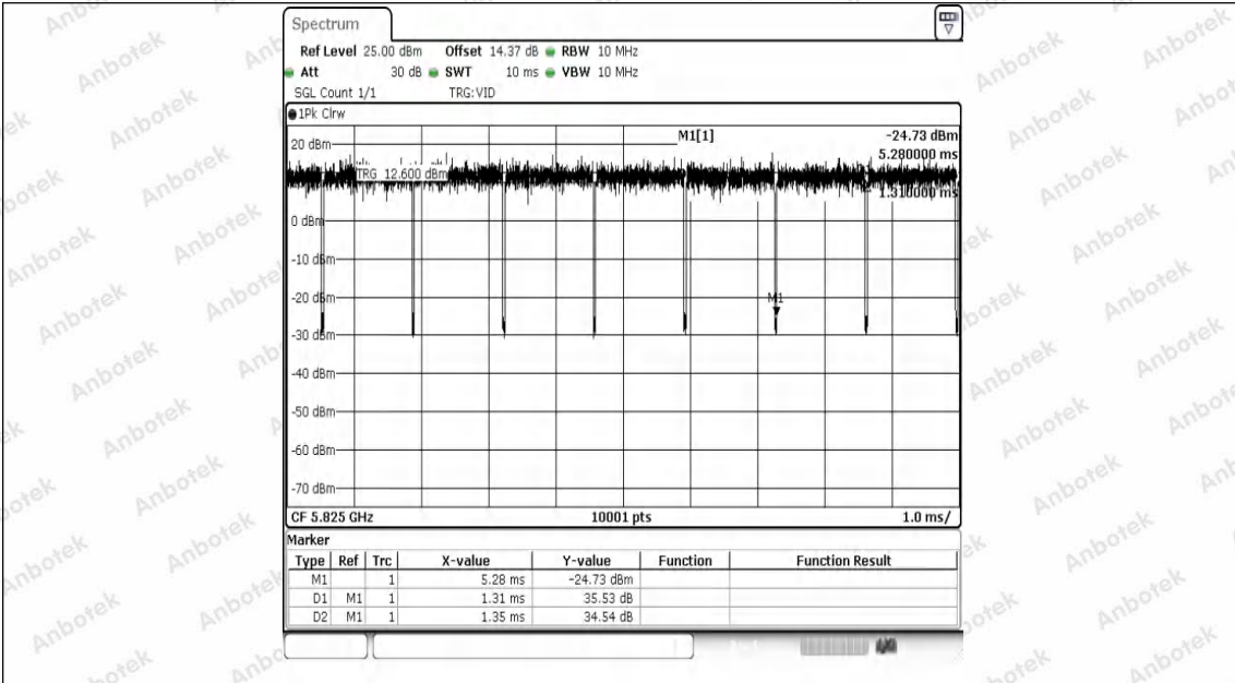
NTNV-11AC20SISO-Ant1-5825
