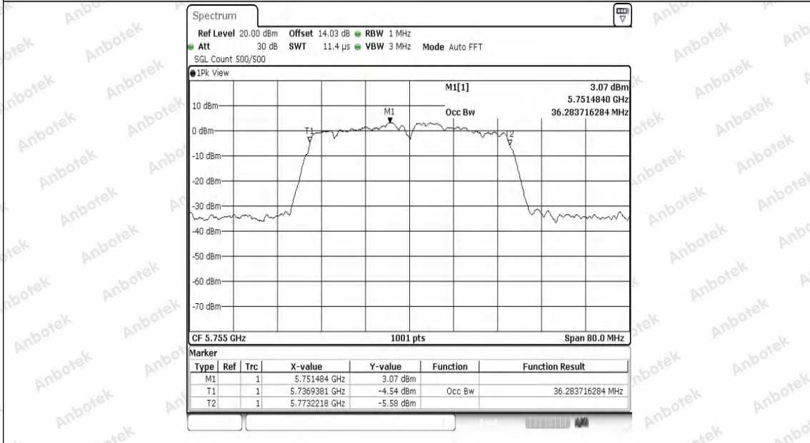
11AC40SISO-Ant1-5755
