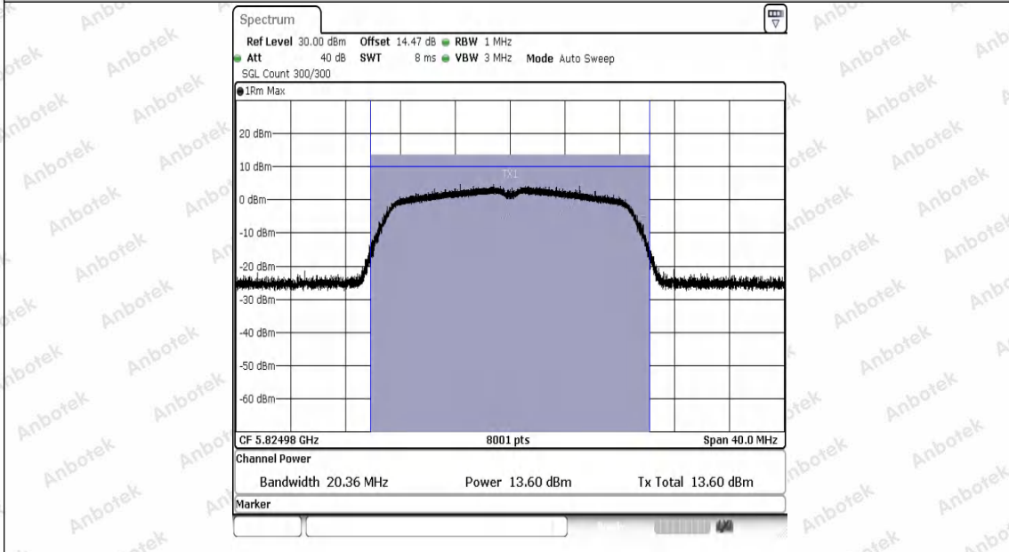
11N20SISO-Ant1-5825-PASS
