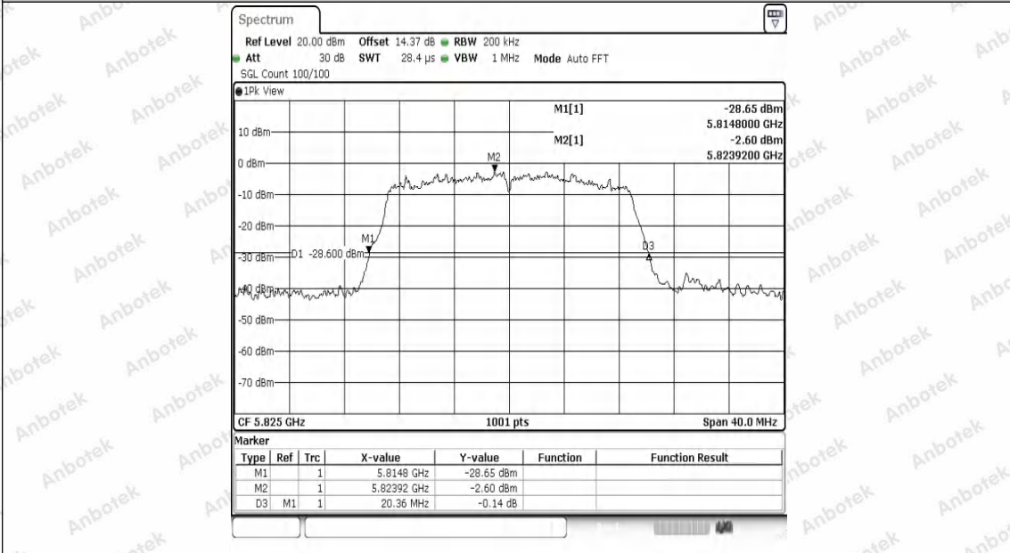
11N20SISO-Ant1-5825
