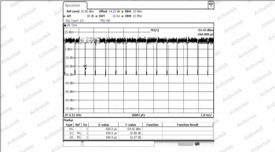
NTNV-11N40SISO-Ant1-5510
