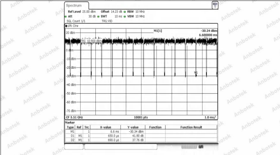
NTNV-11AC40SISO-Ant1-5510
