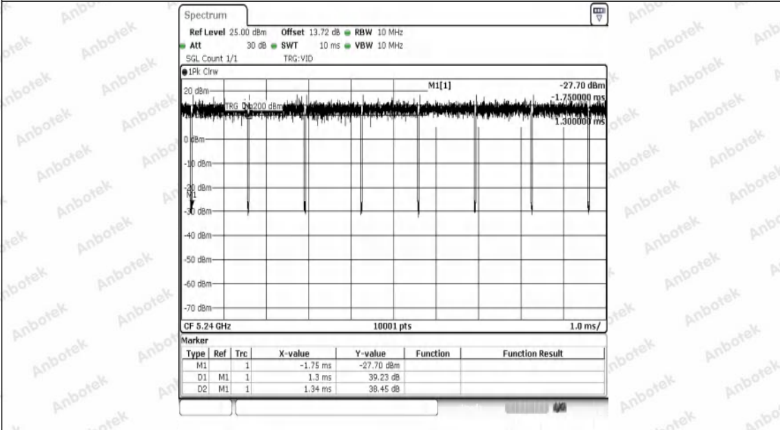
NTNV-11N20SISO-Ant1-5240
