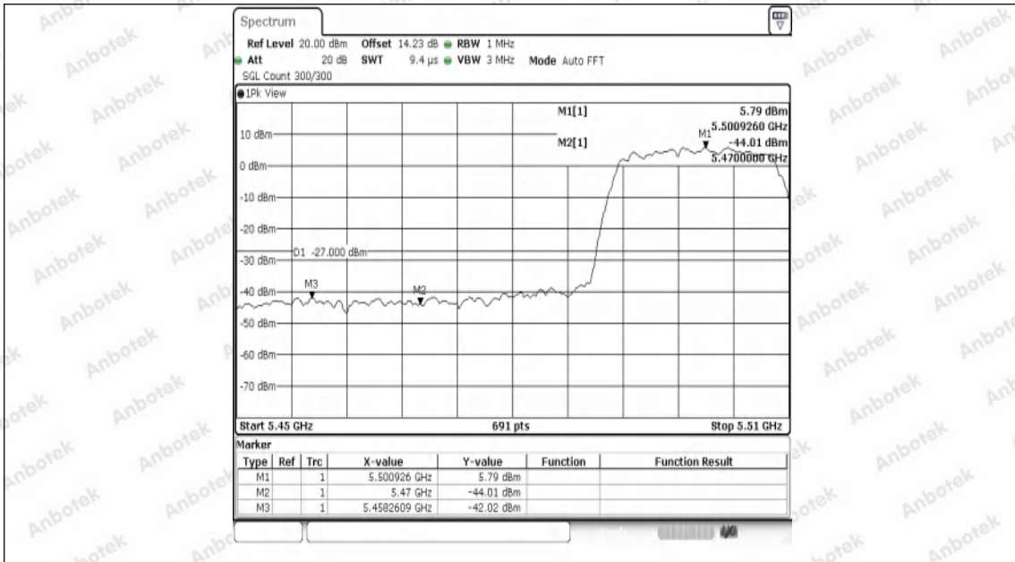
11AC20SISO-Ant1-5500-PASS
