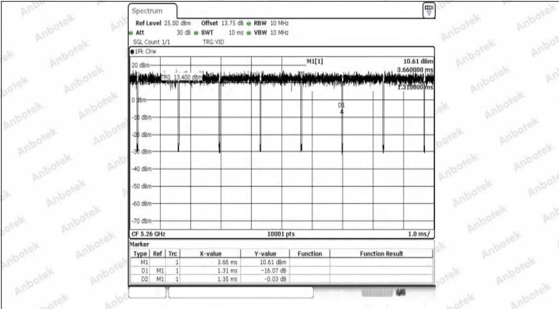
NTNV-11AC20SISO-Ant1-5260
