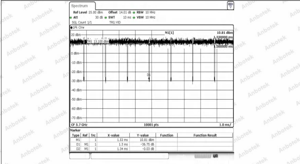
NTNV-11N20SISO-Ant1-5700
