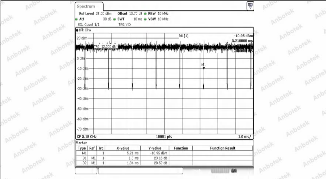
NTNV-11N20SISO-Ant1-5180
