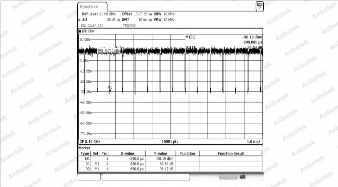
NTNV-11N40SISO-Ant1-5190
