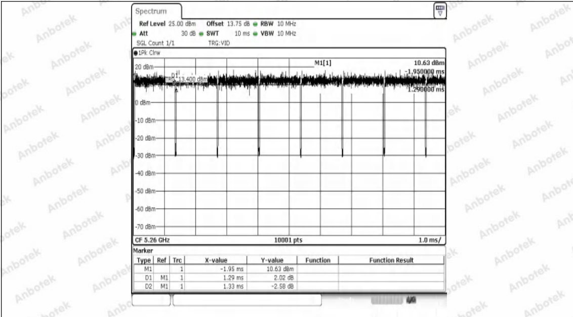
NTNV-11N20SISO-Ant1-5260
