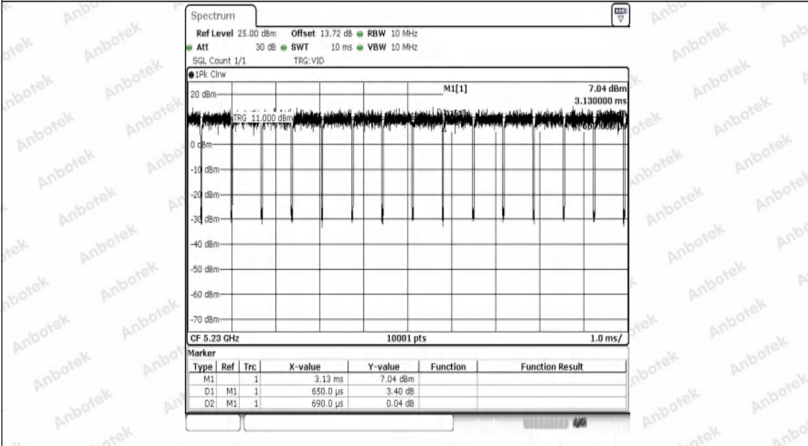
NTNV-11AC40SISO-Ant1-5230
