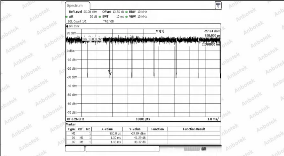
NTNV-11A-Ant1-5260
