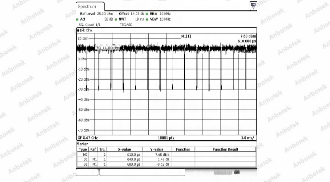
NTNV-11N40SISO-Ant1-5670
