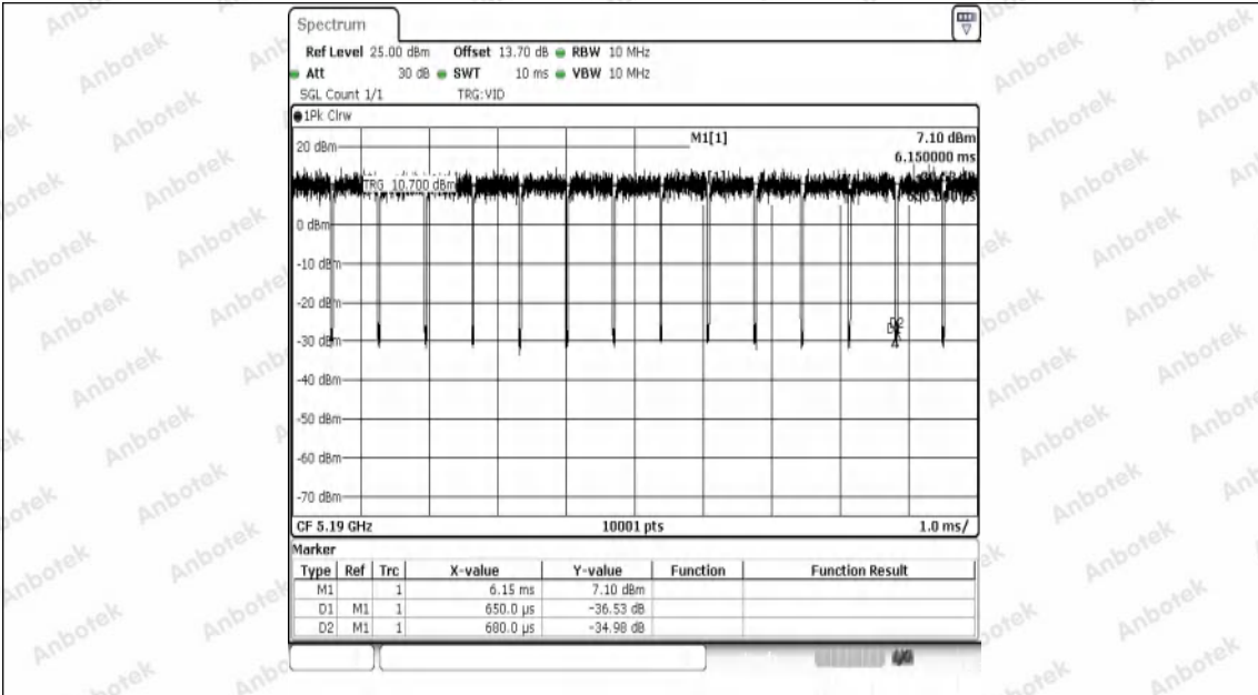
NTNV-11AC40SISO-Ant1-5190
