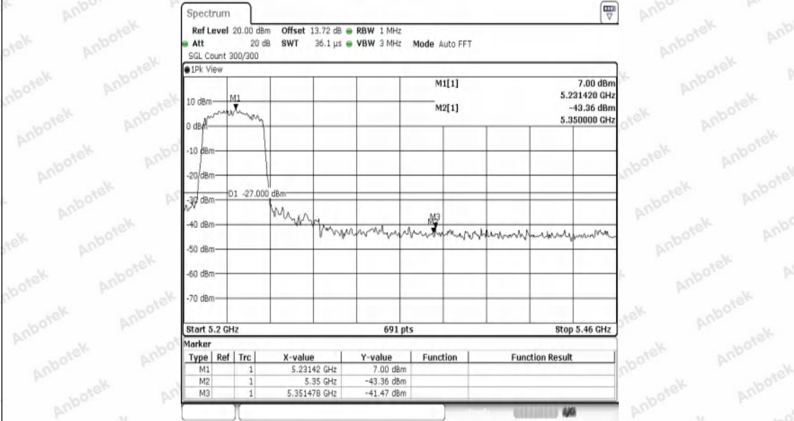
11AC40SISO-Ant1-5230-PASS
