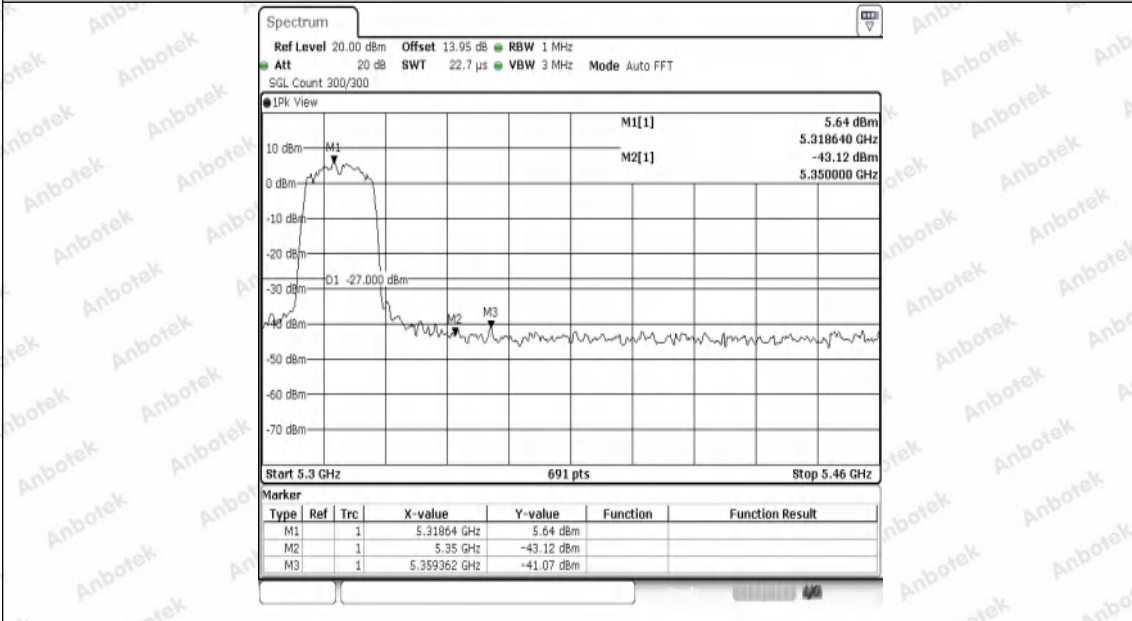
11AC20SISO-Ant1-5320-PASS
