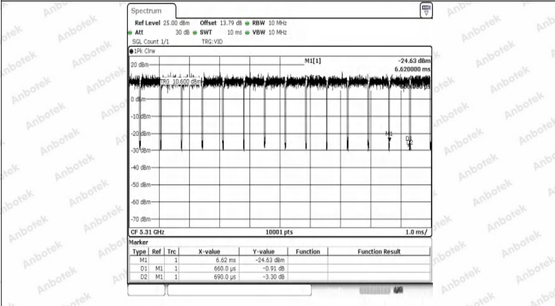
NTNV-11AC40SISO-Ant1-5310
