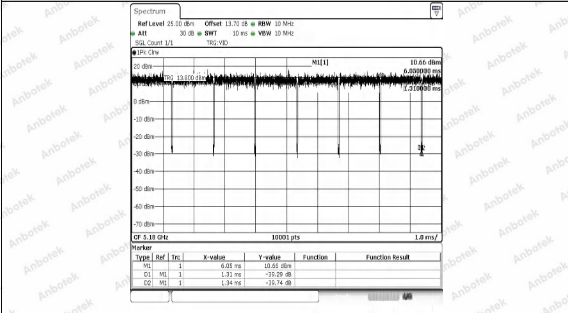
NTNV-11AC20SISO-Ant1-5180
