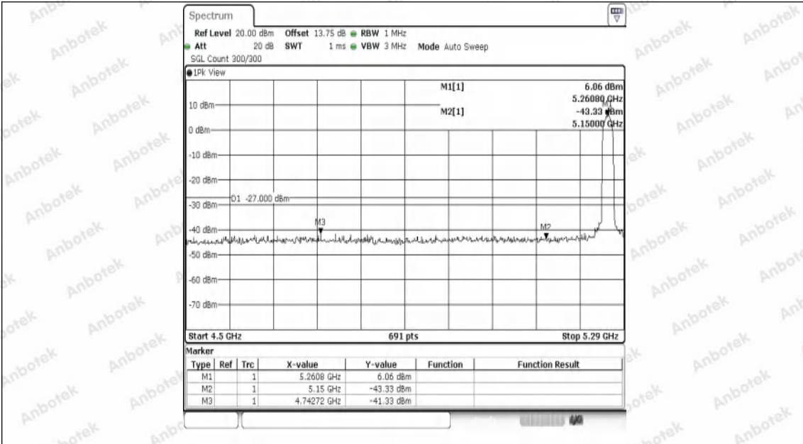
11AC20SISO-Ant1-5260-PASS
