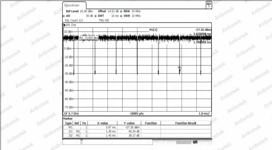
NTNV-11A-Ant1-5700
