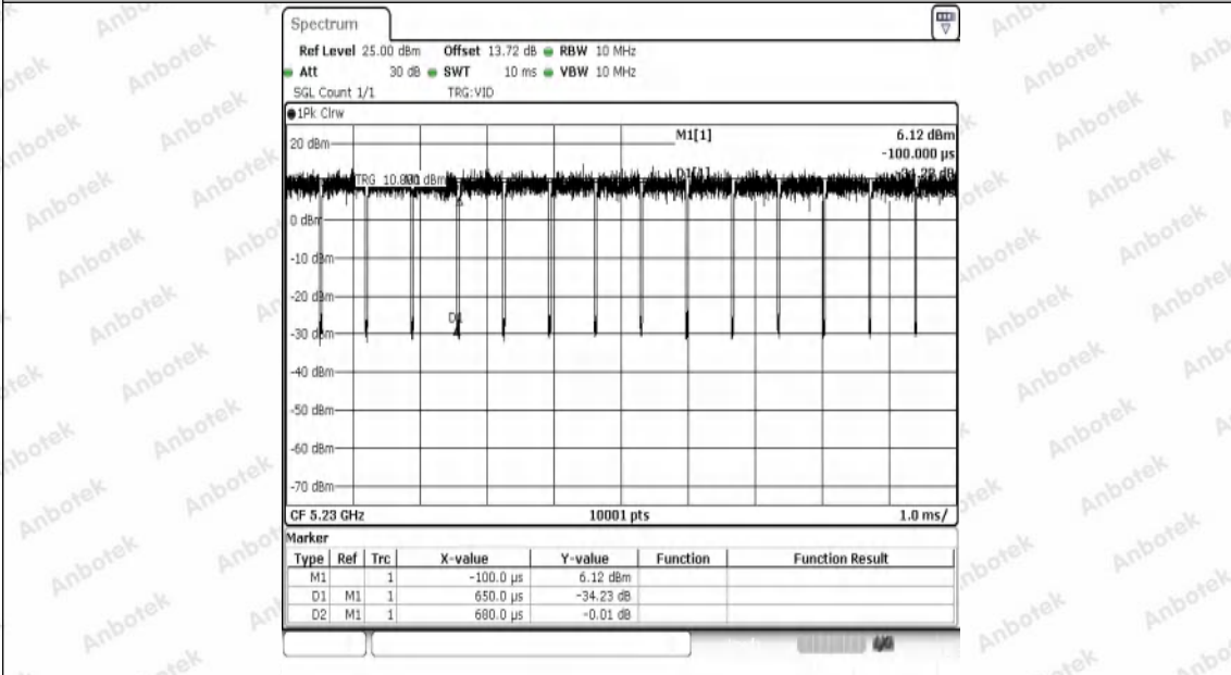
NTNV-11N40SISO-Ant1-5230
