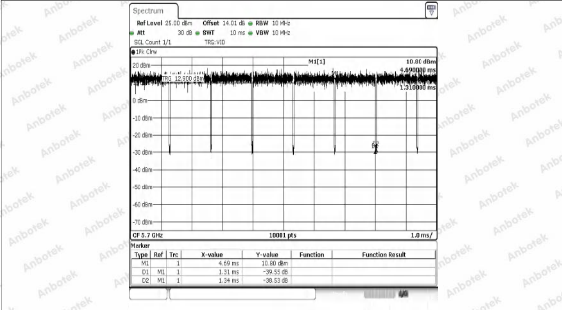
NTNV-11AC20SISO-Ant1-5700
