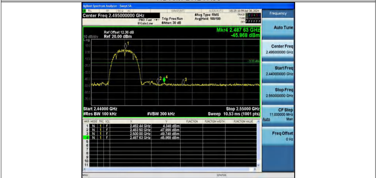
11B-Ant1-2462-PASS
