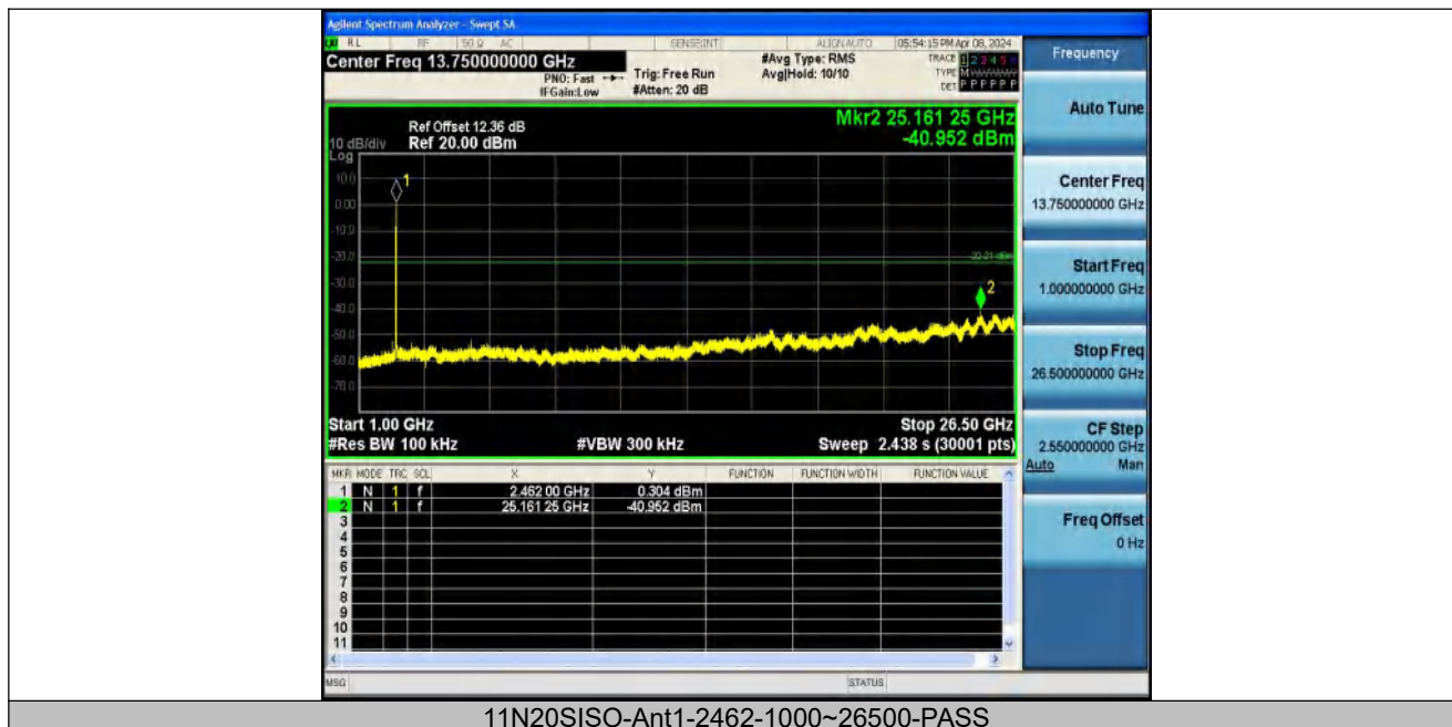
11N20SISO-Ant1-2462-1000~26500-PASS
