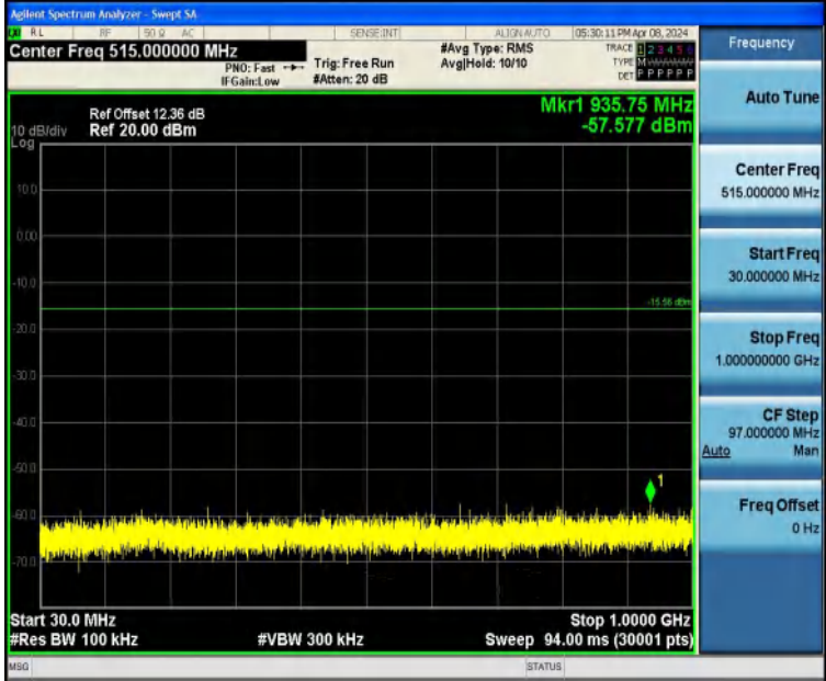
11B-Ant1-2462-30~1000-PASS
