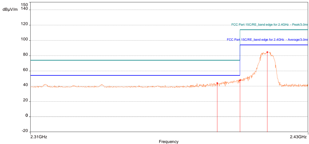
2412MHz Vertical
