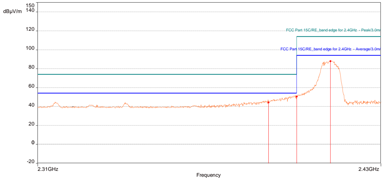
2412MHz Vertical
