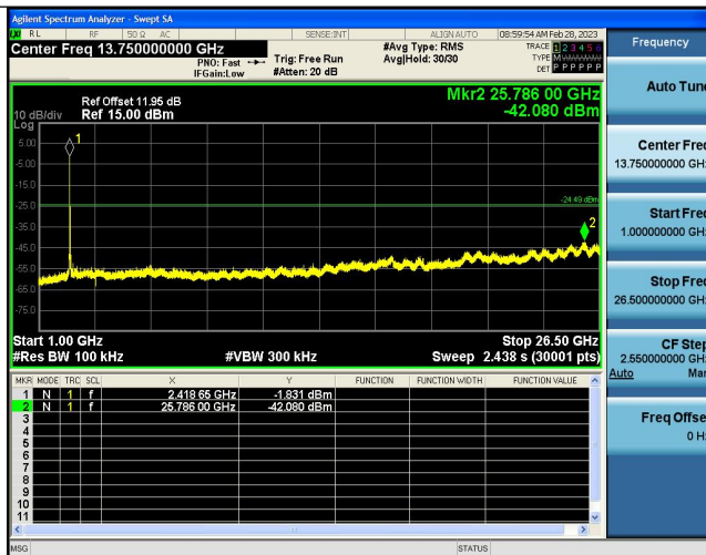
11G-Ant1-2437-0~Reference--1.43
