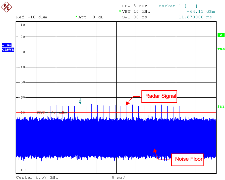
Radar Signal 1 (Test B)
