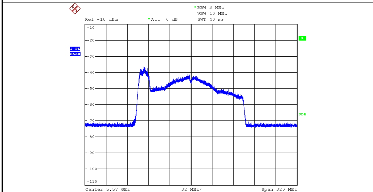
EUT (master) links with Client on 5570 MHz
