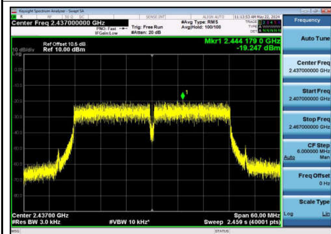
Power spectral density-802.11n(40MHz) ,2437MHz,Ant0
