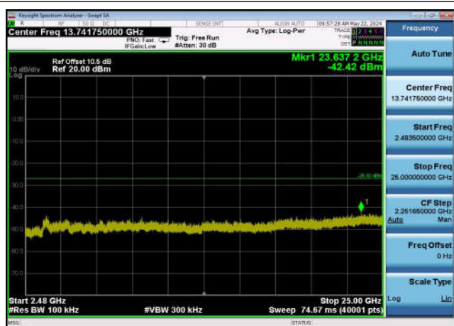
,Plot 4,2483.5MHz~25000MHz-802.11g
