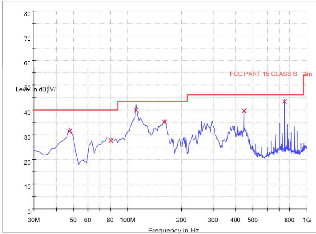
EMI Sweep-3M(30-1G)
