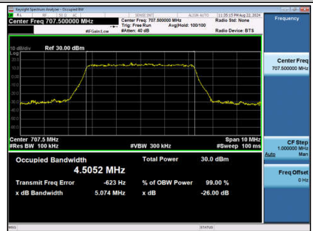
Band12-5MHz-16QAM-23095-25RB#0-PASS
