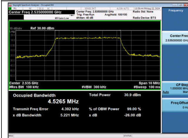
Band7-5MHz-QPSK-21100-25RB#0-PASS
