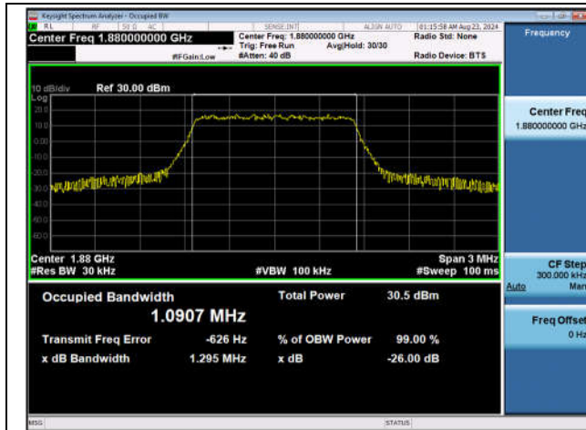
Band2-1.4MHz-QPSK-18900-6RB#0-PASS
