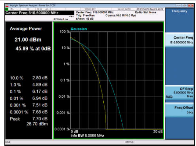
Band26(Part 90)-5MHz-16QAM-26715-25RB#0-PASS
