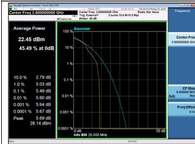
Band41-20MHz-16QAM-40690-1RB#0-PASS
