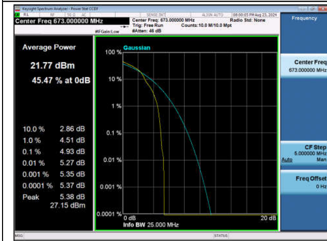
Band71-20MHz-16QAM-133222-1RB#0-PASS
