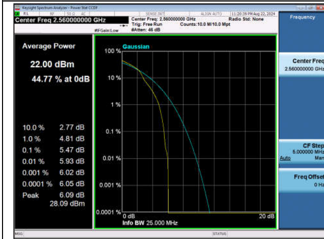
Band7-20MHz-16QAM-21350-1RB#0-PASS
