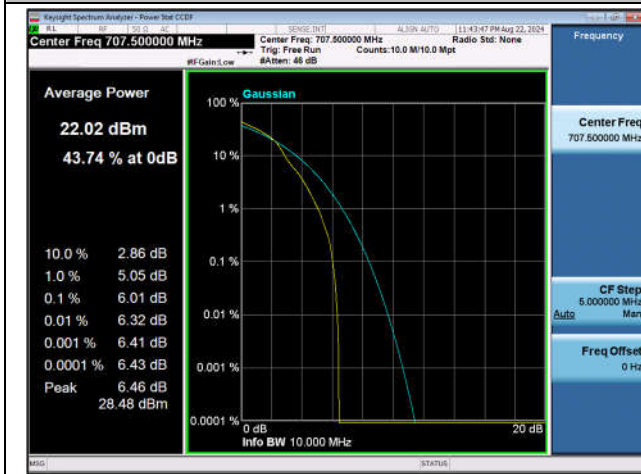
Band12-10MHz-16QAM-23095-1RB#0-PASS
