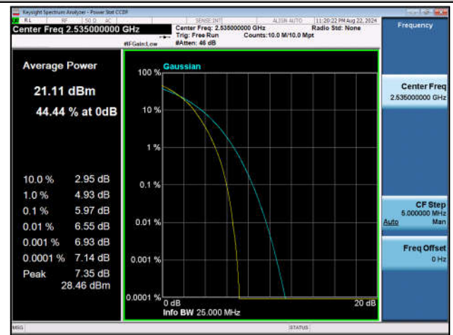
Band7-20MHz-16QAM-21100-100RB#0-PASS
