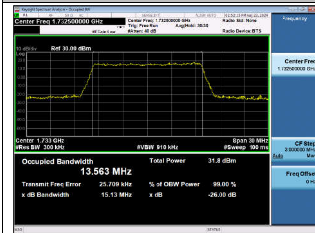
Band4-15MHz-QPSK-20175-75RB#0-PASS
