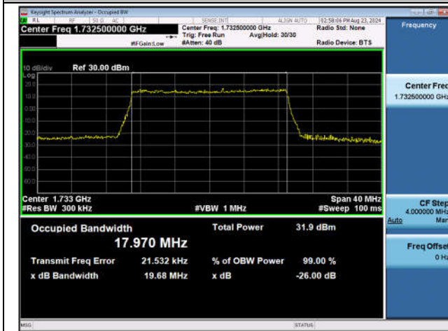
Band4-20MHz-QPSK-20175-100RB#0-PASS
