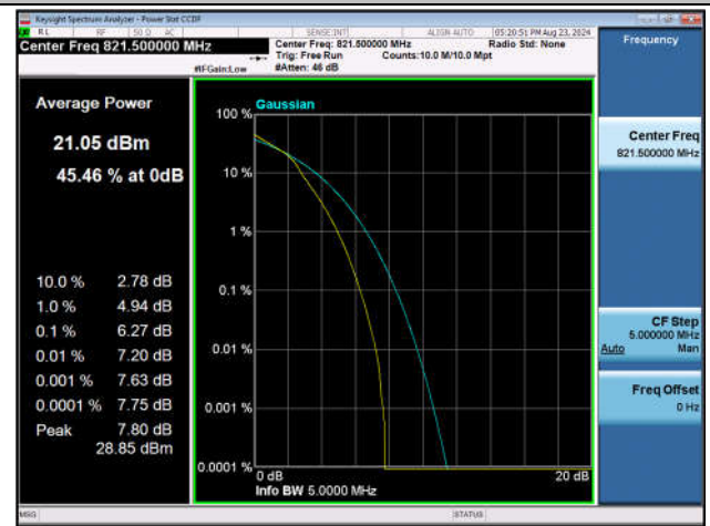
Band26(Part 90)-5MHz-16QAM-26765-25RB#0-PASS
