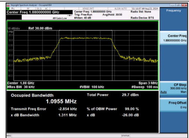
Band2-1.4MHz-16QAM-18900-6RB#0-PASS
