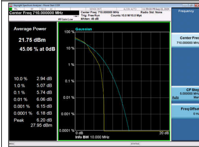
Band17-10MHz-16QAM-23790-1RB#0-PASS
