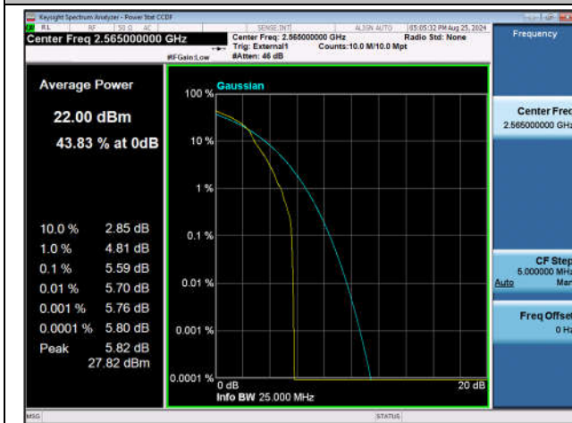
Band41-20MHz-16QAM-40340-1RB#0-PASS
