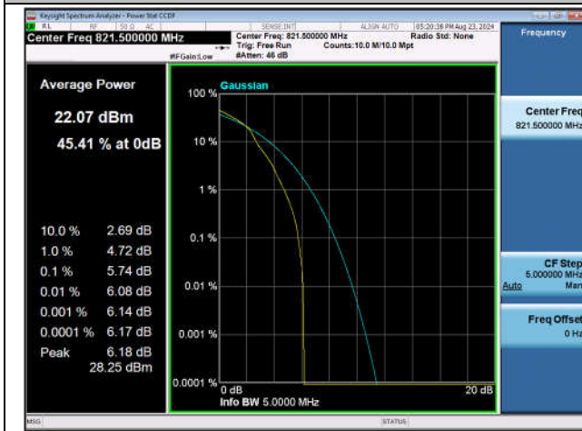
Band26(Part 90)-5MHz-16QAM-26765-1RB#0-PASS
