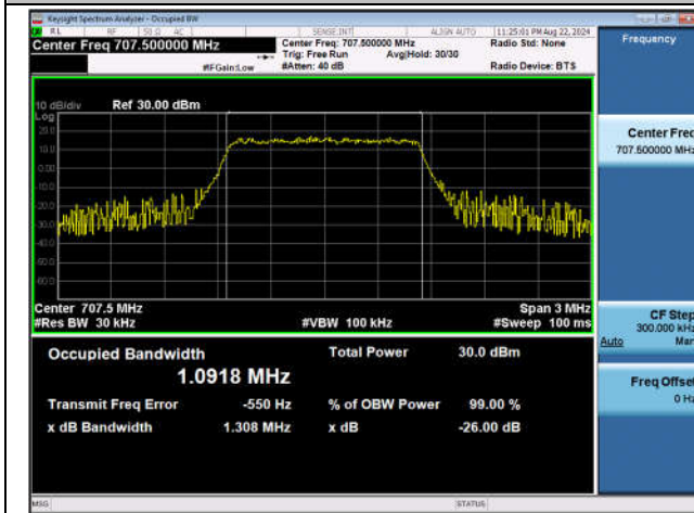
Band12-1.4MHz-QPSK-23095-6RB#0-PASS
