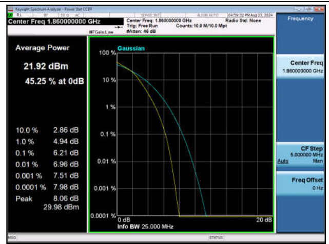
Band25-20MHz-16QAM-26140-100RB#0-PASS
