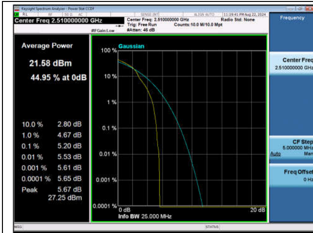
Band7-20MHz-16QAM-20850-1RB#0-PASS
