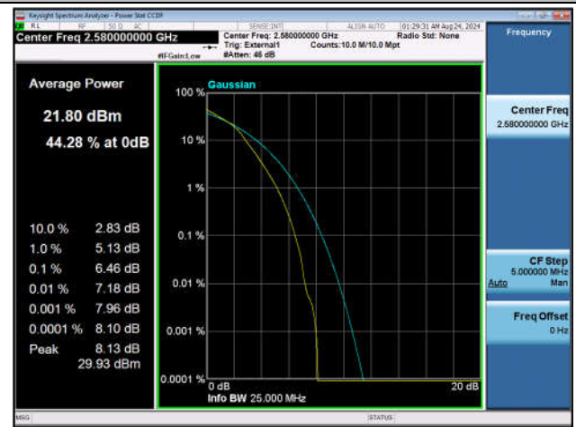
Band38-20MHz-16QAM-37850-100RB#0-PASS
