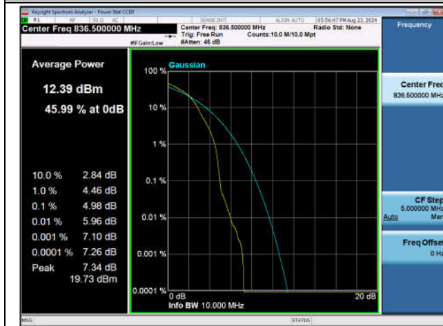
Band26(Part 22)-15MHz-16QAM-26915-1RB#0-PASS
