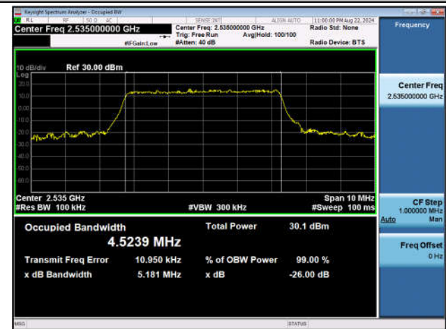
Band7-5MHz-16QAM-21100-25RB#0-PASS
