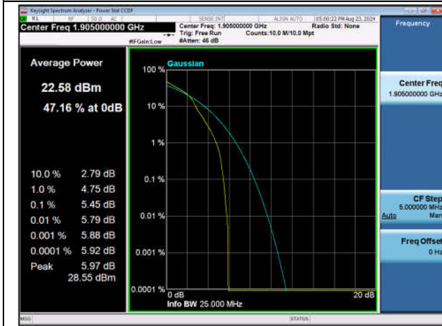
Band25-20MHz-16QAM-26590-1RB#0-PASS
