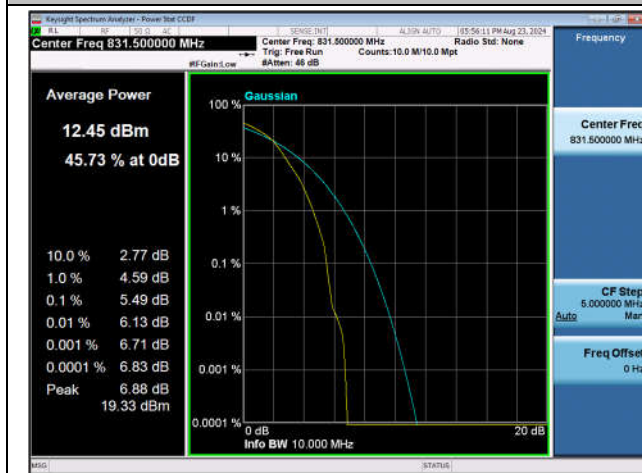
Band26(Part 22)-15MHz-16QAM-26865-1RB#0-PASS
