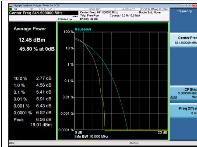
Band26(Part 22)-15MHz-16QAM-26965-1RB#0-PASS
