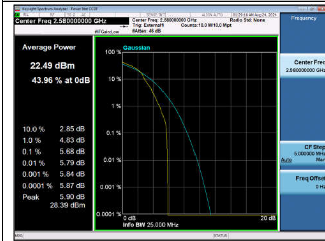
Band38-20MHz-16QAM-37850-1RB#0-PASS
