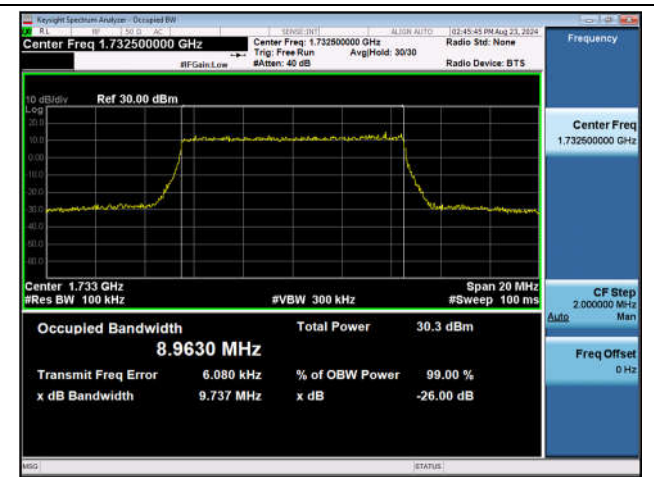
Band4-10MHz-16QAM-20175-50RB#0-PASS
