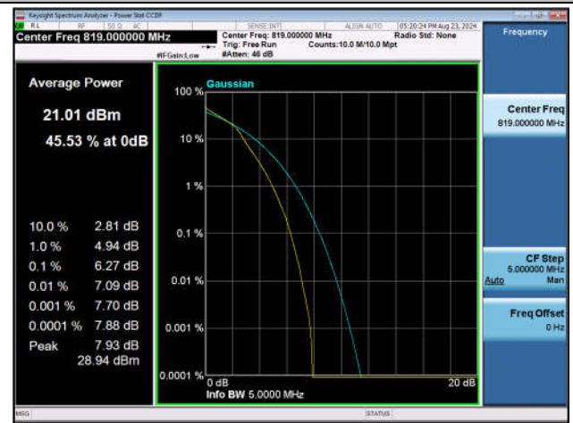
Band26(Part 90)-5MHz-16QAM-26740-25RB#0-PASS
