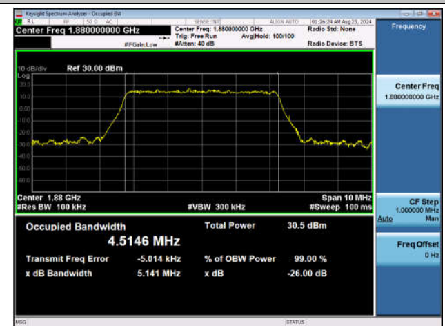
Band2-5MHz-16QAM-18900-25RB#0-PASS
