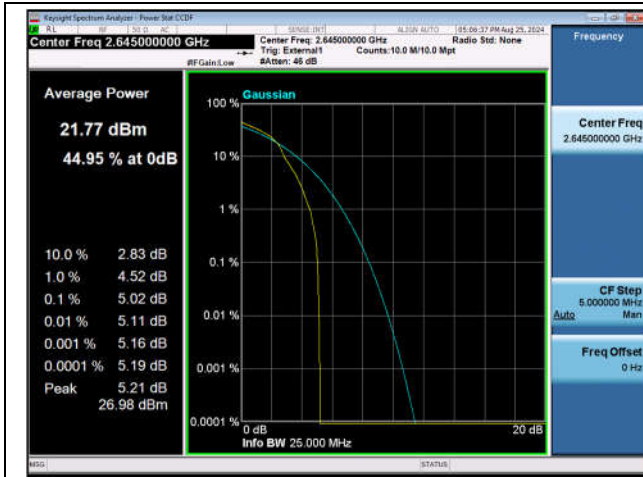
Band41-20MHz-16QAM-41140-1RB#0-PASS
