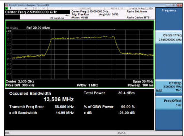
Band7-15MHz-16QAM-21100-75RB#0-PASS
