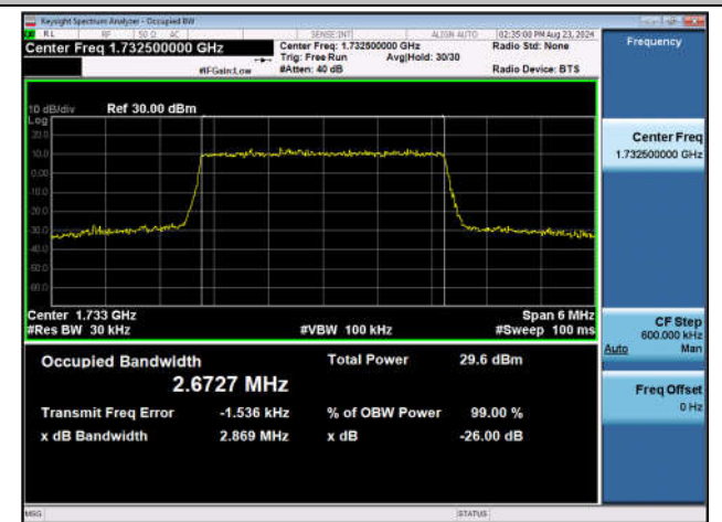
Band4-3MHz-16QAM-20175-15RB#0-PASS
