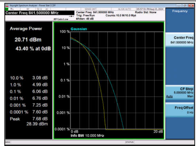
Band26(Part 22)-15MHz-16QAM-26965-75RB#0-PASS
