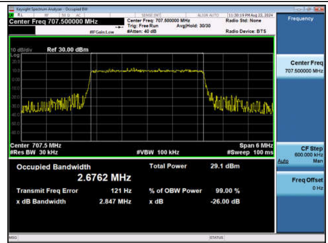
Band12-3MHz-16QAM-23095-15RB#0-PASS
