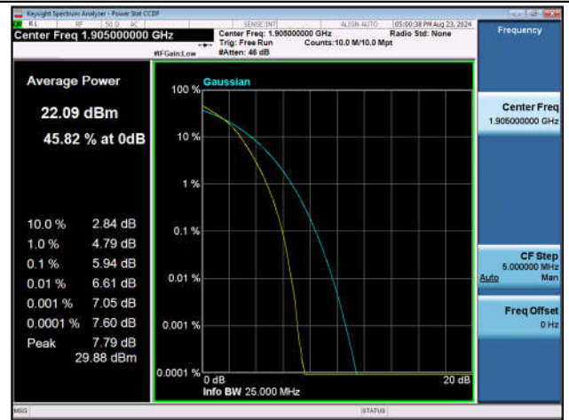
Band25-20MHz-16QAM-26590-100RB#0-PASS
