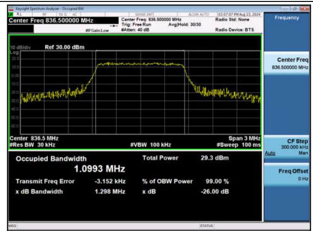
Band5-1.4MHz-16QAM-20525-6RB#0-PASS
