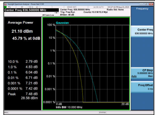
Band5-10MHz-16QAM-20525-50RB#0-PASS
