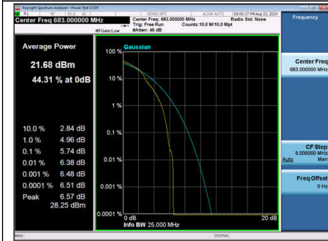
Band71-20MHz-16QAM-133322-1RB#0-PASS
