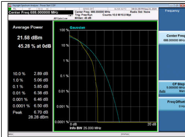
Band71-20MHz-16QAM-133372-1RB#0-PASS
