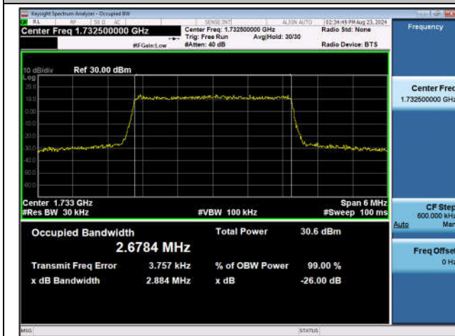
Band4-3MHz-QPSK-20175-15RB#0-PASS
