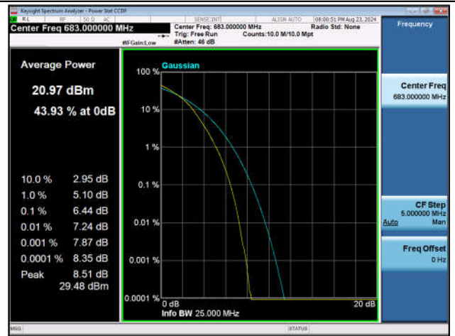
Band71-20MHz-16QAM-133322-100RB#0-PASS
