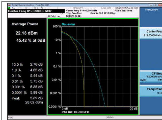
Band26(Part 90)-10MHz-16QAM-26740-1RB#0-PASS
