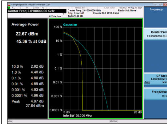
Band38-20MHz-16QAM-38150-1RB#0-PASS
