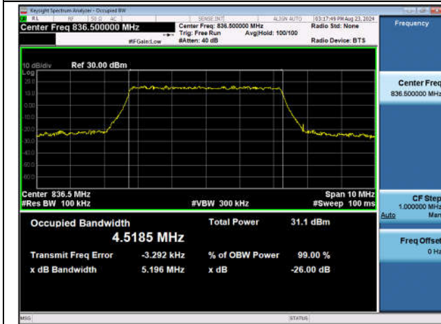
Band5-5MHz-QPSK-20525-25RB#0-PASS
