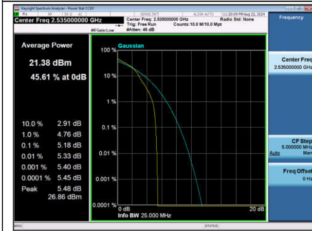
Band7-20MHz-16QAM-21100-1RB#0-PASS
