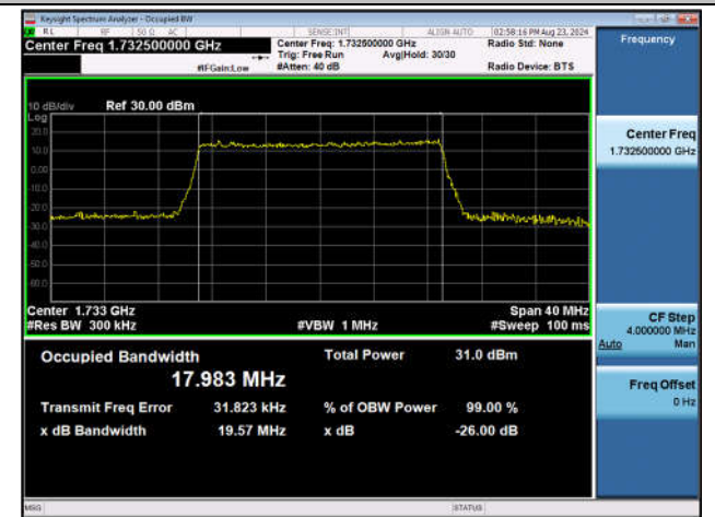
Band4-20MHz-16QAM-20175-100RB#0-PASS
