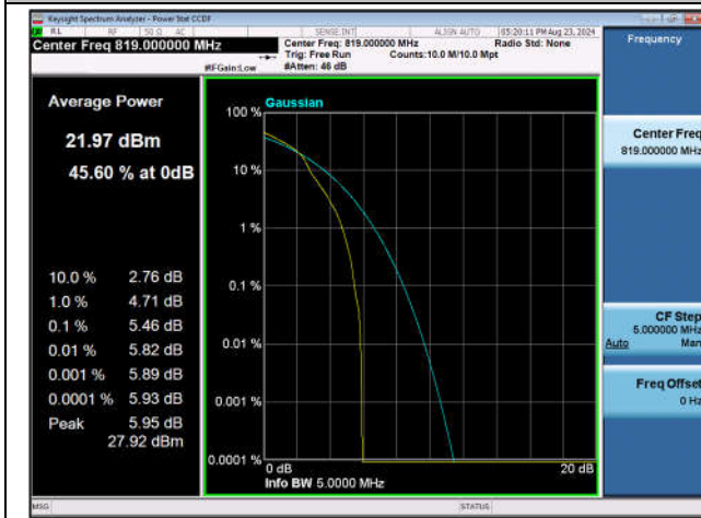
Band26(Part 90)-5MHz-16QAM-26740-1RB#0-PASS
