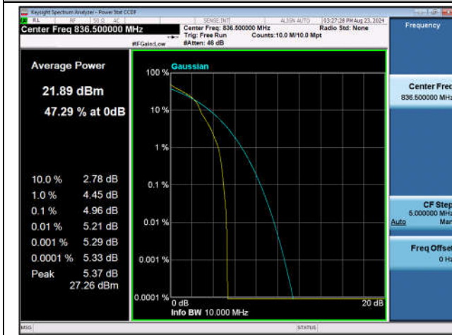
Band5-10MHz-16QAM-20525-1RB#0-PASS
