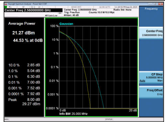
Band7-20MHz-16QAM-21350-100RB#0-PASS
