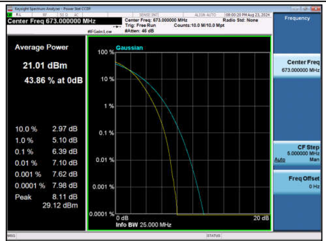
Band71-20MHz-16QAM-133222-100RB#0-PASS
