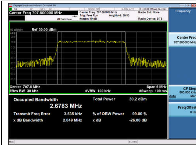
Band12-3MHz-QPSK-23095-15RB#0-PASS
