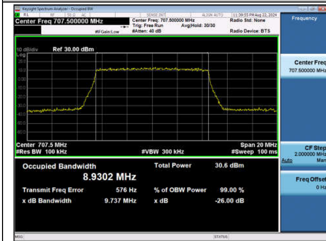
Band12-10MHz-QPSK-23095-50RB#0-PASS
