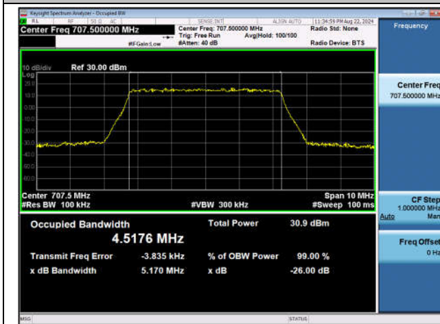
Band12-5MHz-QPSK-23095-25RB#0-PASS
