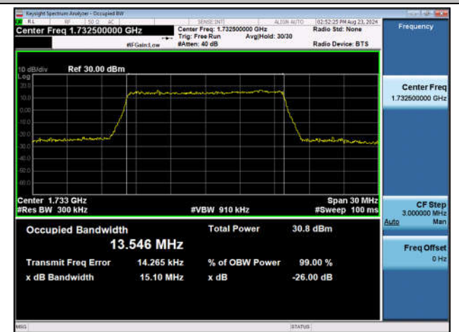
Band4-15MHz-16QAM-20175-75RB#0-PASS
