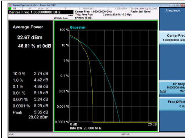
Band25-20MHz-16QAM-26140-1RB#0-PASS
