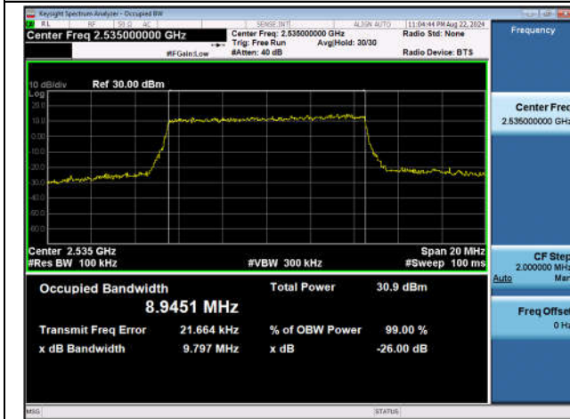
Band7-10MHz-QPSK-21100-50RB#0-PASS
