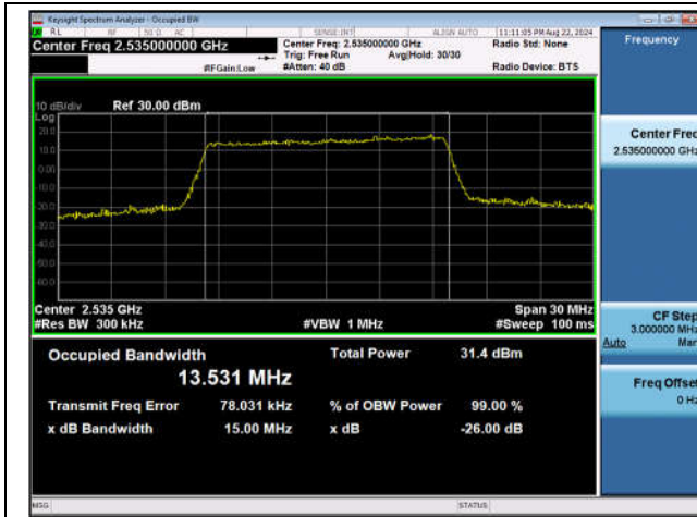
Band7-15MHz-QPSK-21100-75RB#0-PASS
