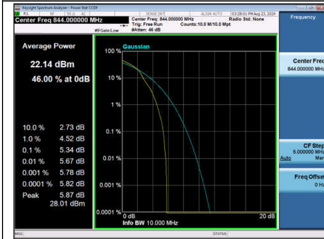
Band5-10MHz-16QAM-20600-1RB#0-PASS
