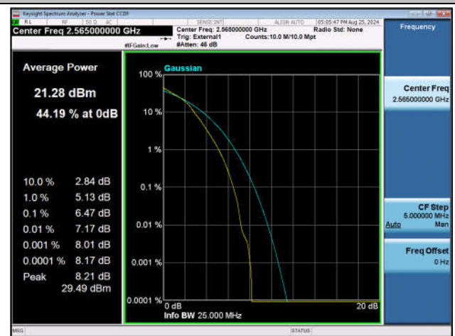
Band41-20MHz-16QAM-40340-100RB#0-PASS
