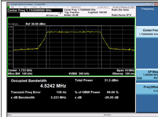
Band4-5MHz-QPSK-20175-25RB#0-PASS
