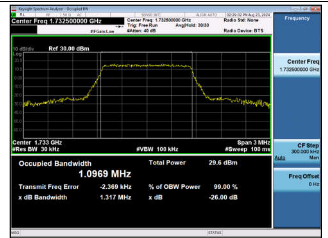
Band4-1.4MHz-16QAM-20175-6RB#0-PASS
