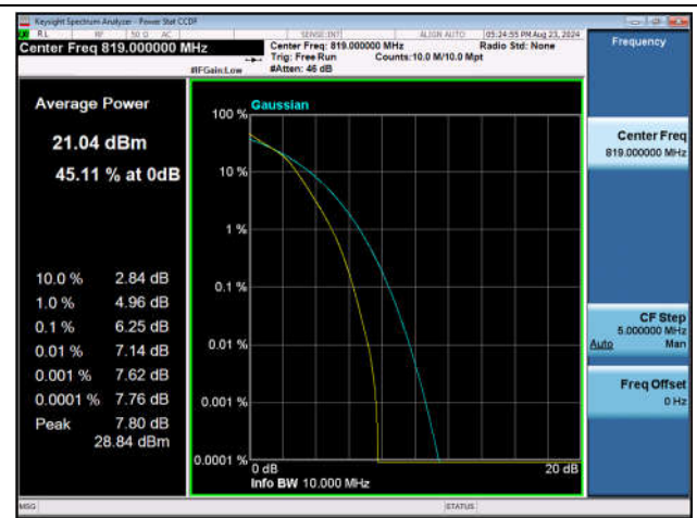
Band26(Part 90)-10MHz-16QAM-26740-50RB#0-PASS
