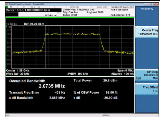
Band2-3MHz-16QAM-18900-15RB#0-PASS
