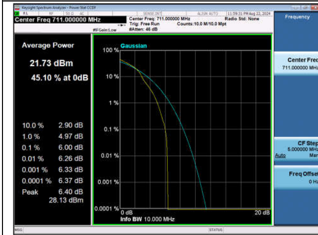
Band17-10MHz-16QAM-23800-1RB#0-PASS
