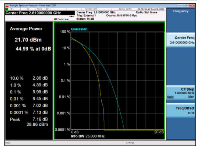
Band38-20MHz-16QAM-38150-100RB#0-PASS
