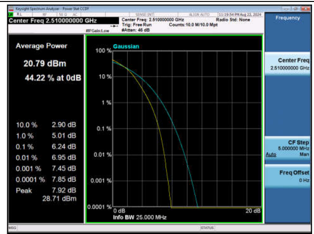
Band7-20MHz-16QAM-20850-100RB#0-PASS
