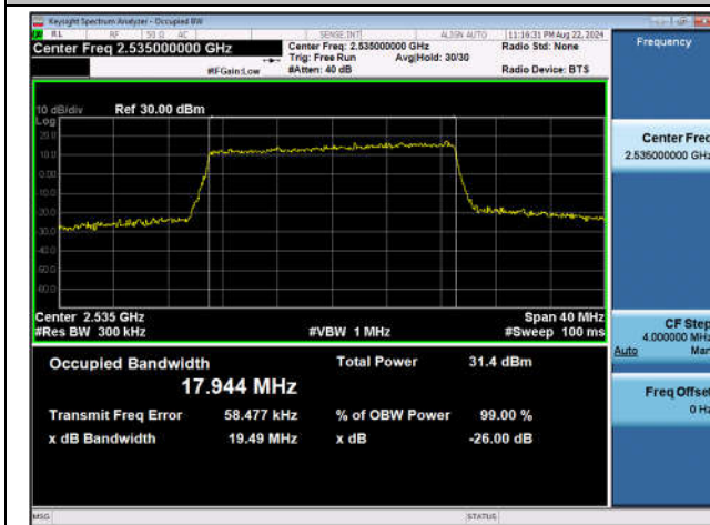
Band7-20MHz-QPSK-21100-100RB#0-PASS
