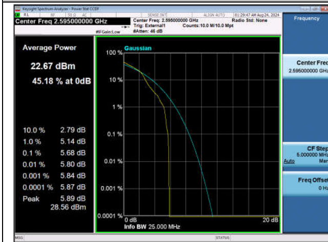
Band38-20MHz-16QAM-38000-1RB#0-PASS
