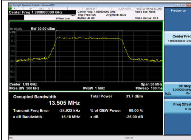
Band2-15MHz-QPSK-18900-75RB#0-PASS
