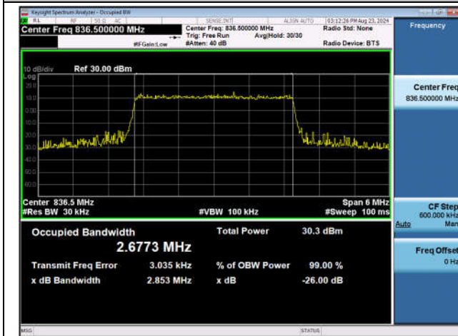
Band5-3MHz-QPSK-20525-15RB#0-PASS
