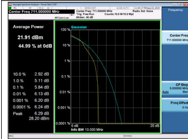
Band12-10MHz-16QAM-23130-1RB#0-PASS
