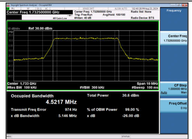
Band4-5MHz-16QAM-20175-25RB#0-PASS
