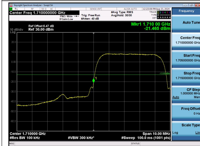
Band4-1312-PASS
