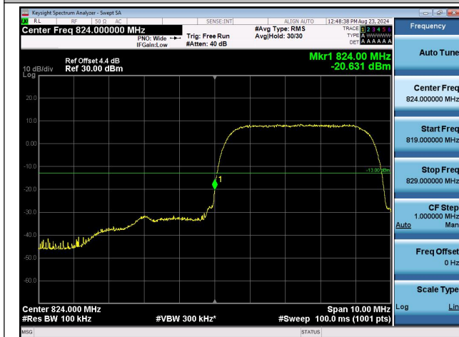
Band5-4132-PASS
