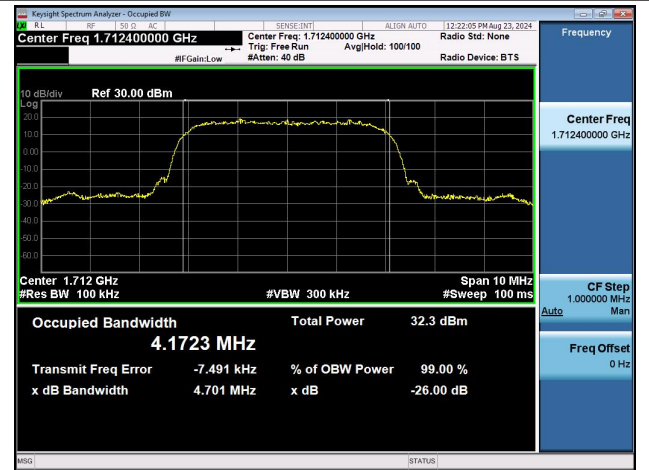
Band4-1312-PASS
