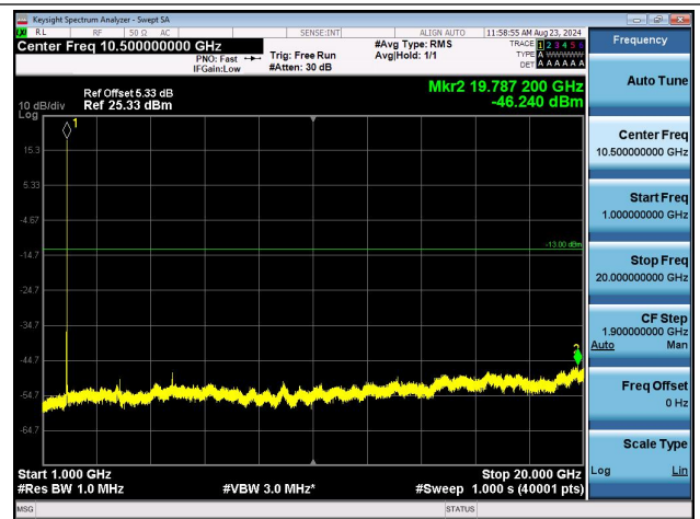
Band2-9262-1000~20000MHz-PASS
