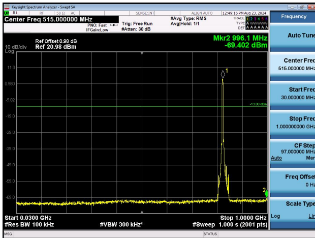
Band5-4132-30~1000MHz-PASS
