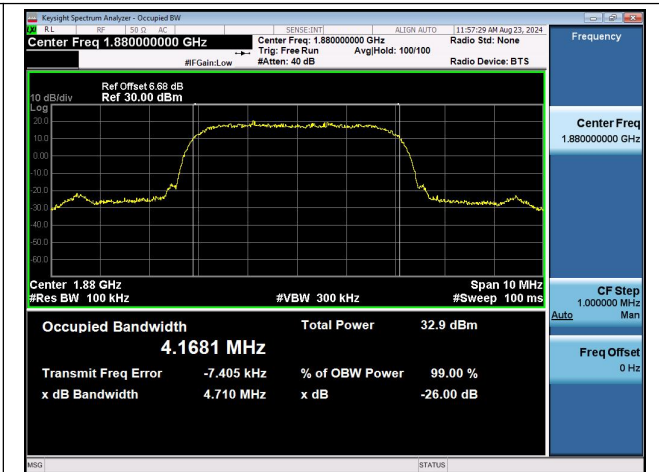
Band2-9400-PASS
