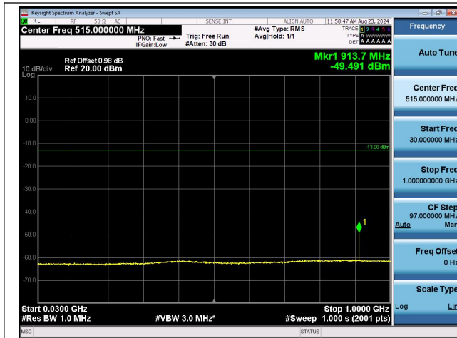
Band2-9262-30~1000MHz-PASS
