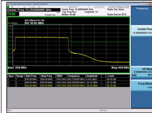
Band5_10MHz_QPSK_20600_50RB#0
