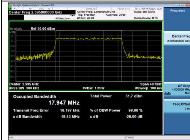
Band38-20MHz-QPSK-38000-100RB#0-PASS
