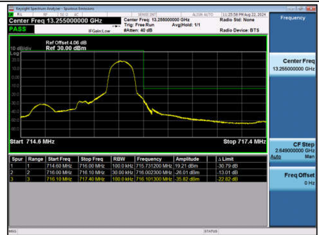
Band12_1.4MHz_QPSK_23173_1RB#5
