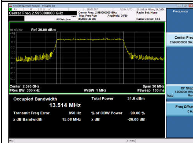
Band38-15MHz-QPSK-38000-75RB#0-PASS
