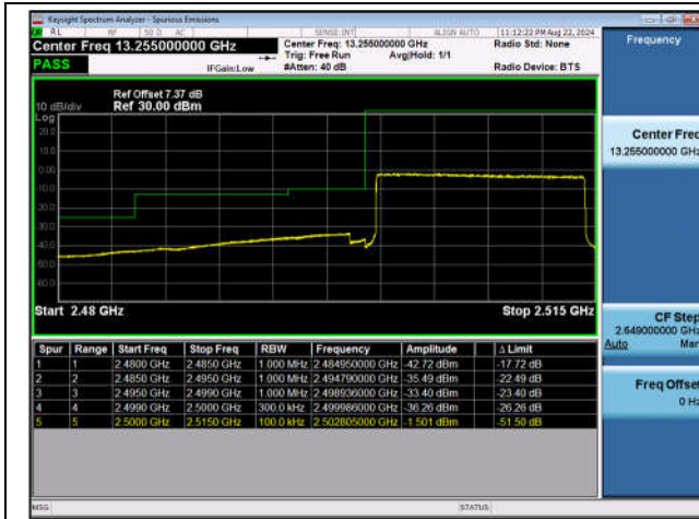
Band7_15MHz_QPSK_20825_75RB#0
