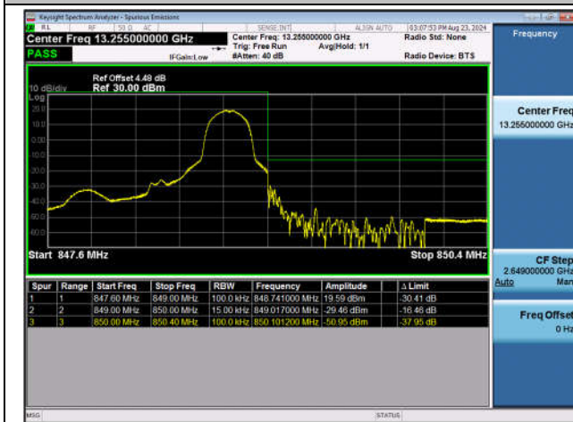
Band5_1.4MHz_QPSK_20643_1RB#5
