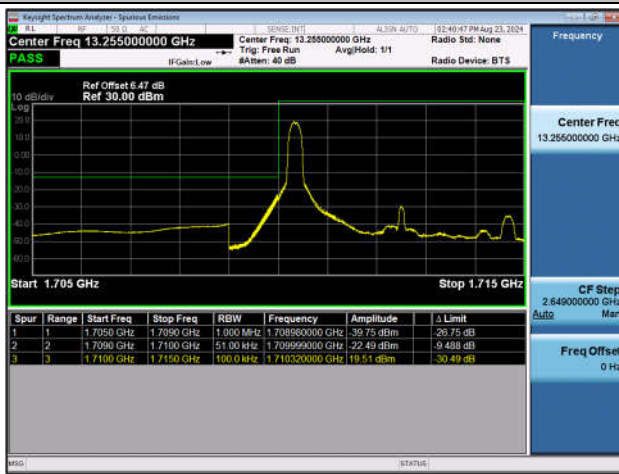
Band4_5MHz_QPSK_19975_1RB#0
