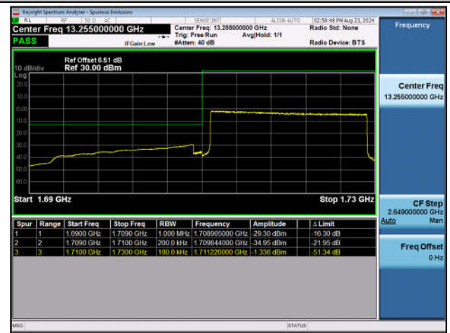
Band4_20MHz_QPSK_20050_100RB#0
