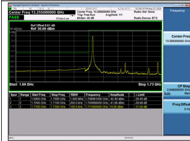
Band4_20MHz_QPSK_20050_1RB#0
