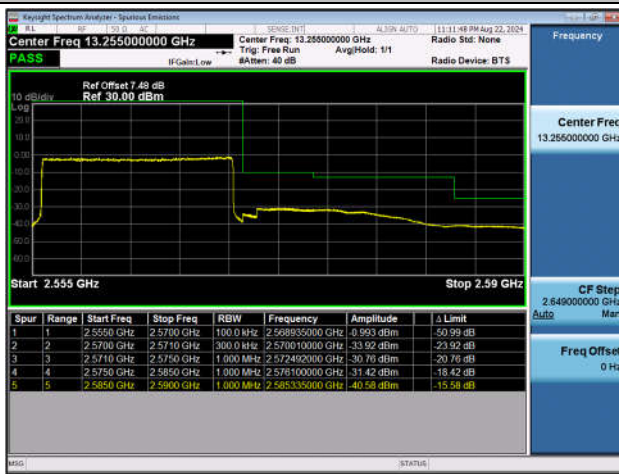
Band7_15MHz_QPSK_21375_75RB#0
