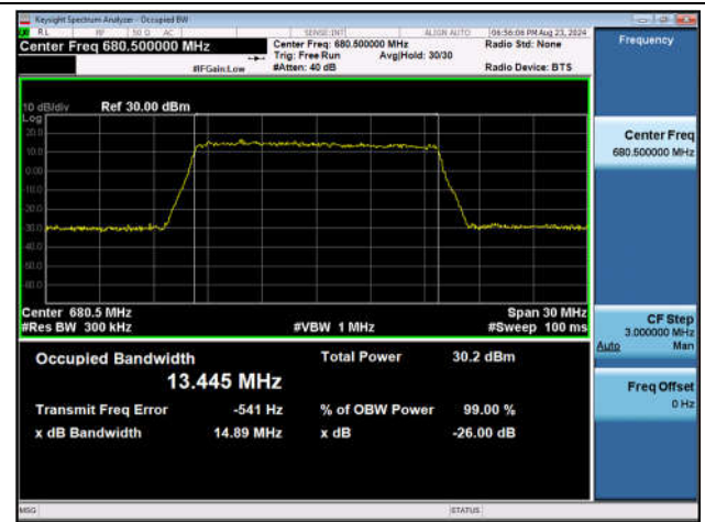
Band71-15MHz-16QAM-133297-75RB#0-PASS
