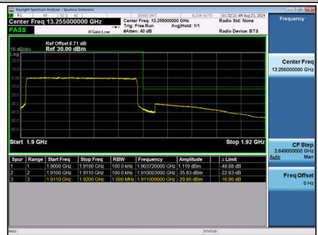
Band2_10MHz_QPSK_19150_50RB#0
