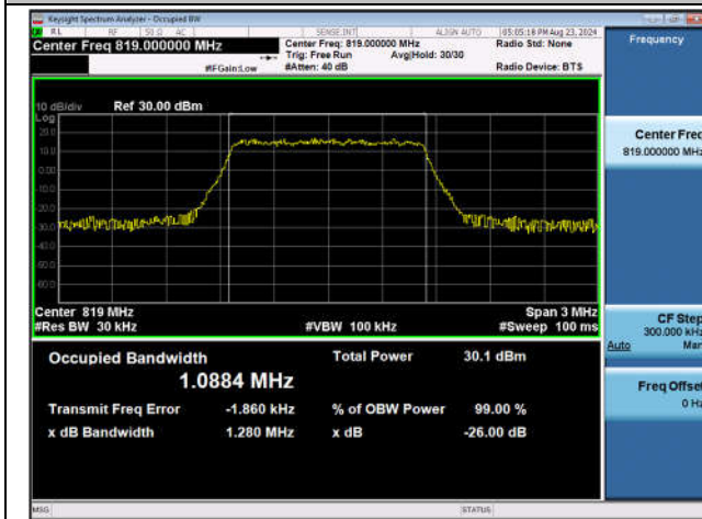
Band26(Part 90)-1.4MHz-QPSK-26740-6RB#0-PASS
