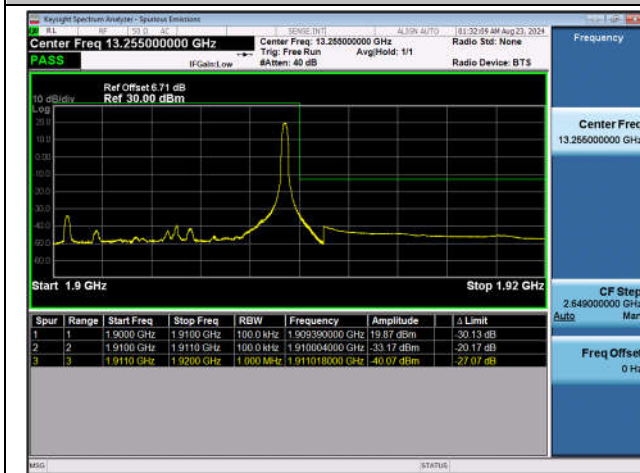
Band2_10MHz_QPSK_19150_1RB#49
