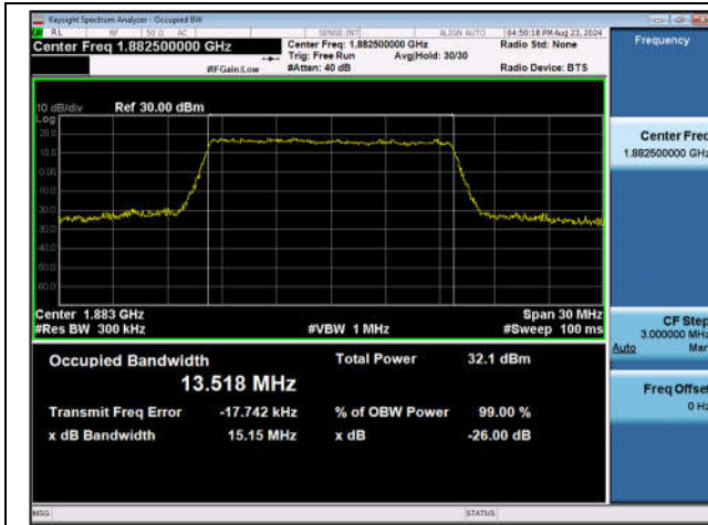
Band25-15MHz-QPSK-26365-75RB#0-PASS
