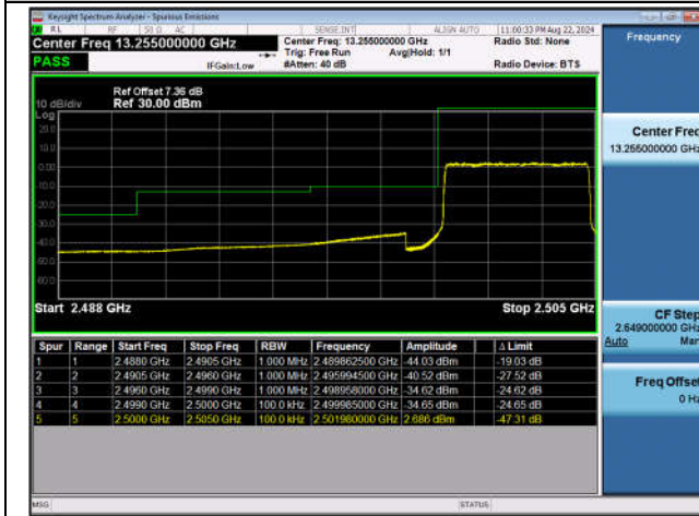
Band7_5MHz_QPSK_20775_25RB#0
