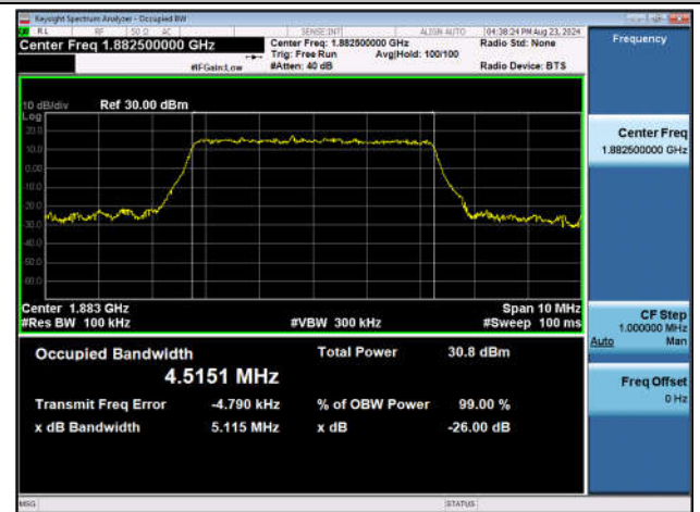
Band25-5MHz-16QAM-26365-25RB#0-PASS
