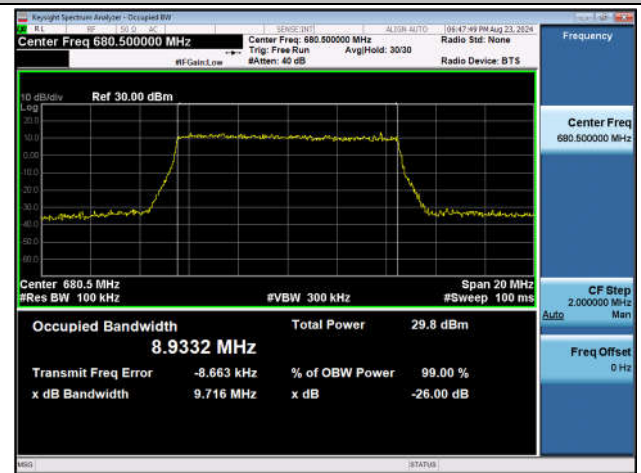
Band71-10MHz-16QAM-133297-50RB#0-PASS
