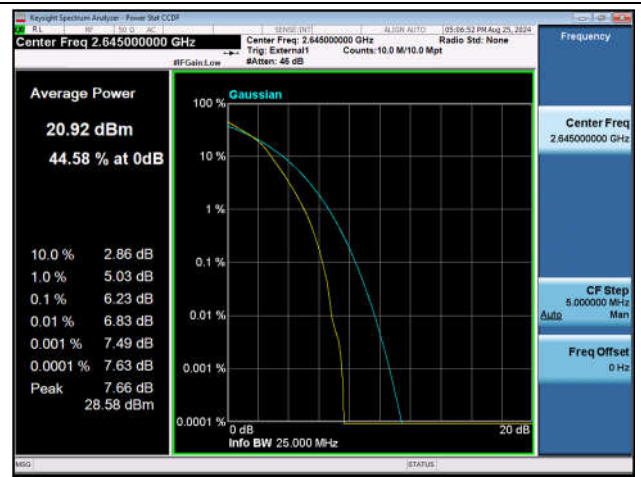
Band41-20MHz-16QAM-41140-100RB#0-PASS
