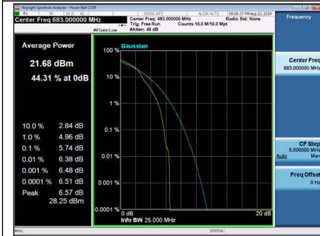
Band71-20MHz-16QAM-133322-1RB#0-PASS
