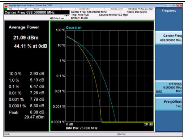
Band71-20MHz-16QAM-133372-100RB#0-PASS
