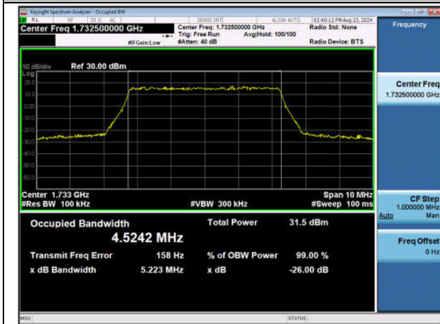
Band4-5MHz-QPSK-20175-25RB#0-PASS
