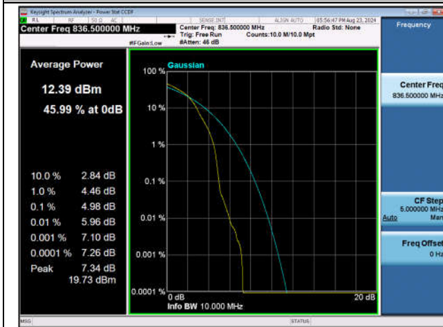
Band26(Part 22)-15MHz-16QAM-26915-1RB#0-PASS
