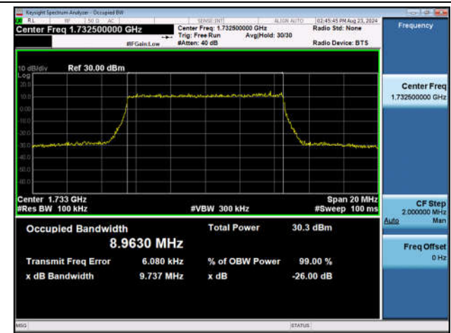
Band4-10MHz-16QAM-20175-50RB#0-PASS
