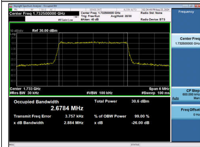
Band4-3MHz-QPSK-20175-15RB#0-PASS
