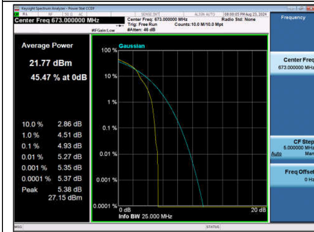
Band71-20MHz-16QAM-133222-1RB#0-PASS
