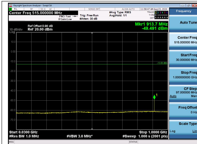
Band2-9262-30~1000MHz-PASS
