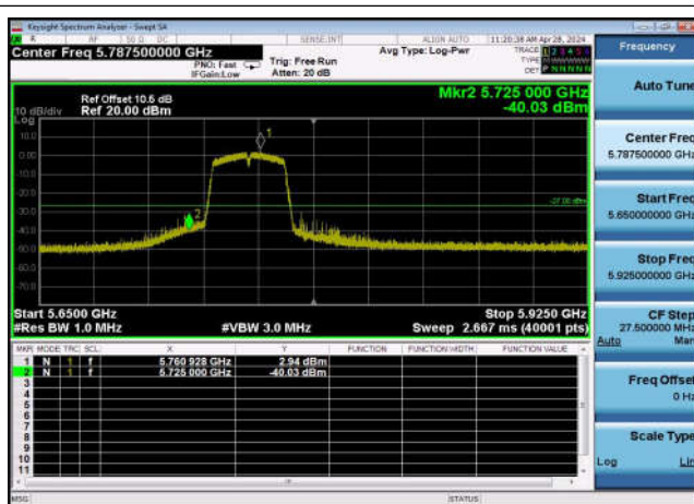
U-NII-3 ,Plot 1,Band Edge-802.11ac(80 MHz),5775MHz,Ant1
