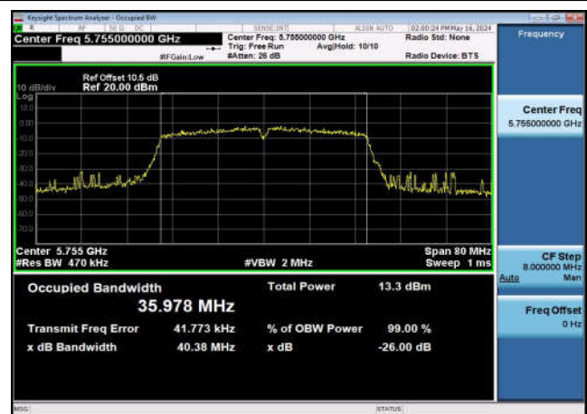
U-NII-3 99%&26dB Bandwidth-802.11n(40MHz) ,5755MHz,Ant1
