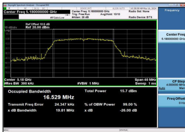
U-NII-1 99%&26dB Bandwidth-802.11a(20MHz) ,5180MHz,Ant1
