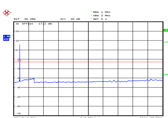
LTE Band 4 1.4MHz CH- Middle 1GHz ~20GHz
