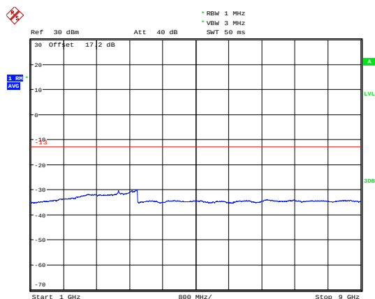
LTE Band 85 5MHz CH-Low 1GHz~9GHz
