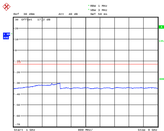
LTE Band 85 5MHz CH-Middle 1GHz~9GHz
