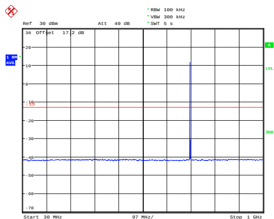
LTE Band 85 5MHz CH-Middle 30MHz~1GHz
