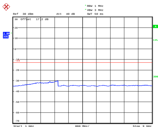
LTE Band 85 5MHz CH-High 1GHz~9GHz
