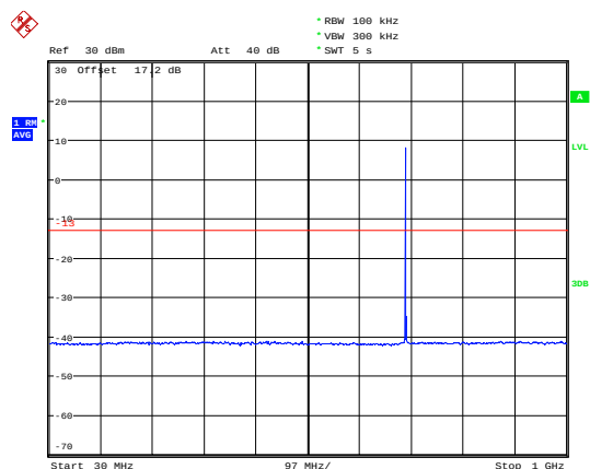
LTE Band 85 5MHz CH-Low 30MHz~1GHz
