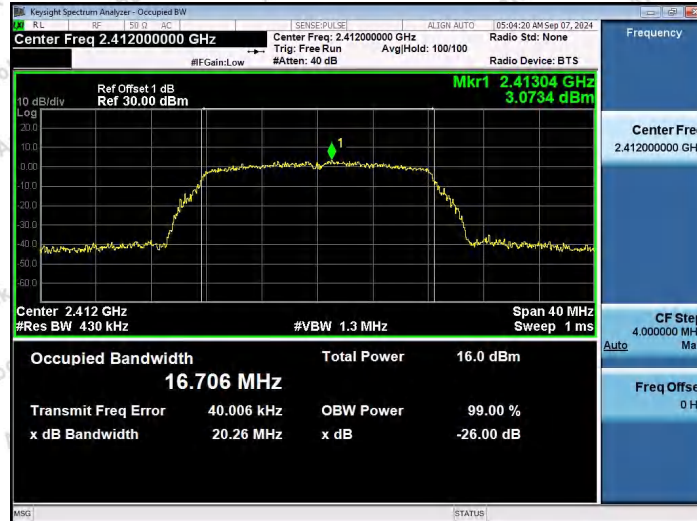
11G-Ant1-2412
