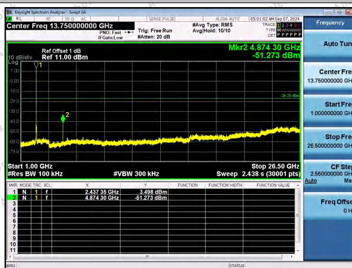
11B-Ant1-2437-1000~26500-PASS
