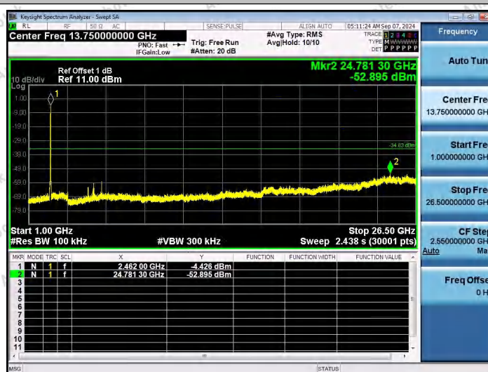
11G-Ant1-2462-1000~26500-PASS
