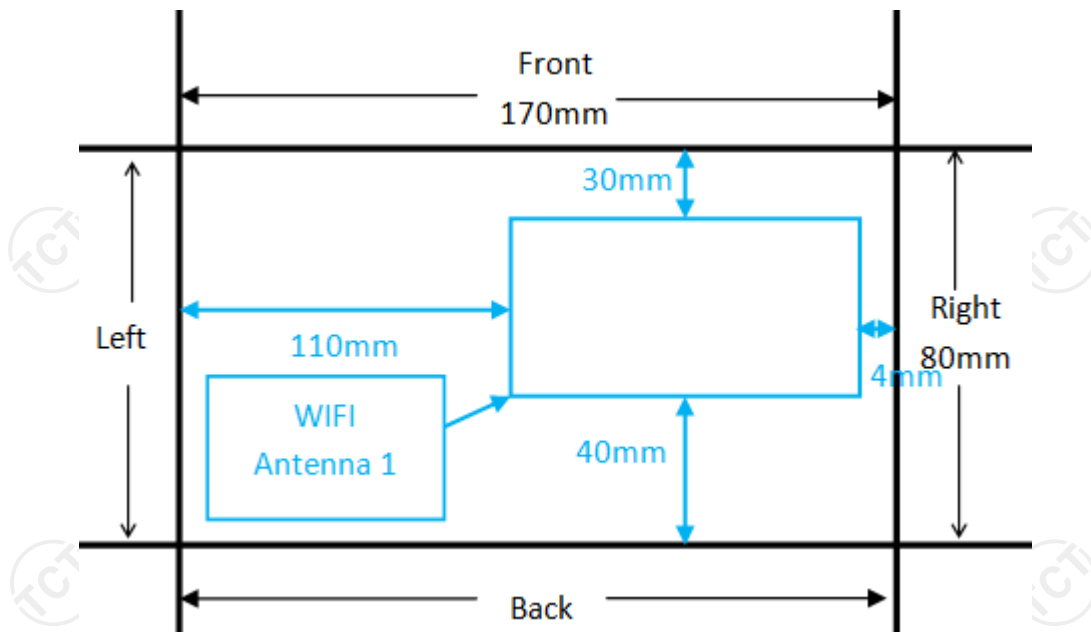
Antenna Configuration 2
