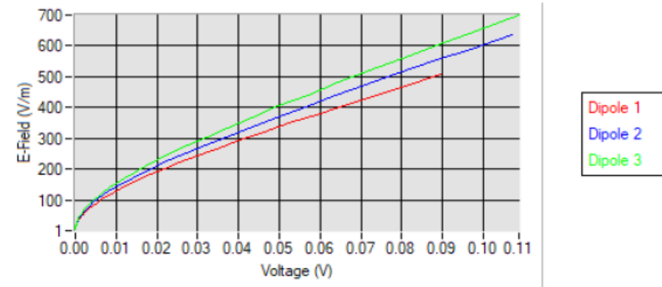
Calibration curves
