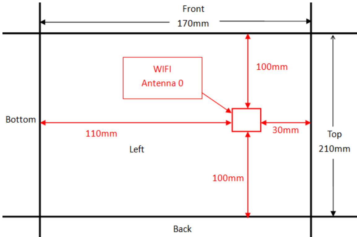
Antenna Configuration 1
