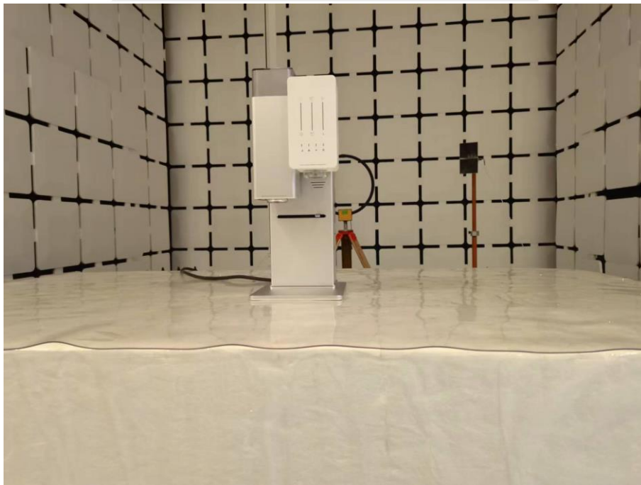
DXX Loop antenna
