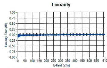
Linearity: +/- 1.99% (+/-0.09dB)
