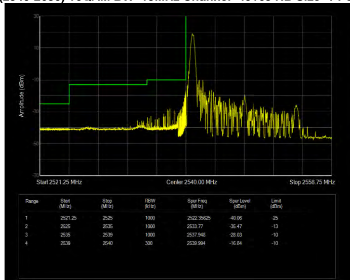
Band41(2540-2650) 16QAM BW=15MHz Channel=40165 RB Size=1 Position=#0
