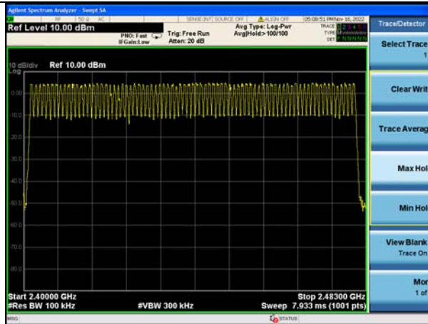
GFSK Modulation
