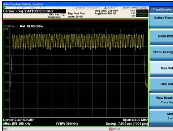
8DPSK Modulation
