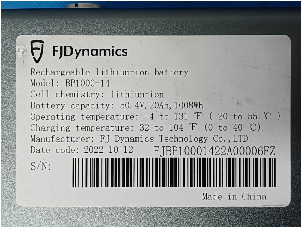
LABEL VIEW OF BATTERY
