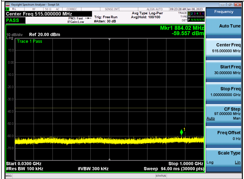
Test_Graph_802.11ax80_ANT2_5775_MCS9_Frequency Band1
