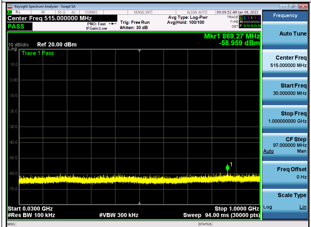
Test_Graph_802.11ax80_ANT1_5775_MCS9_Frequency Band1
