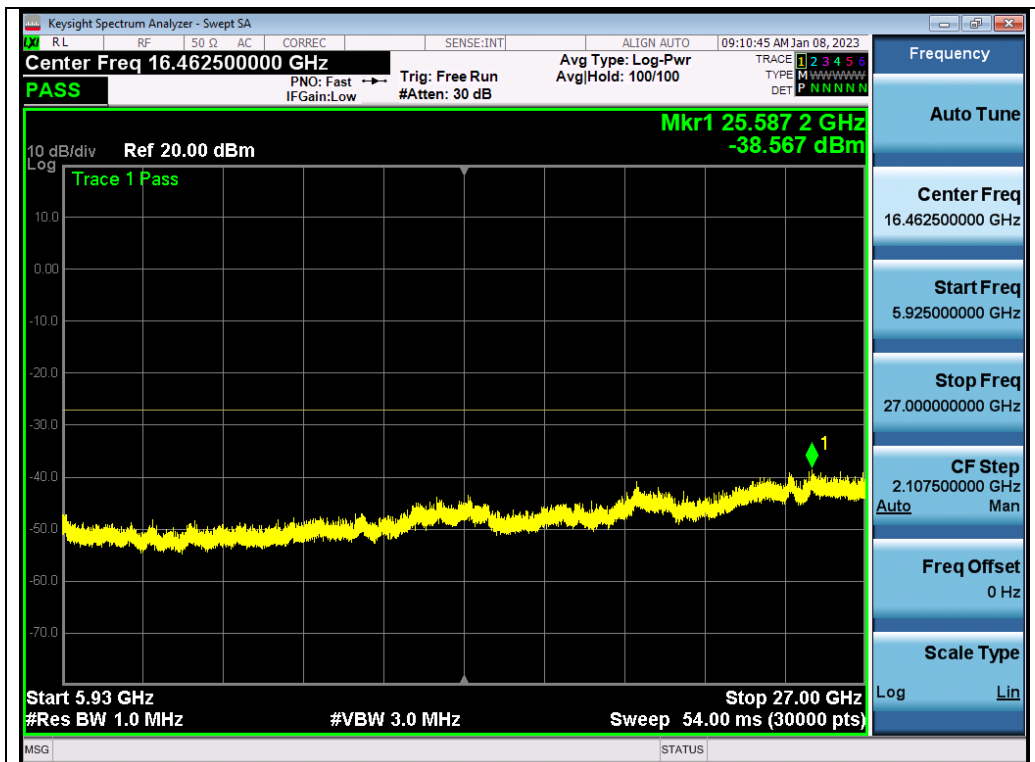
Test_Graph_802.11ax80_ANT1_5775_MCS9_Frequency Band4
