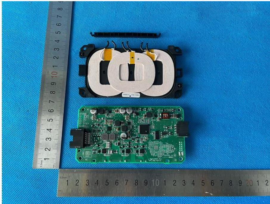
Internal view of main unit
