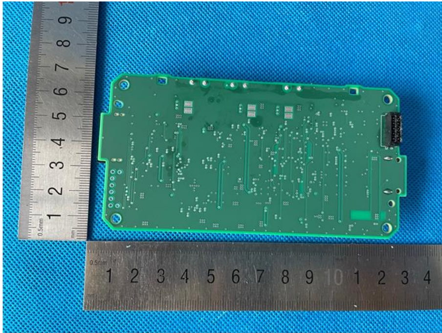
Bottom of top main board
