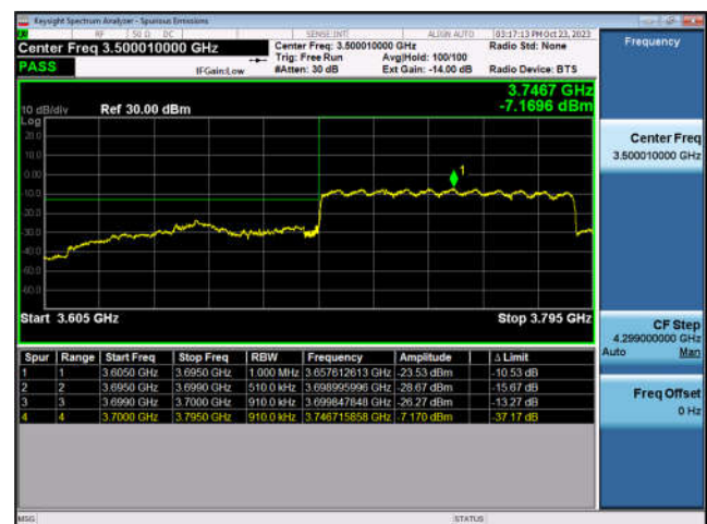
N77_90MHz_DFT-s-OFDM_PI/2-BPSK_Edge_ Outer_Full_Low_CH
