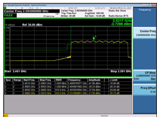
N41_90MHz_DFT-s-OFDM_PI/2-BPSK_Edge_ Outer_Full_Low_CH
