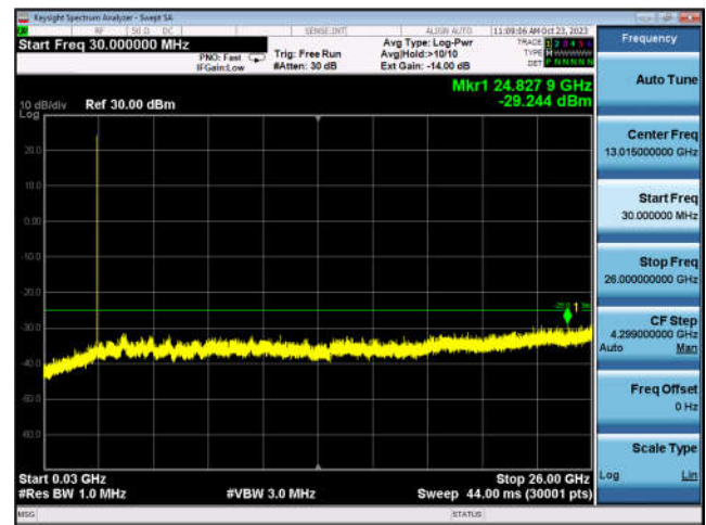
N26_Part 22_20MHz_DFT-s-OFDM_BPSK_ Edge_1RB_Left_Low_CH
