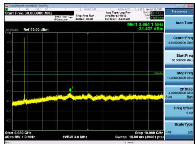
N5_20MHz_DFT-s-OFDM_BPSK_ Edge_1RB_Left_High_CH
