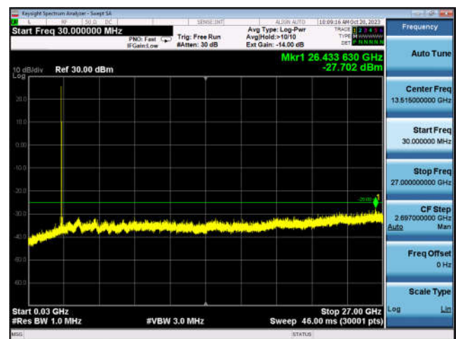
N41_100MHz_DFT-s-OFDM_BPSK_ Edge_1RB_Left_Mid_CH
