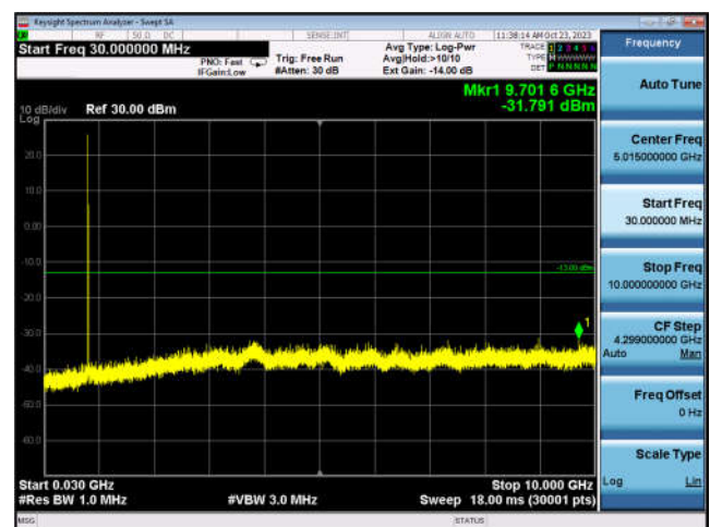
N26_Part 22_20MHz_DFT-s-OFDM_BPSK_ Edge_1RB_Left_High_CH
