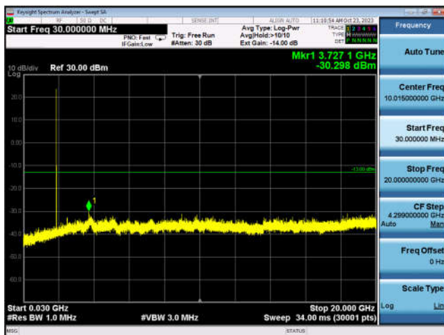
N5_20MHz_DFT-s-OFDM_BPSK_ Edge_1RB_Left_Mid_CH
