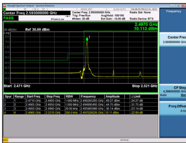
N41_20MHz_DFT-s-OFDM_PI/2-BPSK_Edge_ 1RB_Right_High_CH
