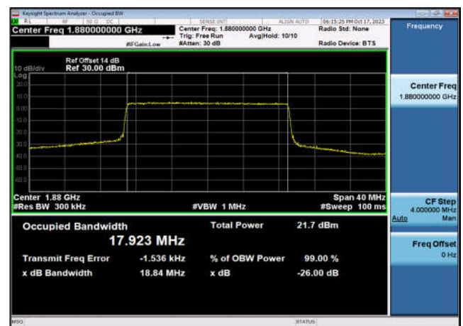
FDD02_MidRange_3_1880_QPSK
