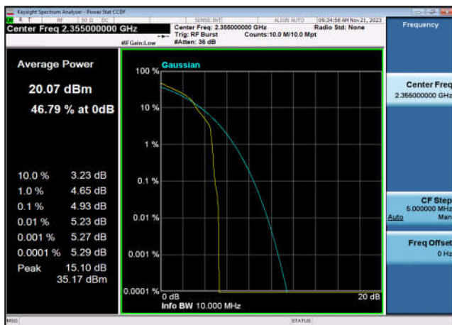
TDD40B_MidRange_10MHz_2355_OneRB_high_Q16
