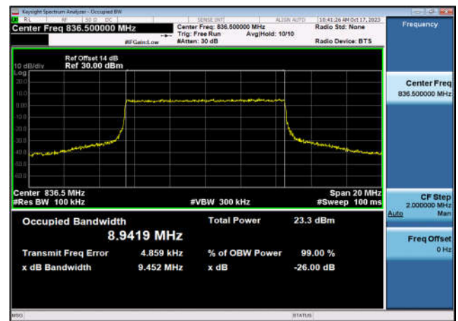
FDD26_Part 22_MidRange_15_836.5_QPSK
