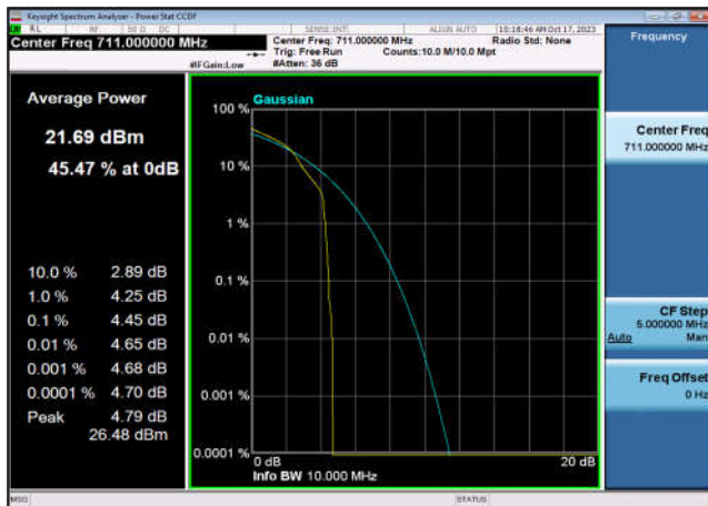
FDD17_HighRange_10MHz_711_OneRB _high_Q16
