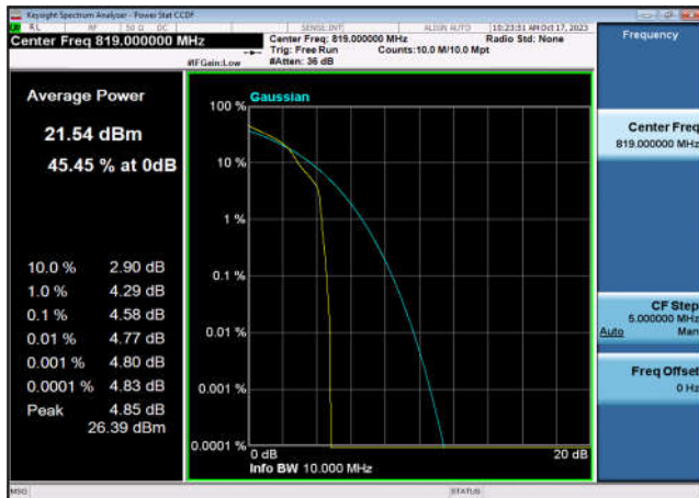
TDD40A_MidRange_10MHz_2310_OneRB_high_Q16
