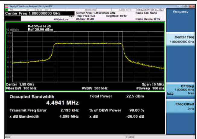
FDD02_MidRange_5_1880_QPSK
