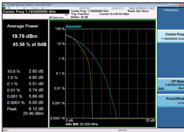
FDD66_MidRange_20MHz_1745_fullIRB _Q16
