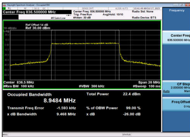
FDD26_Part 22_MidRange_15_836.5_Q16
