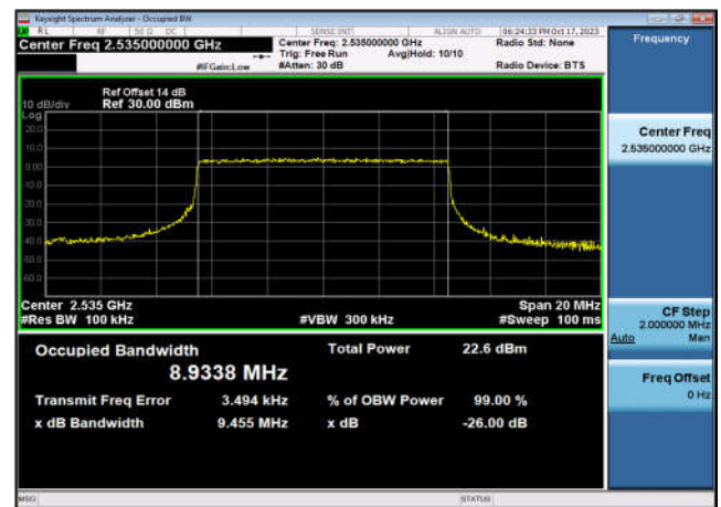
FDD07_MidRange_15_2535_QPSK
