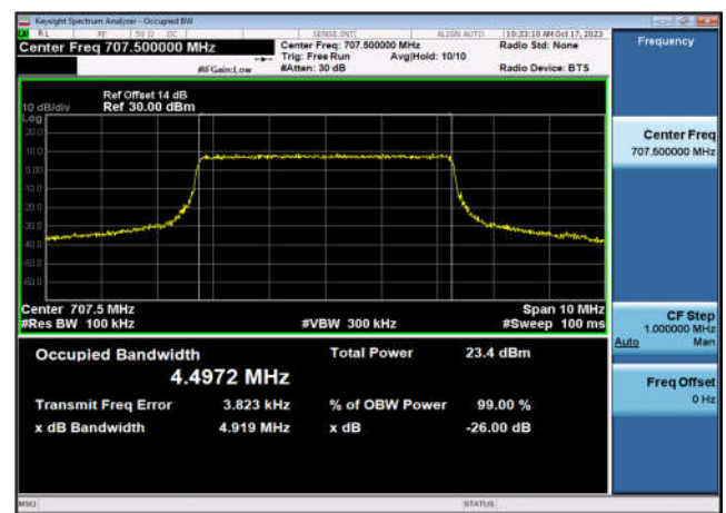
FDD12_MidRange_5_707.5_QPSK
