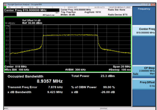
FDD26_Part 90_MidRange_10_819_QPSK
