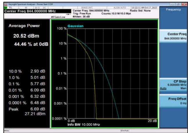
FDD26_Part 22_HighRange_10MHz_844_fullRB_Q16
