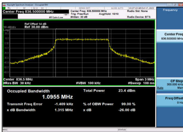
FDD05_MidRange_10_836.5_Q16
