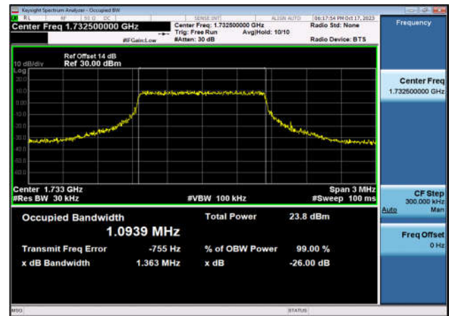
FDD04_MidRange_10_1732.5_QPSK
