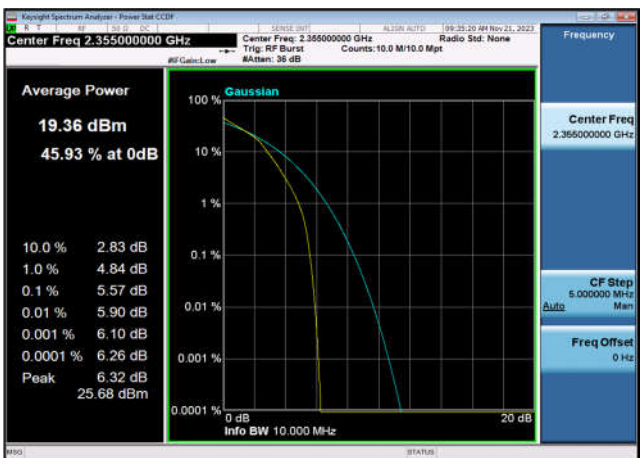
TDD40B_MidRange_10MHz_2355_fullRB_Q16
