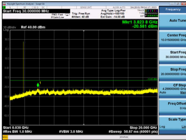
PCS 1900-661, 30MHz ~20GHz
