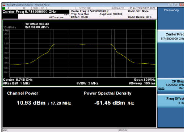
U-NII-3 Output Power-802.11a(20MHz) ,5745MHz,Ant7
