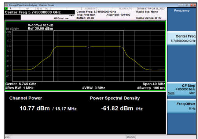
U-NII-3 Output Power-802.11ac(20MHz) ,5745MHz,Ant6
