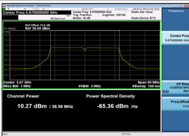
U-NII-2c Output Power-802.11n(40MHz) ,5670MHz,Ant7
