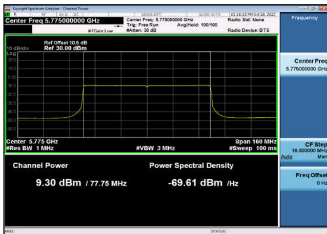
U-NII-3 Output Power-802.11ax(80MHz) ,5775MHz,Ant7
