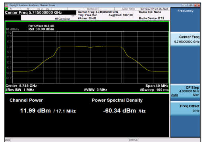
U-NII-3 Output Power-802.11a(20MHz) ,5745MHz,Ant6
