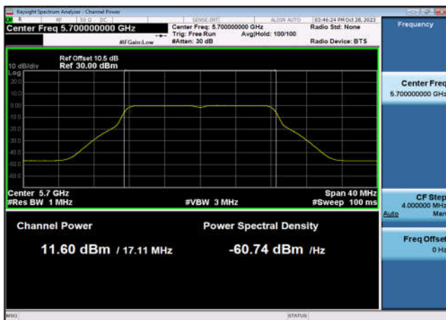
U-NII-2c Output Power-802.11a(20MHz) ,5700MHz,Ant7
