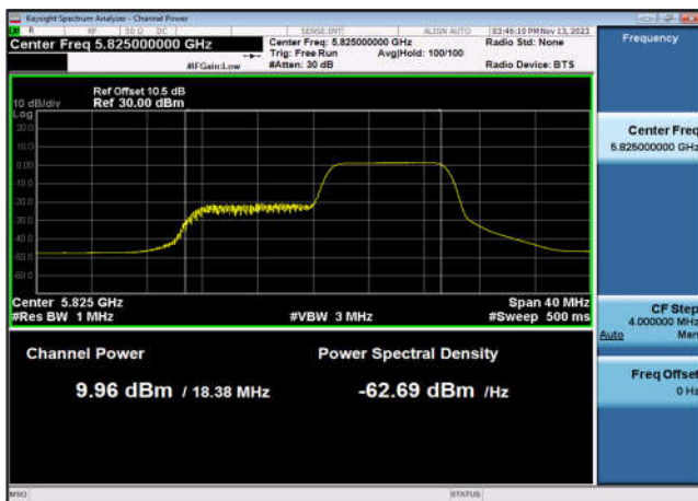
U-NII-3 Output Power-802.11ax(20MHz _RU106_2),5825MHz,Ant7
