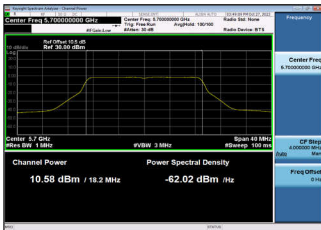
U-NII-2c Output Power-802.11n(20MHz) ,5700MHz,Ant7
