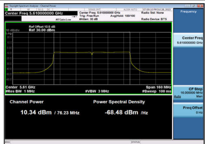
U-NII-2c Output Power-802.11ac(80MHz) ,5610MHz,Ant6
