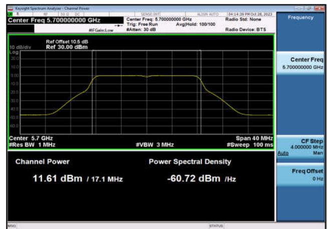
U-NII-2c Output Power-802.11a(20MHz) ,5700MHz,Ant6
