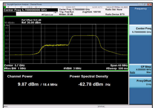
U-NII-2c Output Power-802.11ax(20MHz _RU106_2),5700MHz,Ant6
