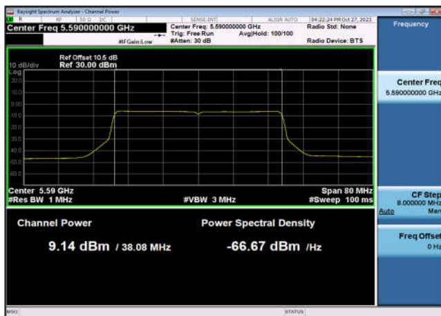
U-NII-2c Output Power-802.11ax(40MHz) ,5590MHz,Ant7
