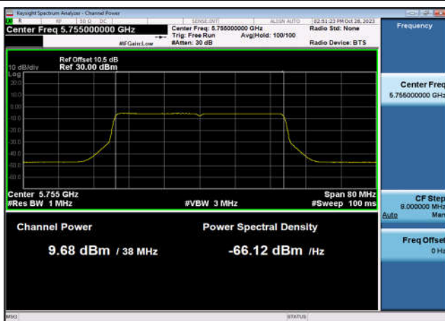
U-NII-3 Output Power-802.11ax(40MHz) ,5755MHz,Ant7
