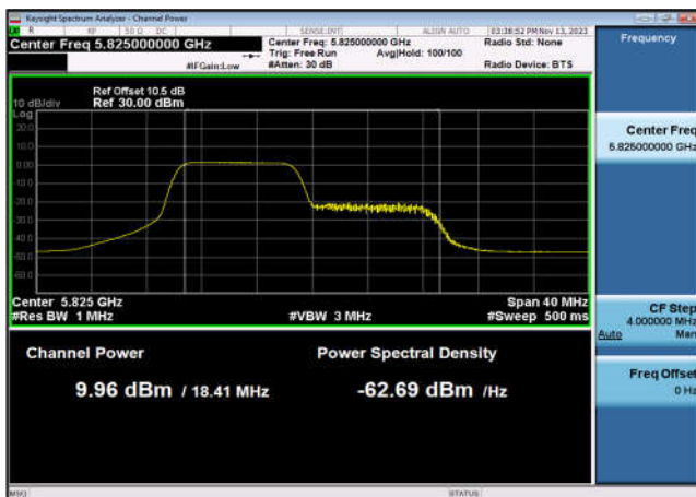
U-NII-3 Output Power-802.11ax(20MHz _RU106_1),5825MHz,Ant7
