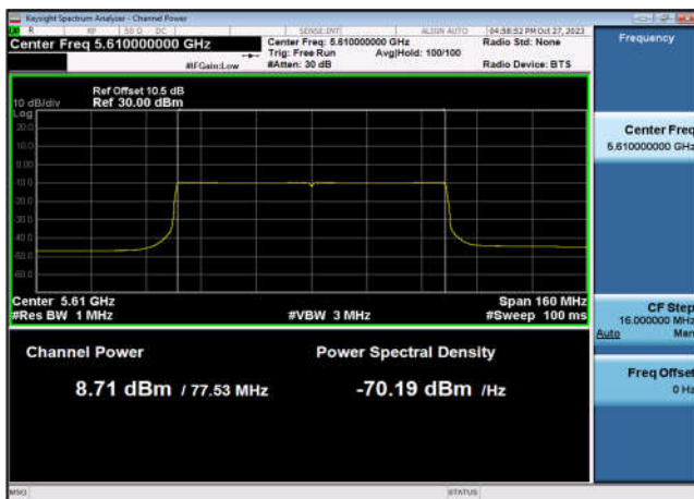
U-NII-2c Output Power-802.11ax(80MHz) ,5610MHz,Ant7
