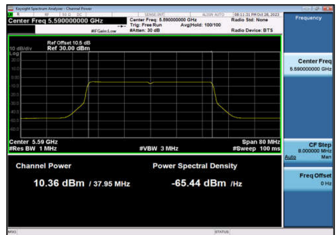
U-NII-2c Output Power-802.11ax(40MHz) ,5590MHz,Ant6
