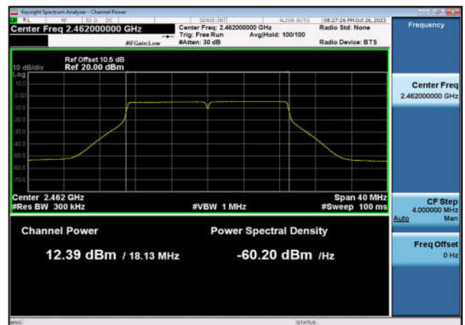
Output Power-802.11n(HT20),2462MHz ,Ant6
