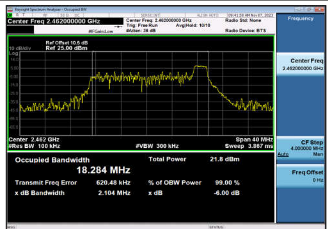
6dB Bandwidth-802.11ax(HE20_RU26 _9),2462MHz,Ant6
