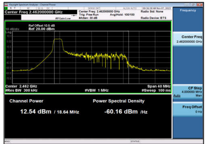
Output Power-802.11ax(HE20_RU26_1),2462MHz,Ant6
