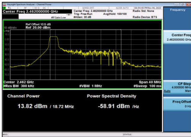
Output Power-802.11ax(HE20_RU26_1),2462MHz,Ant7
