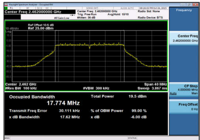
6dB Bandwidth-802.11n(HT20),2462MHz ,Ant6
