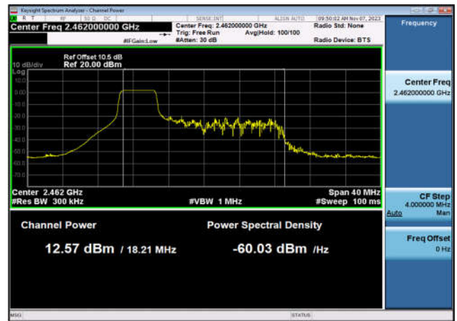
Output Power-802.11ax(HE20_RU52_1),2462MHz,Ant6
