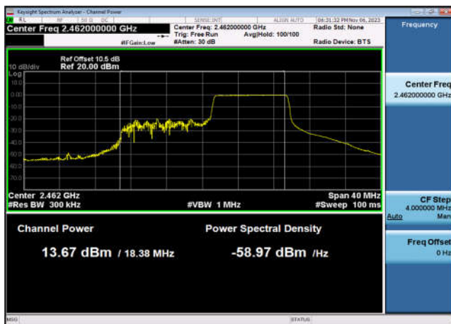
Output Power-802.11ax(HE20_RU106_2),2462MHz,Ant7
