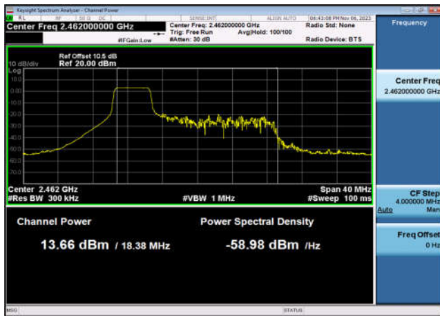
Output Power-802.11ax(HE20_RU52_1),2462MHz,Ant7
