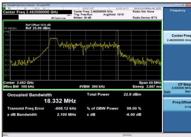
6dB Bandwidth-802.11ax(HE20_RU26_1),2462MHz,Ant7
