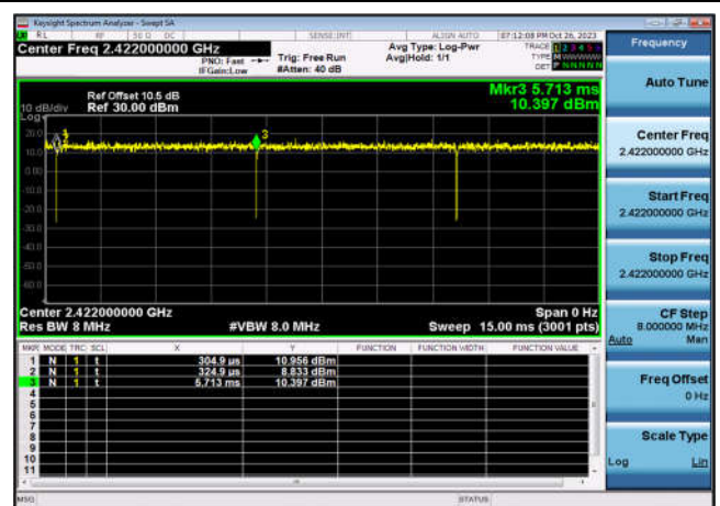
DutyCycle-802.11ax(HE40),2422MHz ,Ant7
