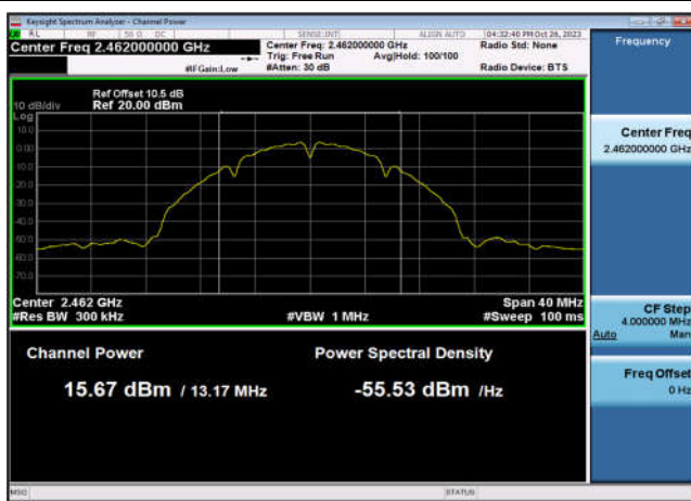
Output Power-802.11b,2462MHz,Ant7
