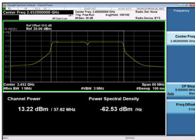
Output Power-802.11n(HT40),2452MHz ,Ant7
