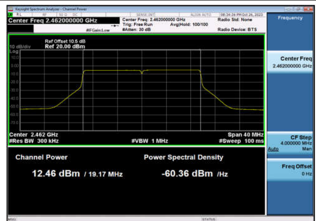
Output Power-802.11ax(HE20),2462MHz ,Ant6
