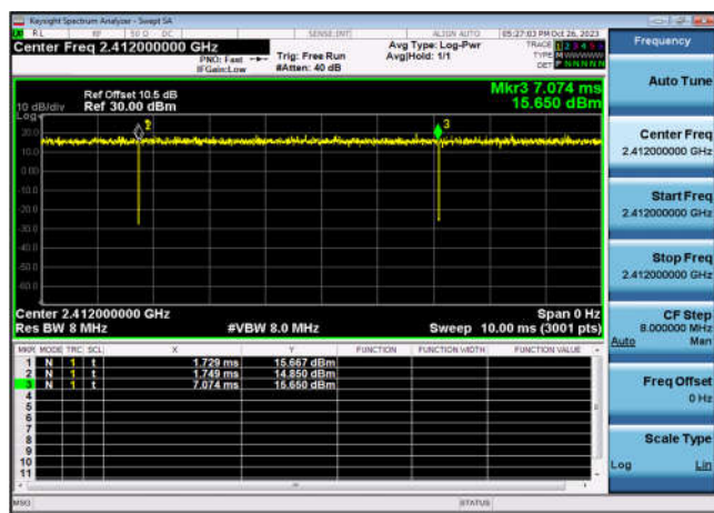
DutyCycle-802.11ax(HE20),2412MHz ,Ant7
