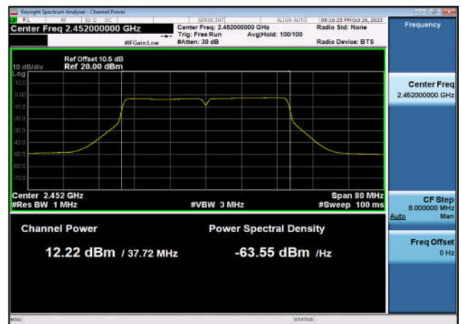
Output Power-802.11n(HT40),2452MHz ,Ant6
