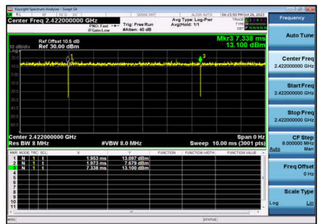
DutyCycle-802.11ax(HE40),2422MHz ,Ant7
