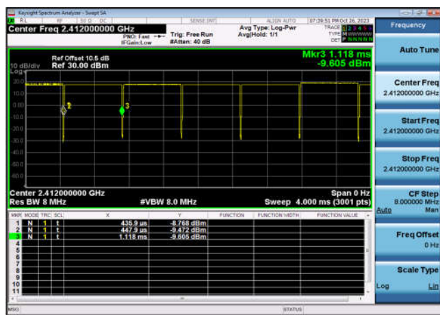
DutyCycle-802.11n(HT20),2412MHz ,Ant7
