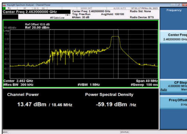
Output Power-802.11ax(HE20_RU26_9),2462MHz,Ant7
