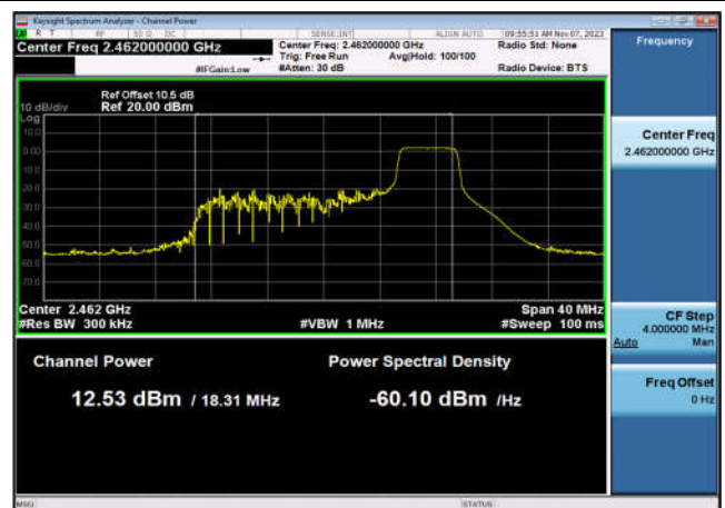
Output Power-802.11ax(HE20_RU52_4),2462MHz,Ant6
