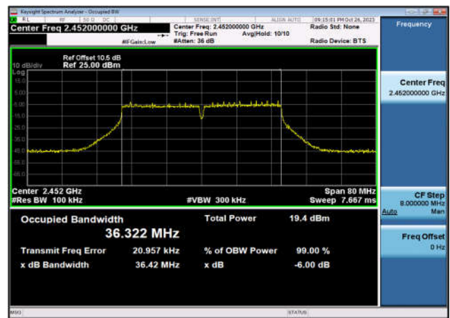
6dB Bandwidth-802.11n(HT40),2452MHz ,Ant6
