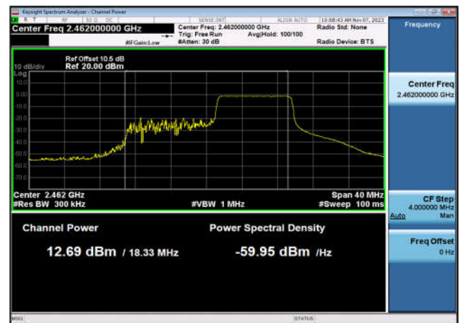
Output Power-802.11ax(HE20_RU106_2),2462MHz,Ant6
