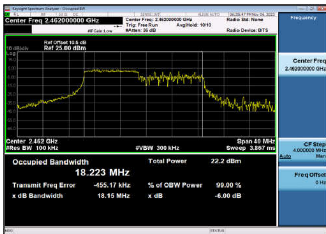
6dB Bandwidth-802.11ax(HE20_RU106 _1),2462MHz,Ant7
