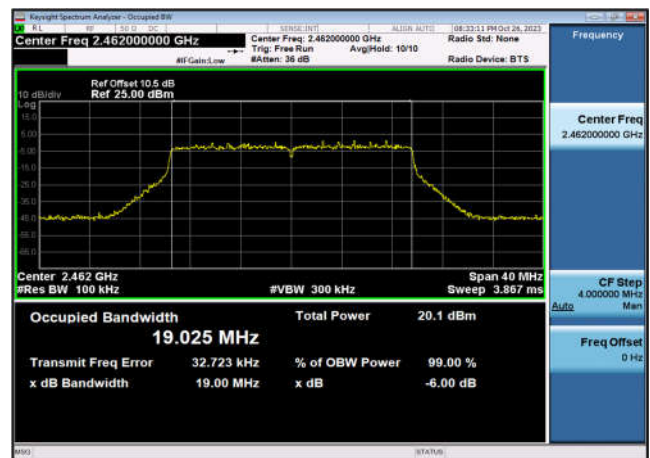
6dB Bandwidth-802.11ax(HE20),2462MHz ,Ant6
