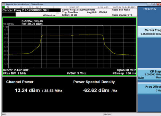
Output Power-802.11ax(HE40),2452MHz ,Ant7
