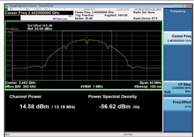
Output Power-802.11b,2462MHz,Ant6
