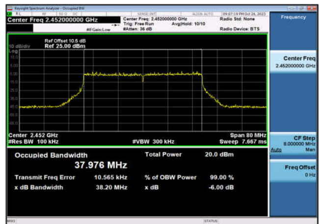
6dB Bandwidth-802.11ax(HE40),2452MHz ,Ant6
