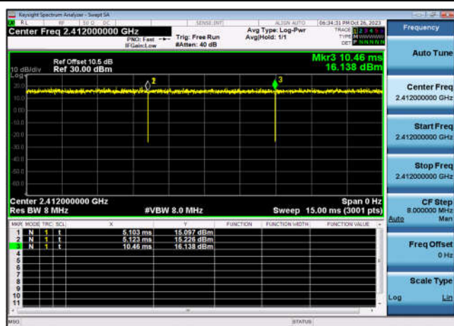
DutyCycle-802.11ax(HE20),2412MHz ,Ant7
