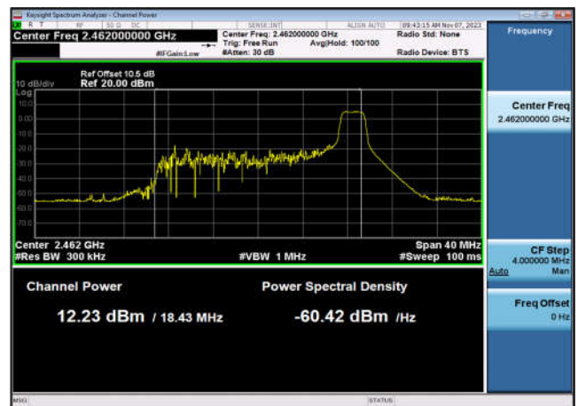
Output Power-802.11ax(HE20_RU26_9),2462MHz,Ant6
