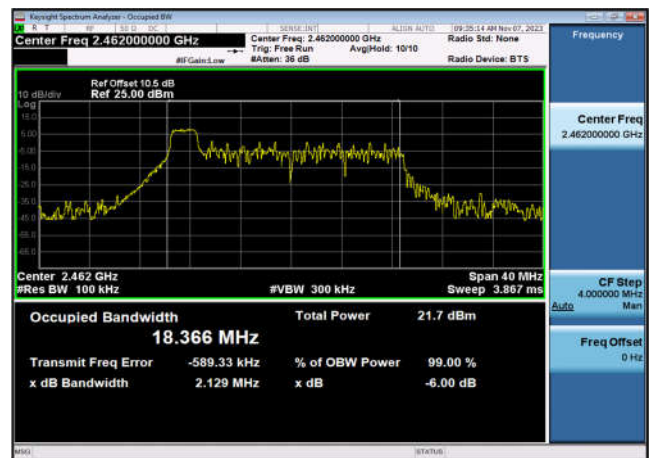
6dB Bandwidth-802.11ax(HE20_RU26_1),2462MHz,Ant6
