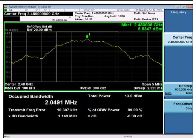
6dB Bandwidth: 2480MHz – 2Mbps
