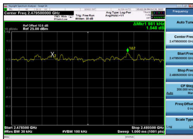
DQPSK,Hopping2DH5,2478.5~2480.5
