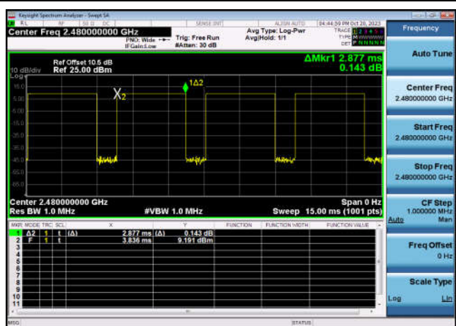
GFSK,2480,DH5,Transmission Time
