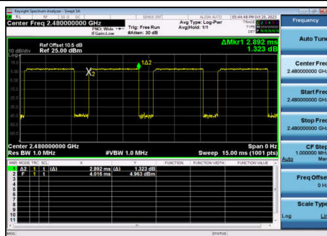
8DPSK,2480,3DH5,Transmission Time
